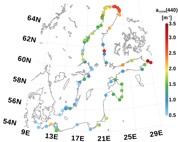
Figure 4. Mean a_{CDOM} of the individual rivers used in the model. The map was created using the software package GrADS 2.1.1.b0 ( http://cola.gmu.edu/grads/ ), using published bathymetry data (Seifert et al., 2008).
