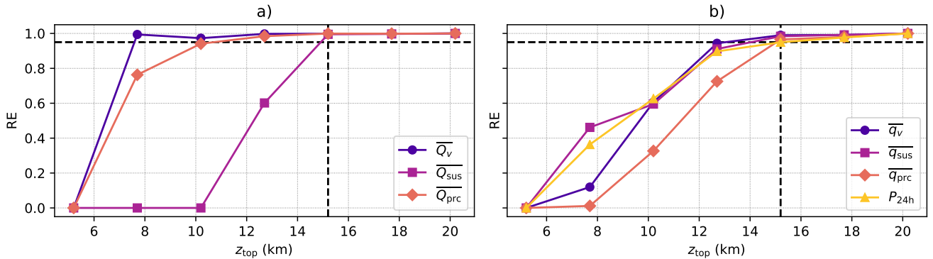
Figure 12. The reduction of error RE of the simulations for the South Island of New Zealand for (a) the total mass of the MP species in the domain and (b) the distribution of the MP species and precipitation in dependence of the model top elevation z_{\text{top}} . ICAR-N imposes a ZG BC on the potential temperature field and constant gradient BCs on the microphysics species (011). The dashed horizontal line indicates the 95 % RE threshold used to determine Z_{\min} and the dashed vertical line shows at which model top this threshold is exceeded for all quantities.
