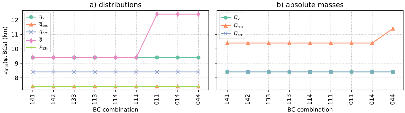
Figure 5. The panels show the minimum model top elevation z_{\min}(\psi, BCs) necessary to reduce the error by 95% for (a) water vapor \bar{q}_v , suspended hydrometeors \bar{q}_{sus} , precipitating hydrometeors \bar{q}_{prc} , potential temperature \bar{\theta} and the 12-hour precipitation sum P_{12h} and (b) the total mass of water vapor \bar{Q}_v , suspended hydrometeors \bar{Q}_{sus} and precipitating hydrometeors \bar{Q}_{prc} , respectively in dependence of the set of upper boundary conditions. The ICAR-N simulations are run for the default scenario.
