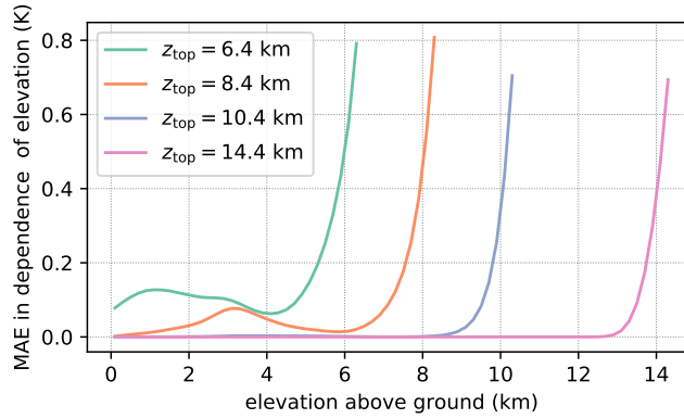
Figure 4. The mean absolute error (MAE) of potential temperature in ICAR-N simulations employing ZG BCs (000) with different model top settings z_{\text{top}} in dependence of the elevation above ground ( x -axis). The MAE is calculated with respect to a reference simulation with z_{\text{top}} = 20.4 km and ZG BCs (000). All simulations are conducted for the default scenario.
