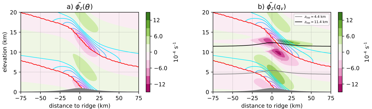
Figure 3. The normalized vertical flux gradient of (a) potential temperature and (b) water vapor (see text for further description). The values are calculated from an ICAR-N simulation at t = 30 \text{ h} with z_{\text{top}} = 20.4 \text{ km} and ZG BCs (000) for the default scenario. The contour lines indicate the vertical convergence ( dw/dz < 0 \text{ s}^{-1} ) in regions where w < 0 \text{ m s}^{-1} . Here the violet contour lines represent stronger and the teal contour lines weaker vertical convergence in the range between -4.5 \cdot 10^{-4} \text{ s}^{-1} and 0 \text{ s}^{-1} spaced in increments of 0.9 \cdot 10^{-4} \text{ s}^{-1} . The red contour line indicates where w = 0 \text{ m s}^{-1} . In panel (b) grey and black lines additionally indicate the location of the model top for z_{\text{top}} = 4.4 \text{ km} and z_{\text{top}} = 11.4 \text{ km} , respectively.
