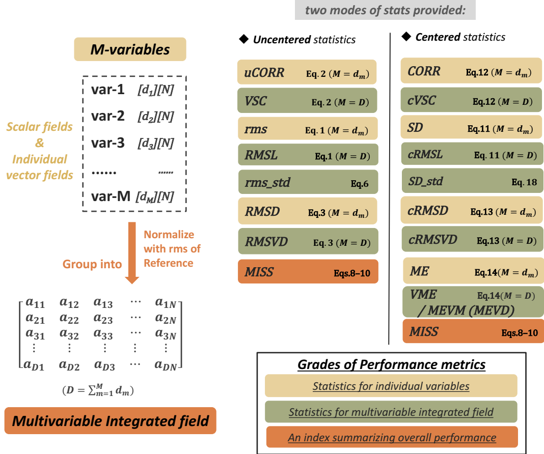
Figure 1. General idea and performance metrics of the improved MVIE. The left-hand column illustrates the general idea of the MVIE. Two modes of statistics are provided for evaluation: uncentered statistics (middle column) and centered statistics (right-hand column). In each mode, the statistics are sorted into three grades: statistics for individual variables, statistics for the multiple field, and a summary index. The right-hand side of the statistics box is its formula.
