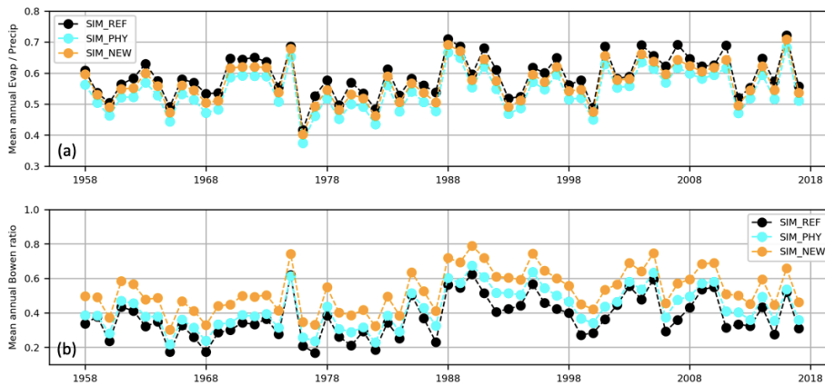
895 Figure 13: Mean annual evaporation to precipitation ratio (a), and Bowen ratio (b), for experiments SIM_REF, SIM_PHY, and SIM_NEW.
