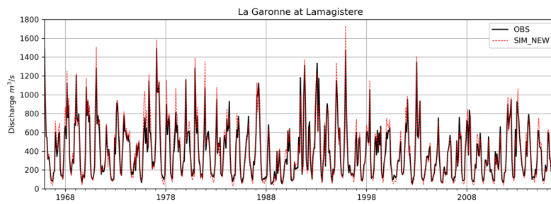
885 Figure 10: Comparison of monthly river flows with SIM_NEW for the Garonne at Lamagistère over the period 1958-2018.
