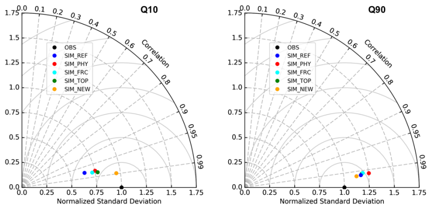
Figure 9: Taylor diagram of Q10 and Q90 deciles of river flows over the period 1958-2018.
