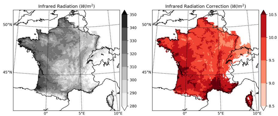
Figure 2: Annual average of uncorrected (left) and corrected (right) downward longwave infrared radiation from SAFRAN analysis.
