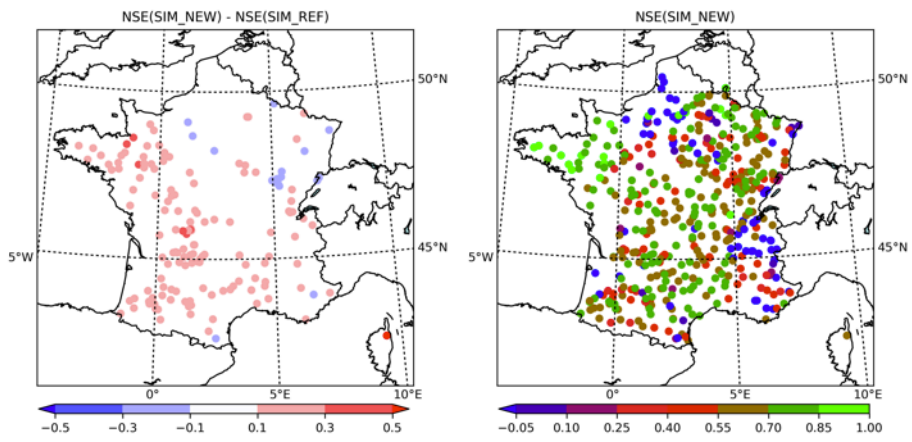
Figure 7: Map of the difference in mean NSE for NSE > 0 between SIM_NEW and SIM_REF (left panel), and SIM_NEW NSE map (right panel).
