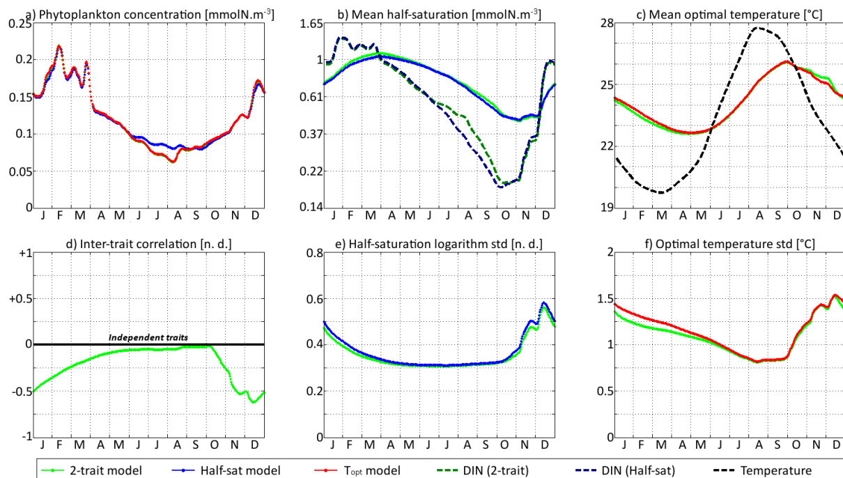
Figure 9. SPEAD state variables at surface for \nu_x = 0.001 (standard) compared with the state variables of 1-trait models: a) total phytoplankton concentration, b) (geometric) mean half-saturation, c) mean optimal temperature, d) inter-trait correlation, e) half-saturation logarithm standard deviation and f) optimal temperature standard deviation. The dashed lines represent the environmental drivers.
