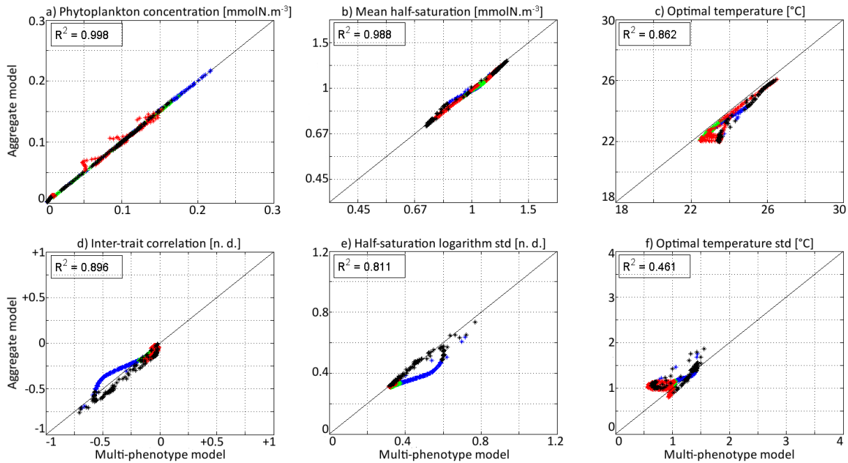
Figure 6. Comparison at all depths and time of the aggregate and multi-phenotype model state variables for \nu_x = 0.001 : a) total phytoplankton concentration, b) (geometric) mean half-saturation, c) mean optimal temperature, d) inter-trait correlation, e) half-saturation logarithm standard deviation and f) optimal temperature standard deviation. Blue is Winter, green is Spring, red is Summer and black is Autumn.
