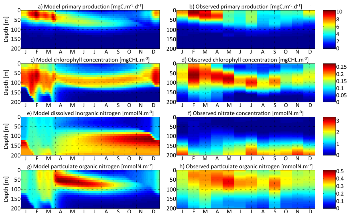
Figure 4. Distribution in depth and time of a) model primary production, c) chlorophyll concentration, e) dissolved inorganic nitrogen concentration and g) particulate organic nitrogen concentration. Each variable is compared with equivalent observations in the Sargasso Sea (b, d, f and h).
