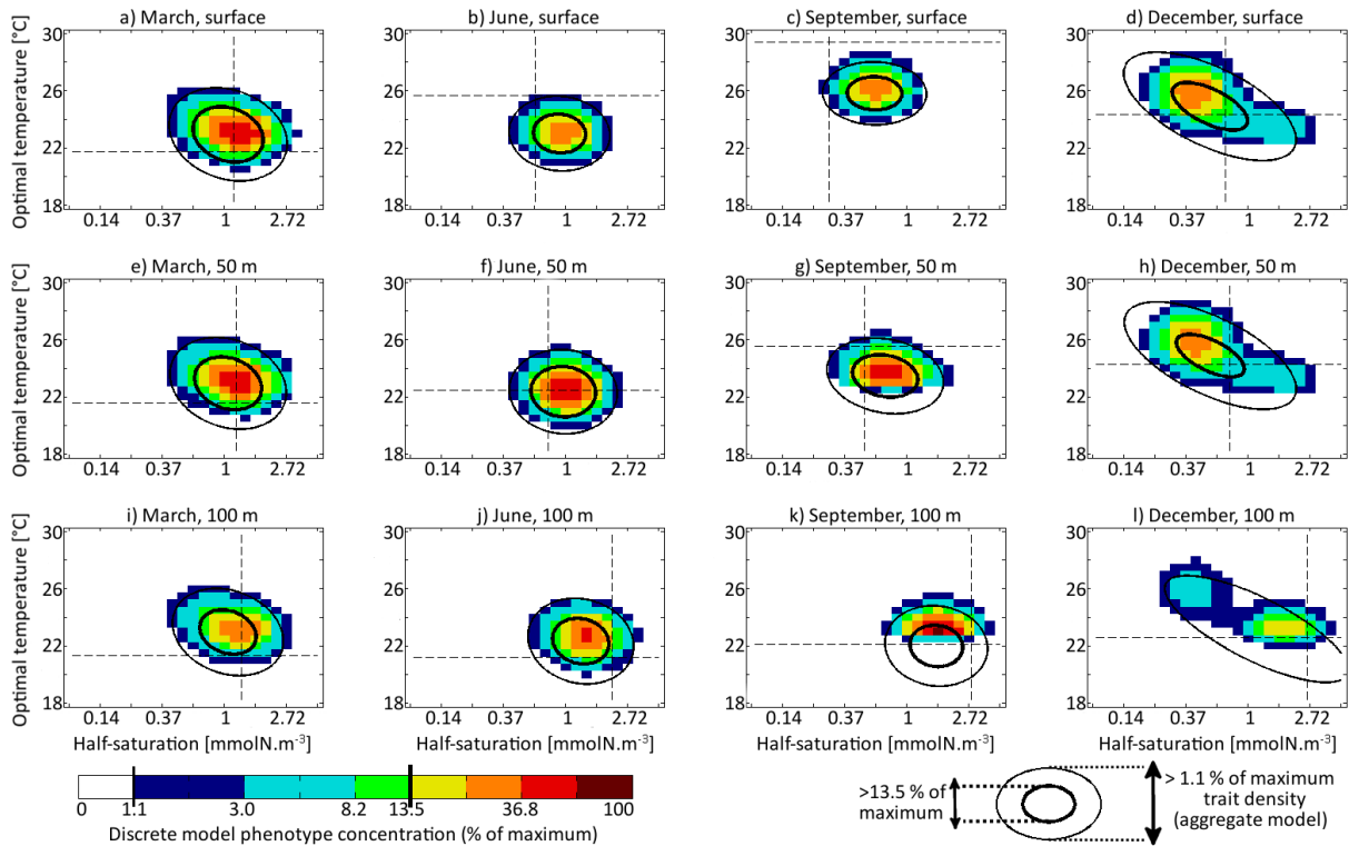
Figure 7. Concentrations of each phenotype of the multi-phenotype model (color) compared with lines of equal density of the aggregate model. Subplots correspond to days 71, 161, 251 and 341, and depths of 0, 50 and 100 m. Dashed lines indicate the optimal competitor.
