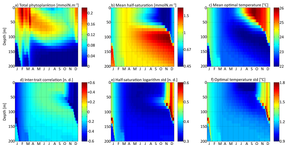
Figure 5. Distribution in depth and time of trait distribution moments for \nu_x = 0.001 : a) phytoplankton concentration, b) (geometric) mean half-saturation, c) optimal temperature, d) inter-trait correlation, e) half-saturation logarithm standard deviation and f) optimal temperature standard deviation. For readability, the mean value of trait x is transformed into a nitrogen concentration in b). To speak properly and contrary to other means present in this study, the "mean half-saturation" is a geometric mean, not an arithmetic mean.
