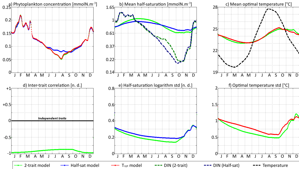
Figure 10. SPEAD state variables at surface for \nu_x = 0.00001 (low mutation rate) compared with the state variables of 1-trait models: a) total phytoplankton concentration, b) (geometric) mean half-saturation, c) mean optimal temperature, d) inter-trait correlation, e) half-saturation logarithm standard deviation and f) optimal temperature standard deviation. The dashed lines represent the environmental drivers.
