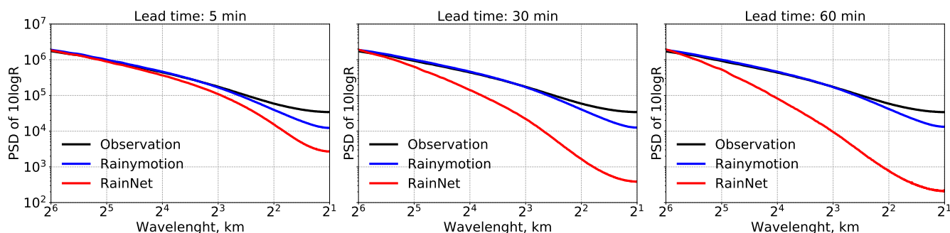
Figure 5. PSD averaged over all verification events and nowcasts, for lead times of 5, 30, and 60 minutes.
