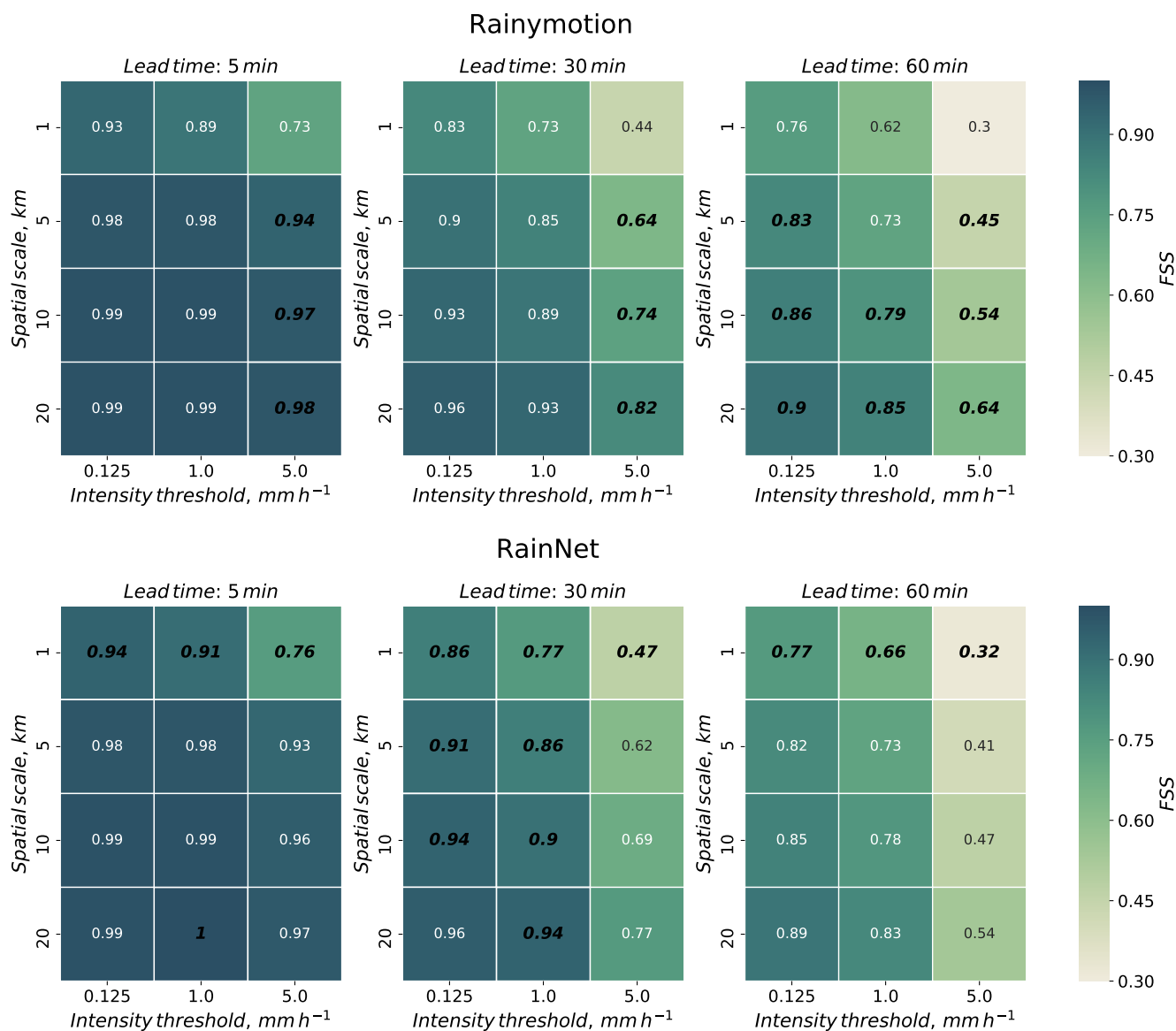
Figure 6. Fractions Skill Score (FSS) for Rainymotion ( top panel ) and RainNet ( bottom panel ), for 5, 30, and 60 minutes lead time, and spatial window sizes of 1, 5, 10 and 20 km, and for intensity thresholds of 0.125, 1, and 5 \text{mm h}^{-1} . In addition to the color code of the FSS, we added the numerical FSS values. The FSS value of the model which is significantly superior for a specific combination of window size, intensity threshold, and lead time is typed in bold black digits, for the inferior model in regular.
