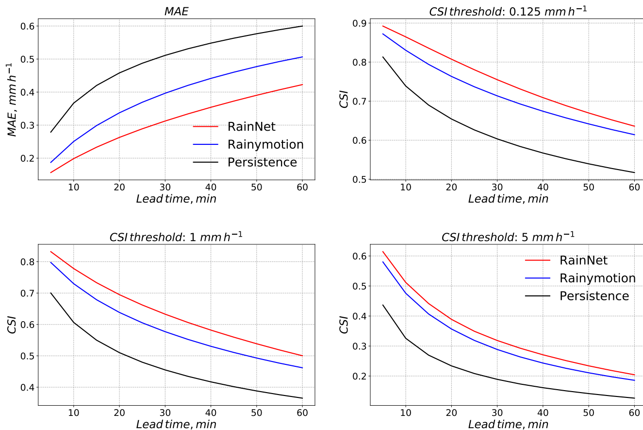
Figure 3. Mean Absolute Error (MAE) and Critical Success Index (CSI) for three different intensity thresholds ( 0.125 \text{ mm h}^{-1} , 1 \text{ mm h}^{-1} , 5 \text{ mm h}^{-1} ). The metrics are shown as a function of lead time. All values represent the average of the corresponding metric over all 11 verification events.
