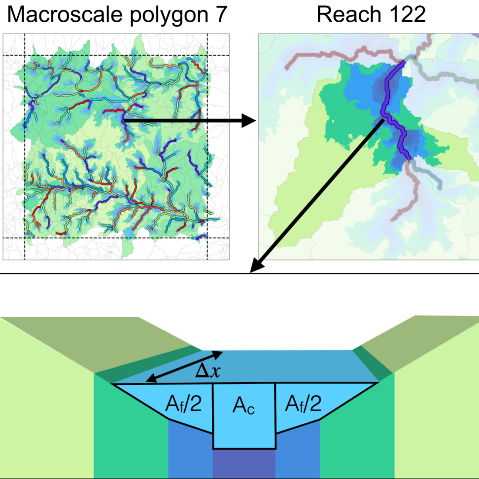
740 Figure 3. The illustration of a river reach in the domain. Using the HAND values, the river reaches are split into a channel (dark blue) and floodplain component (higher blue and greens), where the floodplain component is a combination of the floodplains and hillslopes. Note that a few height bands are omitted in the diagram for simplicity. Similar profiles are assembled for each reach in each macroscale polygon.
