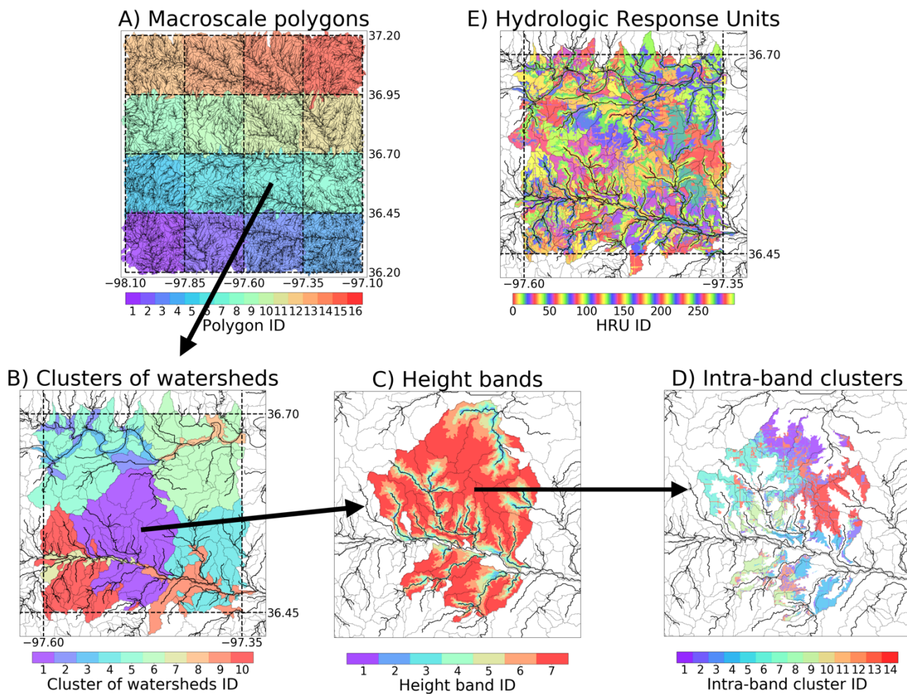
725 Figure 2. (A) The domain is split into 16 macroscale polygons, where each color identifies a polygon. (B) Each macroscale polygon is partitioned into 10 clusters of watersheds via K-means clustering. (C) The HAND data is used to discretize each cluster of watersheds from channel to ridge; this discretization allows to assemble the channel and non-channel height bands. Finally, (D) each of the height bands is split into intra-band clusters (D) . The C and D methods are applied to all clusters of watersheds in B to assemble the final HRU map (E) .
