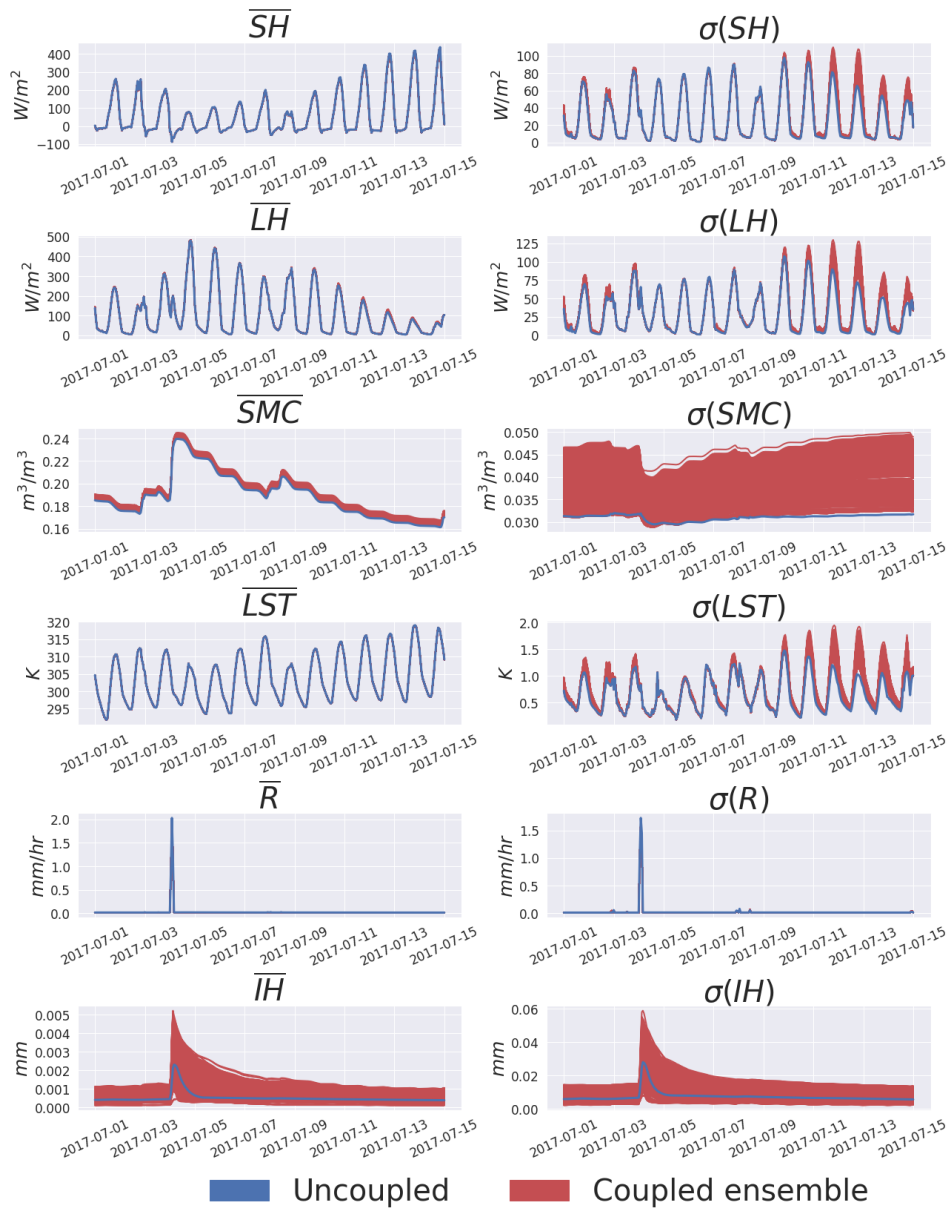
825 Fig 11. Ensemble spread from the Sobolj sensitivity analysis of the coupled routing/land surface HydroBlocks model between July 1 st , 2017 and July 15 th , 2017. The shown simulated variables include the spatial mean ( \bar{X} ) and spatial standard deviation ( \sigma(X) ) of sensible heat flux ( SH ), latent heat flux ( LH ), root zone soil moisture ( SMC ), land surface temperature ( LST ), runoff ( R ), and inundation height ( IH ). For comparison, the baseline uncoupled simulation is shown in blue.
