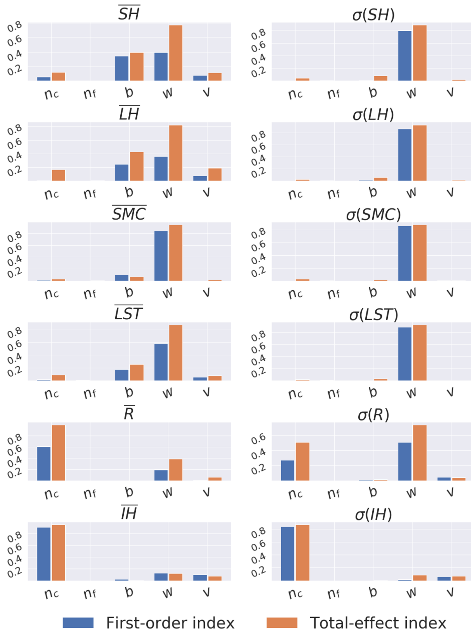
830 Fig 12. First-order ( S_i ) and total-effect sensitivity ( S_{Ti} ) indices from the Sobolj Sensitivity analysis of the n_c (channel manning roughness coefficient), n_f (floodplain manning roughness coefficient), b (channel bankfull depth), w (channel width), and v (uniform overland flow velocity) parameters in the HydroBlocks land surface model over the SGP site in Oklahoma. The explored simulated variables are the same as those in Figure 11.
