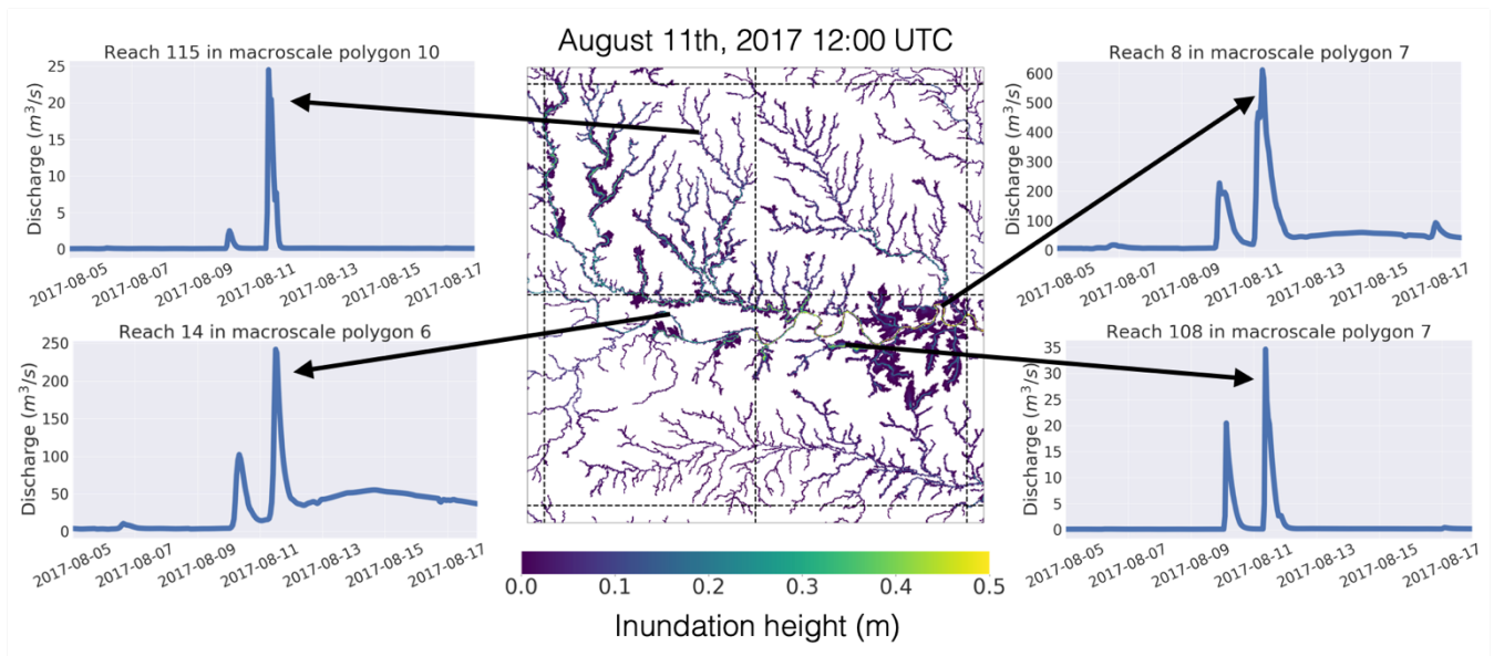
765 Figure 5. The center panel shows the simulated inundated height over the four central macroscale polygons in the study domain on August 11 th , 2017 at 12:00 UTC. The remaining four plots show the simulated discharge at four different reaches between August 5 th and August 17 th . The arrows point to the time step on each time series that correspond to the mapped inundation height. Note that mapped inundation height is upscaled to a 100-meter spatial resolution for visual clarity.
