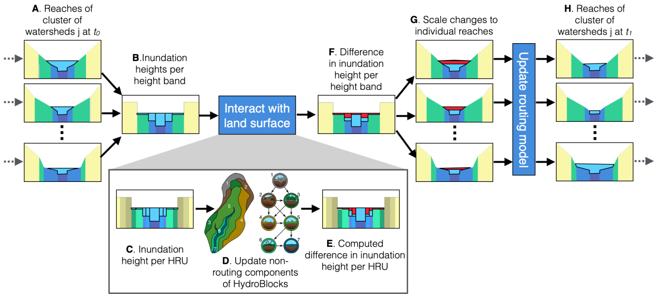
750 Figure 4. Floodplain inundation scheme implemented in HydroBlocks. After the routing module is updated, for a given time step 755 (A), each reach's computed cross-section profile is used to determine the inundation height over each of the height bands in a given reach. The inundation heights per height band are averaged across all watersheds in a given cluster of watersheds (B). These inundation heights are then equally distributed to their corresponding HRUs (C). To update the land surface model component, the computed inundation heights are added to the following time step's as a constant flux at the soil surface to update the non-routing components of HydroBlocks (D). The difference between the old and new inundation heights are computed (E) and averaged back up to the height band level (F). The differences per height band at the cluster of watersheds level are first scaled to each watershed and then aggregated to compute the change in cross-sectional area (G). This difference is then divided by the routing model time step and added to the routing module's source/sink term S in the next iteration of the routing model (H).
