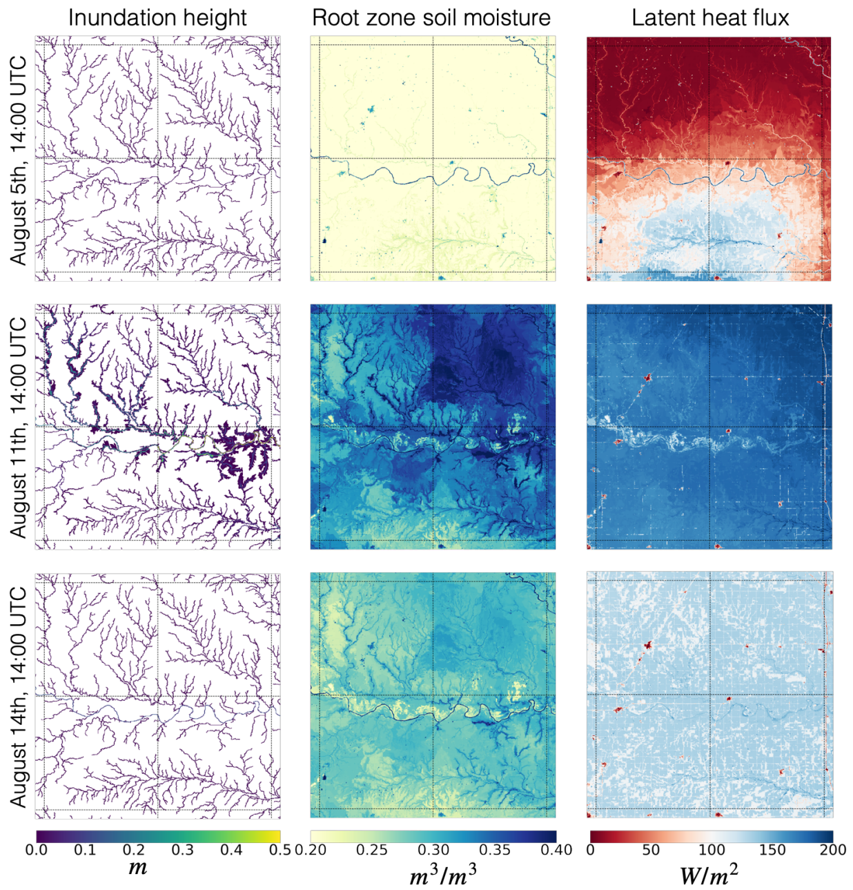
Figure 6. Mapped simulated inundation height, root zone soil moisture, and latent heat flux over the central four macroscale polygons in the study domain on three different time steps: August 5 th 14:00 UTC, August 11 th 14:00 UTC, and August 14 th 14:00 UTC. The chosen time steps coincide with the event shown in Figure 5 and show the area before, during, and after the flood event.
