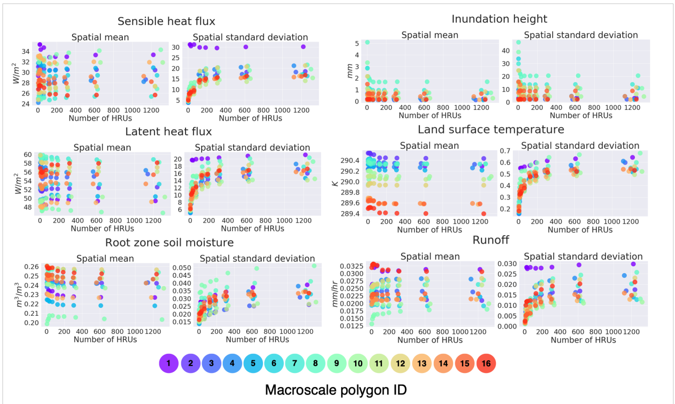
815 Fig 10. Convergence of annual mean of the spatial mean and spatial standard deviation of runoff, land surface temperature, inundation height, root zone soil moisture, latent heat flux, and sensible heat flux for the 9 different HRU configurations. Each color denotes a different macroscale polygon in the 1.0-degree SGP domain.
