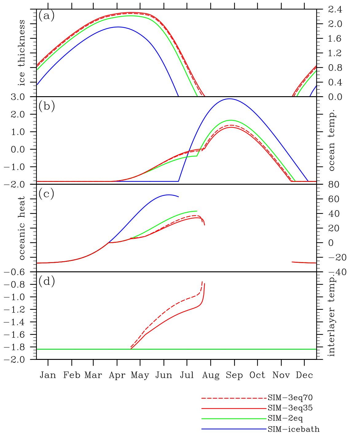
Figure 1. Time series of (a) sea-ice thickness (units: m), (b) ocean temperature (units: ^{\circ}C ), (c) ocean-to-ice heat flux (units: W/m 2 ) and (d) ice-ocean interface temperature (units: ^{\circ}C ) in the experiments SIM-icebath, SIM-2eq, SIM-3eq35 and SIM-3eq70 with friction velocity at 0.002 and ice concentration at 75%. The model is run into equilibrium.
