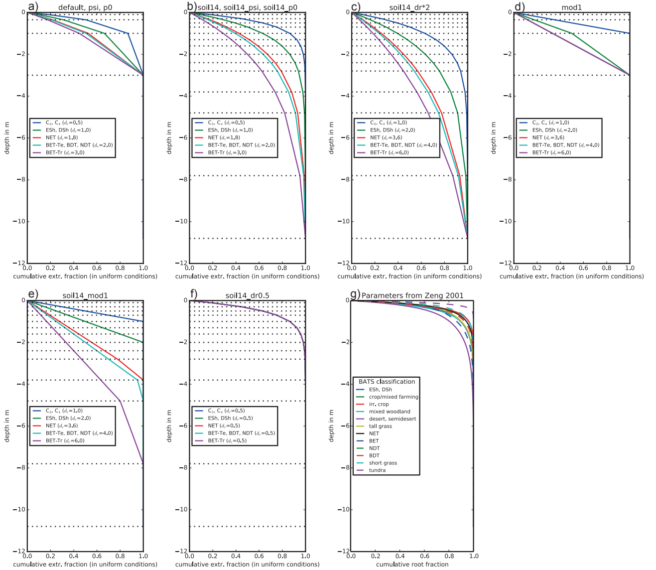
Figure 2: Effective root water extraction profiles for JULES. The parameter d_r is the e-folding depth for weighing root water extraction and soil moisture stress. The Plant Functional Types (PFTs) are: C 3 , C 4 grasses; evergreen and deciduous shrubs (ESh, DSh); needleleaf evergreen trees (NET), temperate broadleaf evergreen trees (BET-Te), broadleaf deciduous trees (BDT), needleleaf deciduous trees (NDT), tropical broadleaf evergreen trees (BET-Tr). The horizontal dotted lines show the bottom depth of each layer. Profiles for the experiments in this study are shown: with the default 3 m deep, four layer soil (a), with an updated 10.8 m deep, 14 layer soil (b), with the 10.8 m deep soil and doubled d_r (c), with water extraction weighted by layer thickness and 3 m deep soils (d), with water extraction
