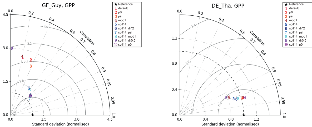
160 Figure 7: Example of impacts of soil moisture stress representations on GPP model skill for two soil moisture stressed sites: GF-Guy (Tropical evergreen forest), and DE-Tha (Temperate evergreen needleleaf forest). The GF-Guy simulations included years 2007-2009; and the DE-Tha simulations included years 1996-2014. Details of the simulations are provided in Sect. 2.3 and Tables 1-2.
