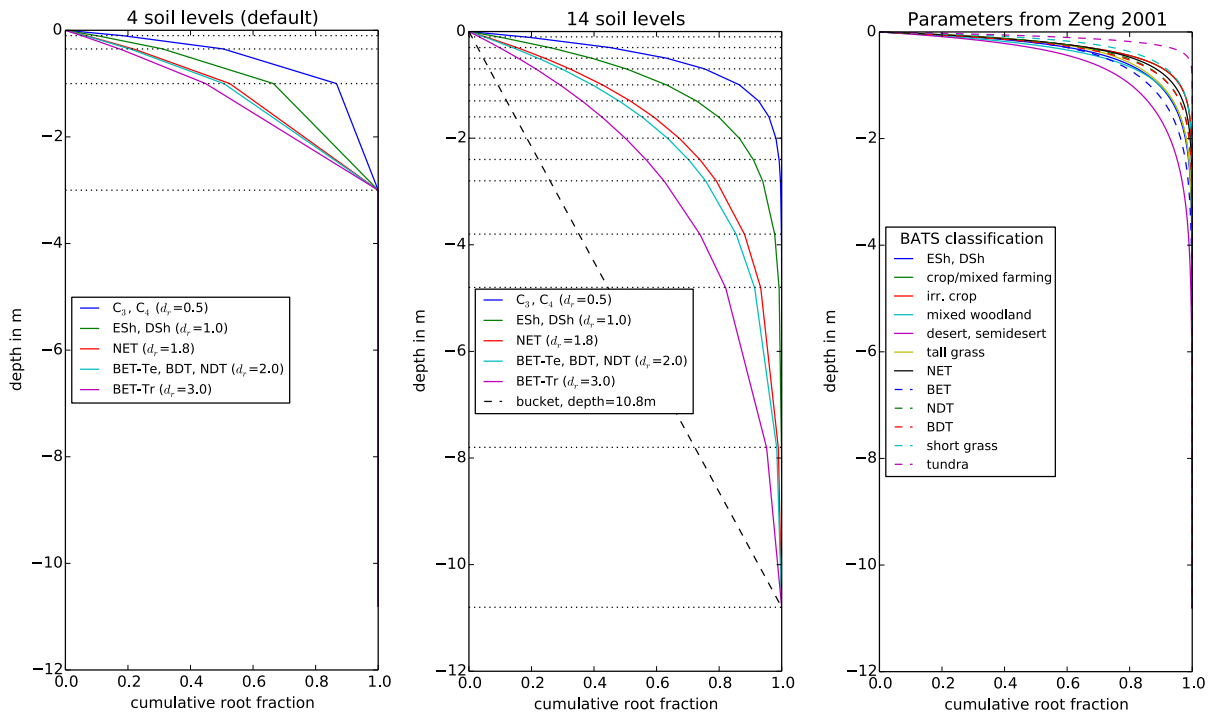
Figure 2: Effective root water extraction profiles for JULES with the default four layer soil (maximum depth of 3 m; left panel), with an updated 14 layer soil (maximum depth of 10.8 m; middle panel), and compared to root fractions from Zeng (2001) (right panel), where distributions were calculated based on available measurements of root profiles. The parameter d_r in JULES is the e-folding depth for weighing root water extraction and soil moisture stress.. The plant functional types are: C_3 , C_4 grasses; evergreen and deciduous shrubs (ESh, DSh); needleleaf evergreen trees (NET), temperate broadleaf evergreen trees (BET-Te), broadleaf deciduous trees (BDT), needleleaf deciduous trees (NDT), tropical broadleaf evergreen trees (BET-Tr).
