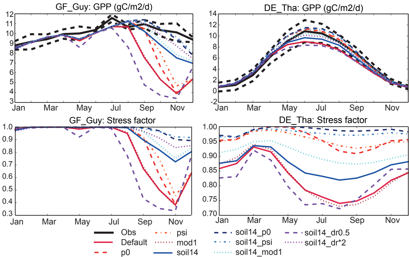
Figure 8: Example of impacts of various soil moisture stress-related changes (see Table 1) on simulated seasonal cycle of GPP at two soil moisture stressed sites (see Section 3.3; similar figures for BE-Vie and CA-Oas are in Fig. SM9a). The GF-Guy simulations included years 2007-2009; and the DE-Tha simulations included years 1996-2014. GF-Guy is a tropical evergreen broadleaf forest and DE-Tha is an evergreen needle-leaf forest. Details of the simulations are provided in Sect. 2.3 and Tables 1-2.
