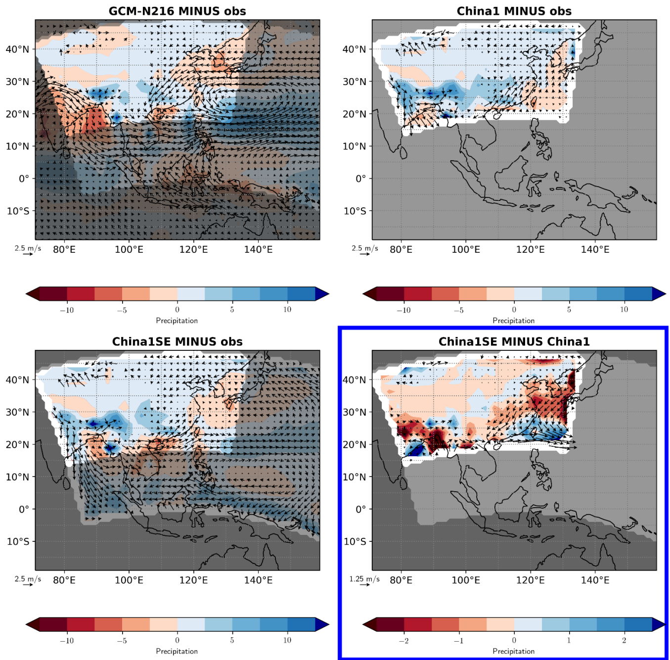
790 Figure 4: (top) JJA climatological (1989-2008) precipitation and 850hPa wind errors in the AGCM-N216 simulation and the China1 RCM simulation vs TRMM and ERA-Interim (obs). (bottom) Effects of extending the domain towards the south and east: (left) China1SE minus obs; (right) China1SE minus China1. Colour bar indicates precipitation differences (mm/day) and vectors indicate differences in 850 hPa winds. NOTE difference in contour intervals and vector scale for lower right panel. Non-shaded area highlights China1 region, lightly shaded area highlights China1SE region, darker shaded area highlights areas not covered by China1 and China1SE domains.
