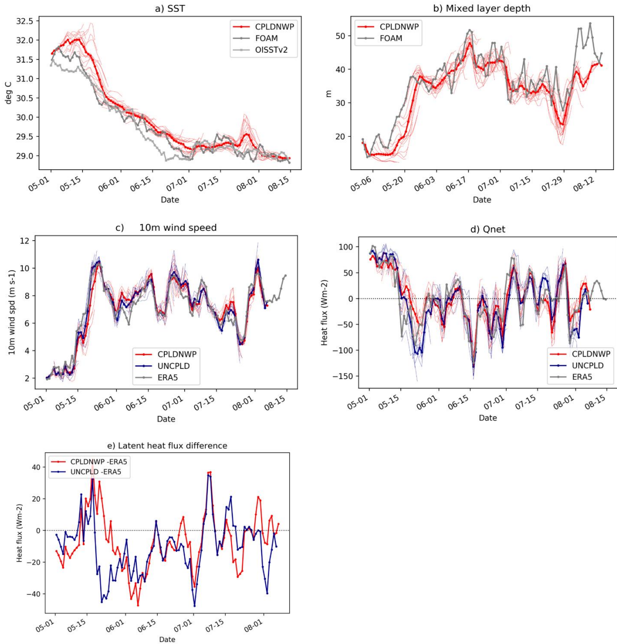
Figure 13: Time series of daily forecasts initialised between 1 May–31 July 2016. Individual forecasts (thin lines) are averaged at each validity time ('Date') into a mean forecast (coloured heavy line). Grey lines are from analyses. Lines show area-averages over EEIO northern box (2°-15°N, 87°-96°E; see Fig. 8e) (a) SST from CPLDNWP and FOAM analyses, out to day 15; (b) mixed layer depth calculated using daily mean temperature and salinity from CPLDNWP and FOAM analyses, out to day 15; (c) 10m wind speed from CPLDNWP (red) and UNCPLDNWP (blue) out to day 7; (d) net surface heat flux from CPLDNWP (red) and UNCPLDNWP (blue) out to day 7. Positive (negative) value denotes net flux into (out of) the ocean; (e) Mean forecast error of latent heat flux in CPLDNWP and UNCPLDNWP forecasts, relative to ERA5.
