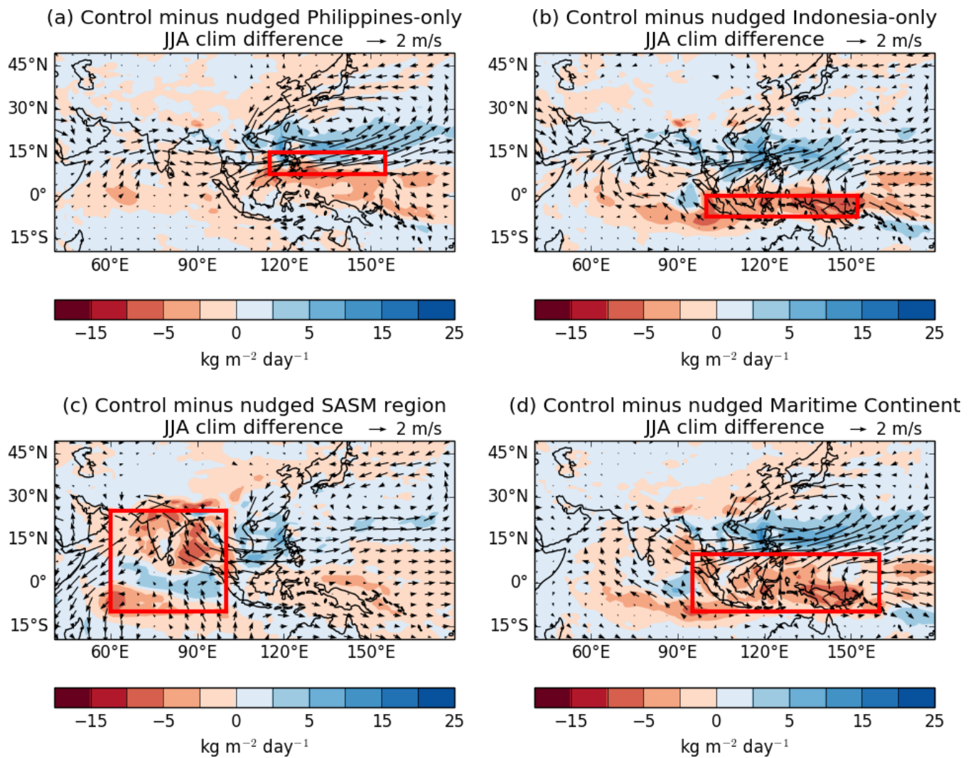
855 Figure 14: Climatological differences in 850 hPa winds and rainfall in JJA between “Nudged” experiments and their Control, indicating the influence on the Control of errors developing in four different regions used for the Nudged experiments: (a) Philippines; (b) Indonesia; (c) South Asian summer monsoon (SASM); (d) Maritime Continent. The nudged regions are shown in red: “Philippines” [115°-155°E, 7.5°-15°N], “Indonesia” [100°-152.5°E, 7.5°S-0°N], “SASM” [60° - 100°E, 10°S - 25°N], and “Maritime Continent” [95° - 160°E, 10°S - 10°N].
