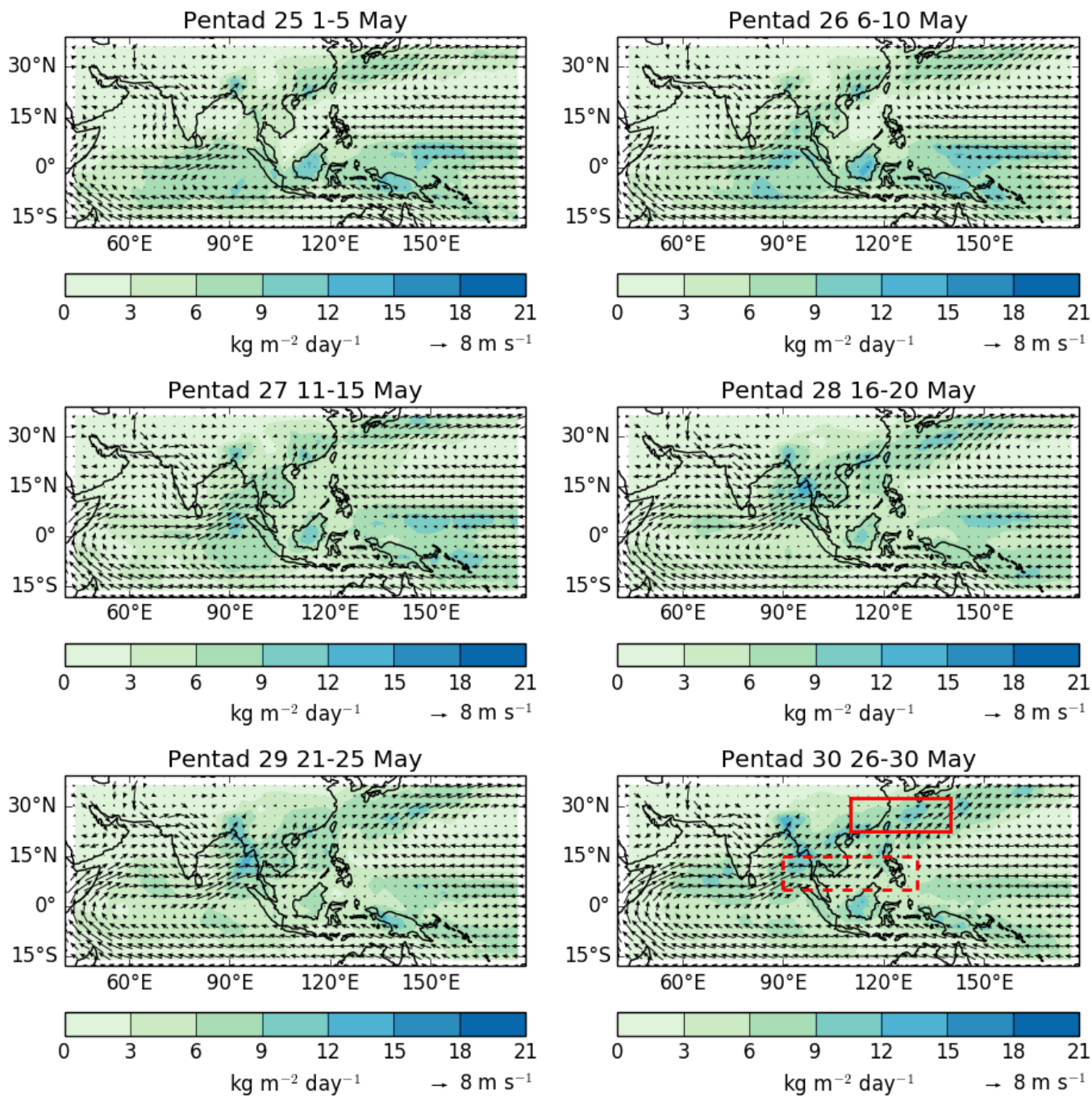
825 Figure 9: Pentad evolution of 850 hPa winds (ERA-Interim) and rainfall (GPCPv2) through the broadscale seasonal transition towards the Asian summer monsoon season, heralded by the reversal of wind direction over the South China Sea which typically occurs around pentad 28 (Wang et al., 2004). The red boxes on the final panel indicate the northern (solid) and southern (dashed) regions that are used in the calculation of the East Asian Summer Monsoon Index (see Wang et al. (2008) and Fig. 8d).
