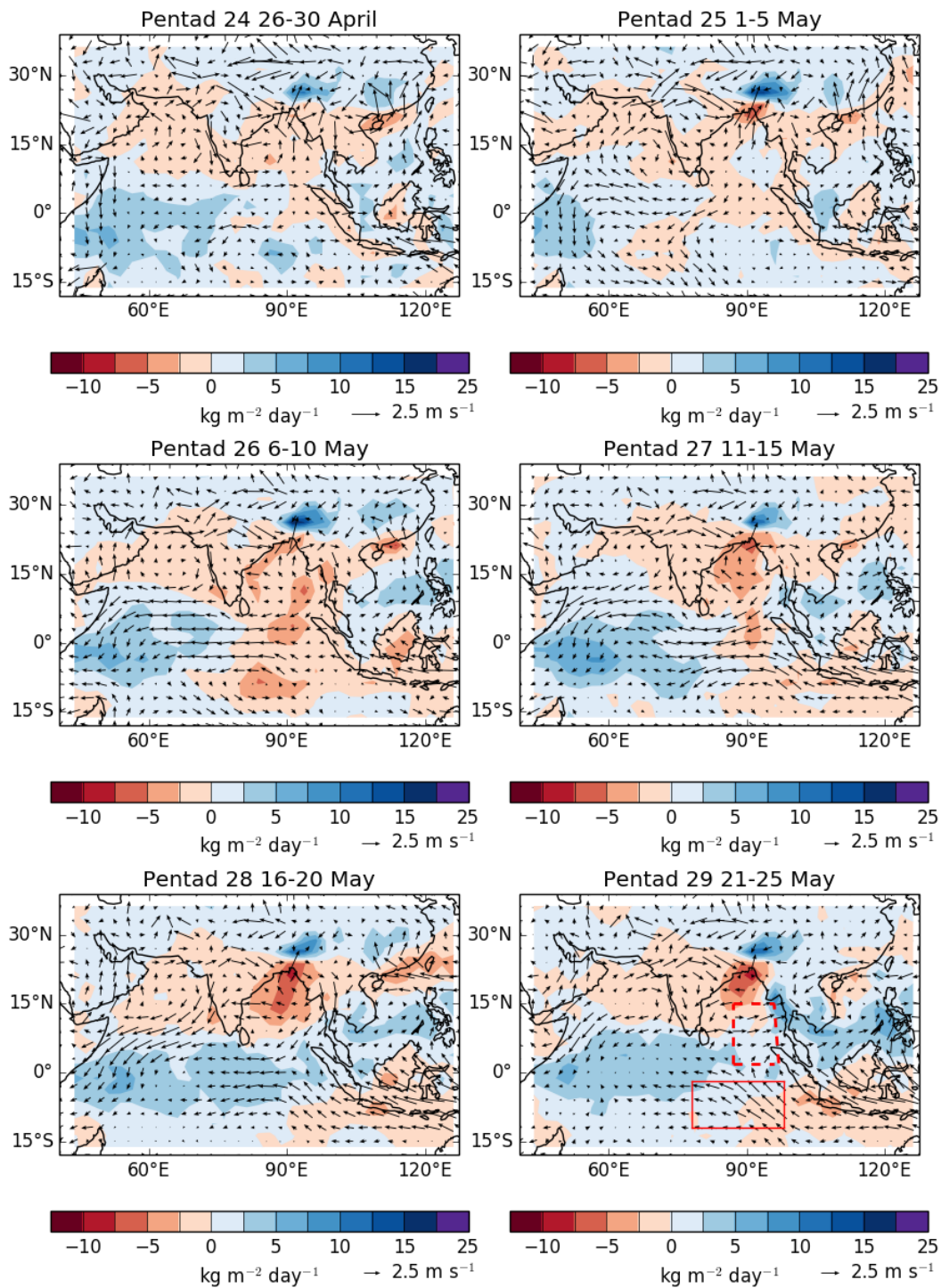
830 Figure 10: Development of climatological errors in 850 hPa winds and precipitation (against ERA-I and GPCPv2), pentad by pentad after initialisation on 25 th April. The red boxes indicate the northern (dashed) and southern (solid) EEIO boxes used in Fig. 8(e, f).
