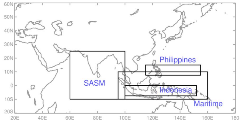
915 Figure 14: Regions used in nudged climate simulations: “Philippines” [115°–155°E, 7.5°–15°N], “Indonesia” [100°–152.5°E, 7.5°S–0°N], “S Asian Monsoon (SASM)” [60°–100°E, 10°S–25°N], and “Maritime Continent” [95°–160°E, 10°S–10°N].
