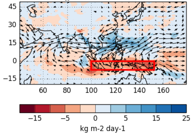
(b) Control minus nudged Indonesia-only JJA clim difference \rightarrow 2 \text{ m/s}
