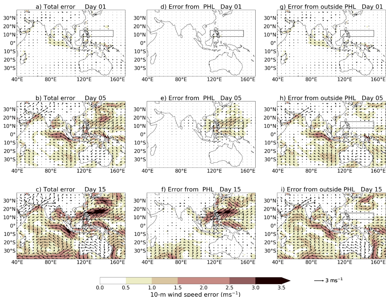
930 Figure 4615: June–August 2016 mean 10m-wind errors (arrows) and their magnitudes ( shading, ms-colours, \text{m s}^{-1} ). (a–c) atmosphere-only NWP- N2162016 total errors, with respect to MetUM analysis, for forecast lead times of 1, 5 and 15 days. (d–f) NWP- N216-free2016 Control run minus Philippines nudging (nudged region shown in Fig. 15a as black box ), showing errors forced from the Philippines for forecast lead times of 1, 5 and 15 days. (g–i) Philippines nudging minus global nudging, showing errors forced outside of the Philippines for forecast lead times of 1, 5 and 15 days.
