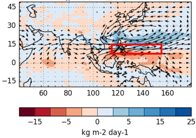
(a) Control minus nudged Philippines-only JJA clim difference \rightarrow 2 \text{ m/s}
