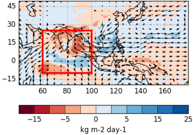
(c) Control minus nudged SASM region JJA clim difference \rightarrow 2 \text{ m/s}
