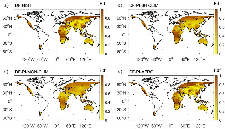
Figure 1. Fdf during 1901-01-01 00:00-06:00 UTC from (a) the original forcing including climate variability from CRU-JRA and historical aerosol concentration ( DF-HIST ), (b) the 6-hour mean of 01-01 00:00-06:00 Fdf over 1901-1920 non-volcanic years ( DF-PI-6H-CLIM ), (c) the monthly mean of January Fdf over 1901-1920 non-volcanic years ( DF-PI-MON-CLIM ), (d) the reconstruction using climate variability from CRU-JRA and mean 1901-1920 aerosol concentration ( DF-PI-AERO ). Night time pixels are masked for comparison.
