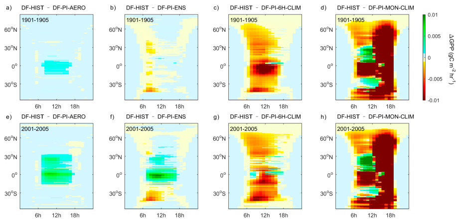
Figure 5. Diurnal variations of \Delta\text{GPP} in \text{gC m}^{-2} \text{hr}^{-1} between DF-HIST and DF-PI-AERO (a,e), DF-PI-ENS (b,f), DF-PI-6H-CLIM (c,g) and DF-PI-MON-CLIM (d,h) during 1901-1905 (a-d) and 2001-2005 (e-h).
