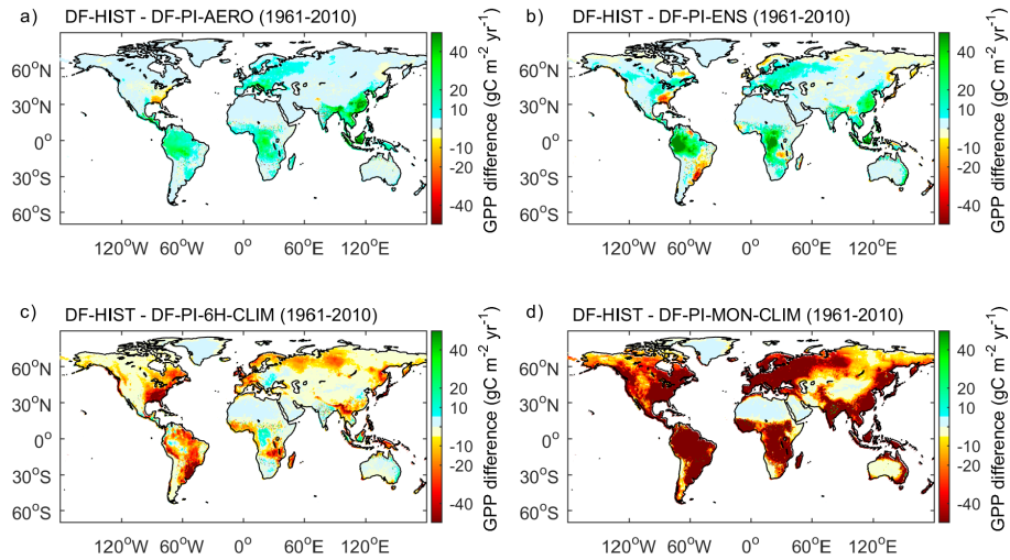
Figure 3. Spatial patterns of \Delta\text{GPP} (in \text{gC m}^{-2} \text{yr}^{-1} ) between DF-HIST and (a) DF-PI-AERO , (b) DF-PI-ENS , (c) DF-PI-6H-CLIM and (d) DF-PI-MON-CLIM during 1961-2010.
