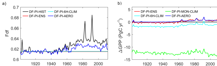
Figure 2. Time series of (a) global mean Fdf and (b) \Delta GPP between DF-HIST and no-anthropogenic-aerosol scenarios. The DF-PI-MON-CLIM has the same mean Fdf as DF-PI-6H-CLIM , thus not shown in (a). The shaded area along the red curve in (b) indicates the range of the three ensemble members of the DF-PI-ENS simulations.
