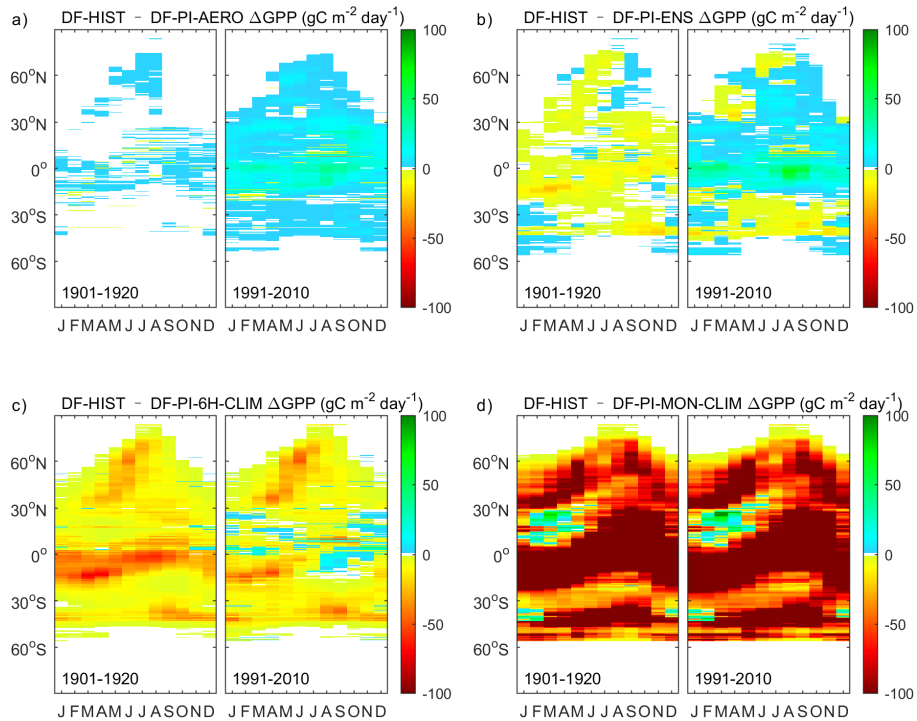
Figure 4. Seasonal variations of \Delta\text{GPP} in \text{gC m}^{-2} \text{day}^{-1} between DF-HIST and (a) DF-PI-AERO , (b) DF-PI-ENS , (c) DF-PI-6H-CLIM and (d) DF-PI-MON-CLIM during 1901-1920 and 1991-2010.
