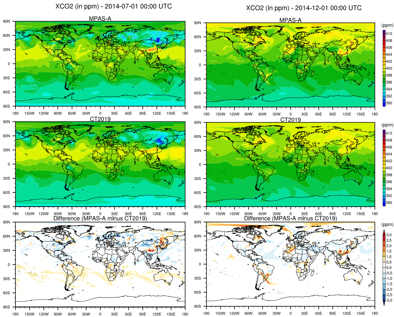
Figure 4. Simulated XCO 2 of MPAS-A, CT2019, and their difference at 2014-07-01 and 2014-12-01 00:00 UTC.
