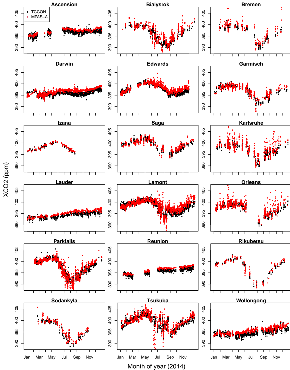
Figure 7. Simulated hourly XCO 2 of MPAS-A at 18 TCCON sites for the year of 2014.
