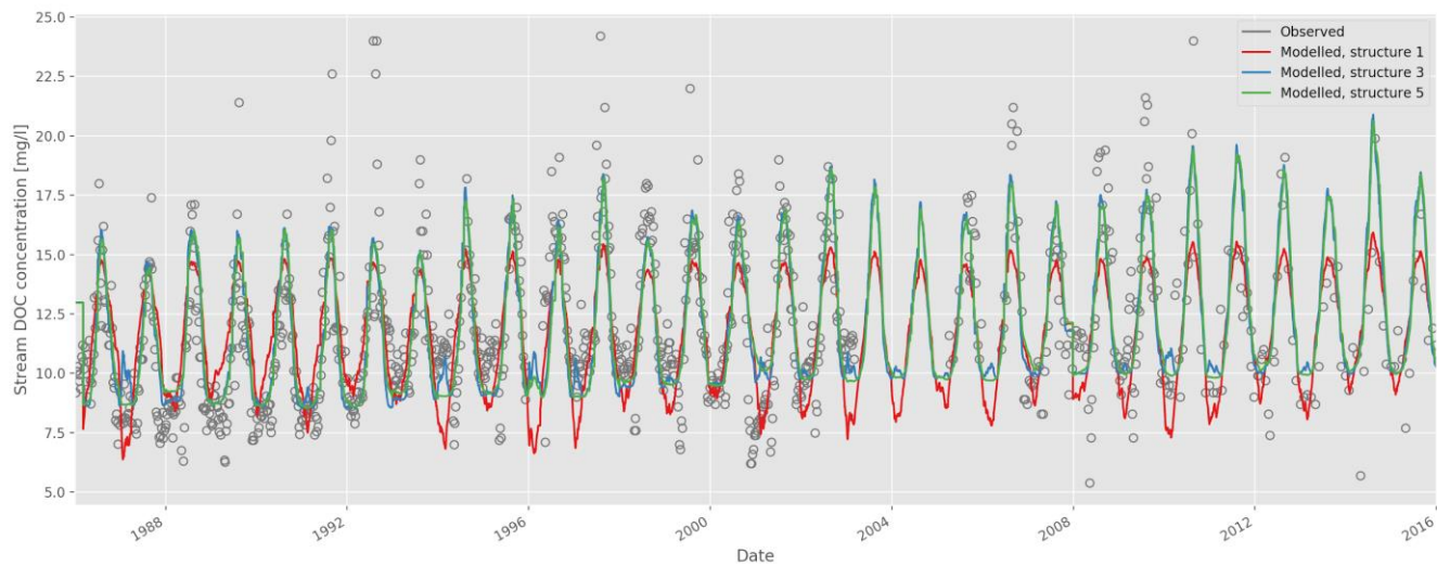
555 Figure 2: Time series of observed and modelled stream dissolved organic carbon (DOC) concentration (model structures 1, 3 and 5; auto-calibrated parameters).
