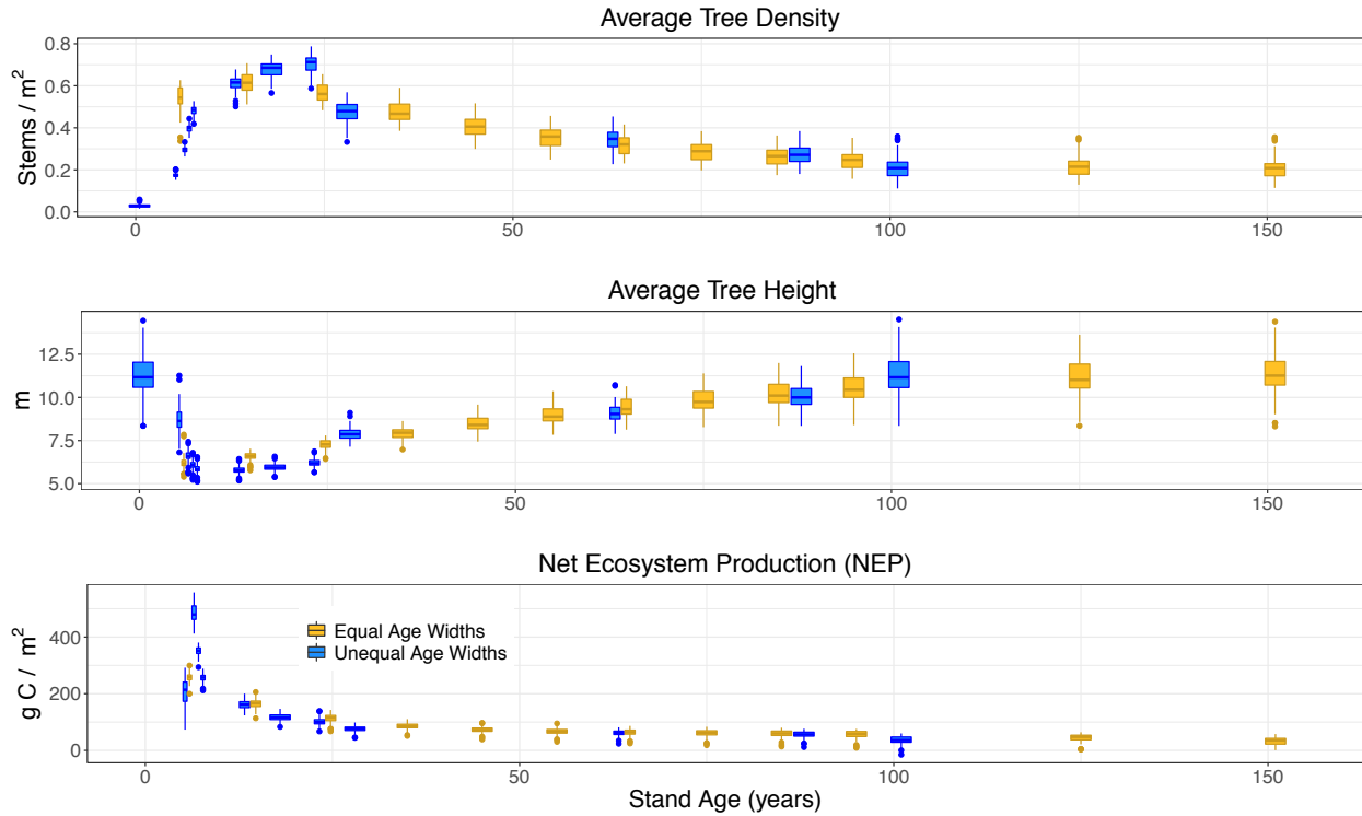
1065 Figure 3. Boxplots by age classes (x-axis, in years ) from LPJ-wsl v2.0 simulations for U.S. States of MI, MN, WI. Data are from (yellow) simulations using equal age widths and (blue) simulations using and unequal age widths (see Table 1). Data are plotted on the x-axis at the middle age of the age class bin; note that the last age class bin for either simulation is defined as +151 yrs (equal bin) and +101 years (unequal bin). For average tree height (middle row), large tree heights in the youngest age class of the unequal bin simulation (blue) represents 1070 so-called ‘survivor’ trees.
