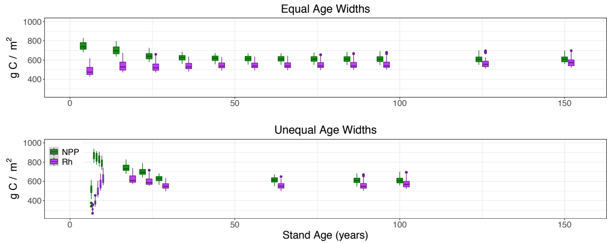
Figure 4. Boxplots of NPP and Rh by age classes (x-axis, in years ) from LPJ-wsl v2.0 simulations for U.S. States MI, MN, WI, for simulations using (top) equal-bin age widths and (bottom) unequal-bin age widths.
