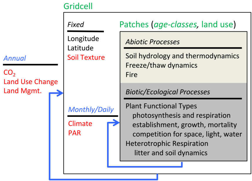
1050 Figure 1. LPJ-wsl v2.0 model structure of inputs (red), time-steps (blue) and the level at which state variables are tracked within grid cells and sub-gridcell age classes (green), such as age classes or land uses. Simulation of abiotic, biotic and ecological processes occurs at the scale of an age class.
