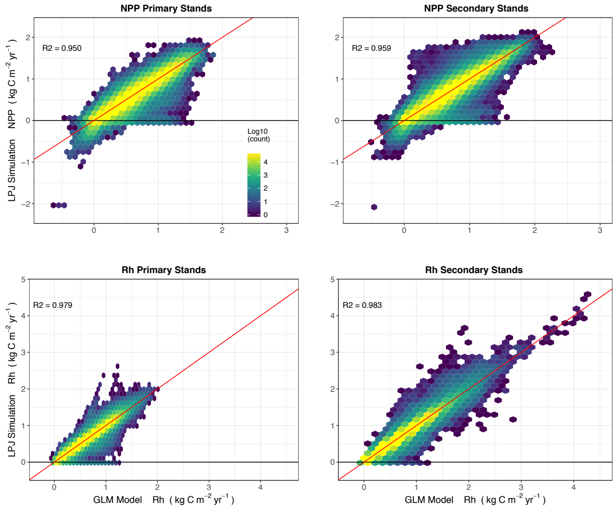
1105 Figure 10. Annual fluxes (NPP, Rh) (2000-2017) from LPJ-wsl v2.0 simulations versus predictions of LPJ-wsl v2.0 fluxes based on a generalized linear model (flux = precipitation + temperature + age-class); coefficients were allowed to vary by grid cell, in essence, reducing the effect of variation in plant composition, soil texture and hydrology. Coloring is by density of grid cells on a log scale; diagonal red line is the 1:1 correspondence line. The simplified statistical model can simplify the dynamics in the global vegetation model, with coefficients from the GLM helping to determine the relative importance of a small set of predictors.
