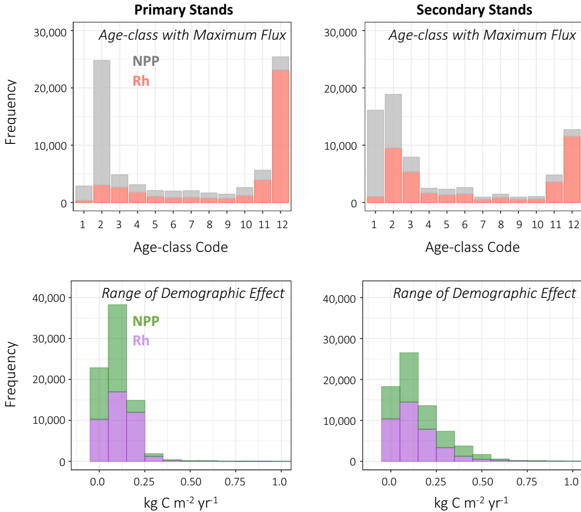
1120 Figure 12. Stacked frequency plots for NPP, Rh on primary and secondary stands. (top row) Global frequency of age classes with the largest flux (NPP, Rh), relative to other age classes in the grid cell. Age-class codes, lowest (youngest) to greatest (oldest), correspond to the 10-yr-equalbin age-class setup (Table 1). (bottom row) Global frequency of the range of the demographic effect on fluxes, bin width is 0.10 \text{ kg C m}^{-2} \text{ yr}^{-1} . An example interpretation, on primary stands, (top left) NPP is greatest in the second age class and (bottom left) the demographic effect on NPP is < 0.25 \text{ kg C m}^{-2} \text{ yr}^{-1} .
