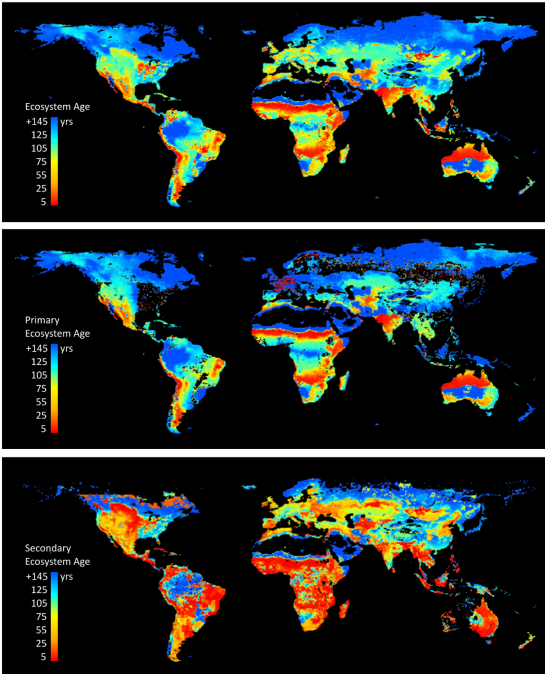
Figure 13. LPJ-wsl v2.0 simulated global distribution of ecosystem ages, defined as the time since disturbance by fire and/or land-use change and land management (LUCLM) in year 2016. (top) Average age of the natural ecosystem, scaled to the area of natural lands within 0.5° grid cells. (middle) Average age of primary Ecosystems only, wherein only fire creates age structure, scaled to the area of primary lands. (bottom) Average age of secondary Ecosystems only, wherein fire and LUCLM creates age structure, scaled to the area of secondary lands.
