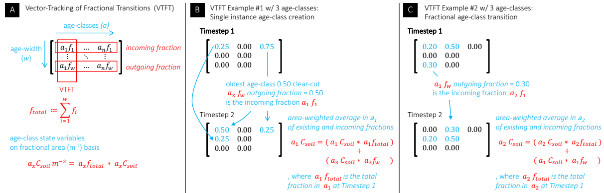
1055 Figure 2. Methodological examples of the matrix based method called Vector-Tracking of Fractional Transitions for computationally-efficient simulation of age classes in large-scale models. (a) Hypothetical matrix of VTFT vectors of fractional areas ( f ). The total area of the age class is the sum of the fractional areas in the corresponding VTFT vector. State variables are calculated on area basis by accounting for the fractional area of the age class, in this example C_{soil} is the carbon in soil. (b) An example of the VTFT method for a newly created age class by clear-cut wood harvest. An area-weighted average updates age-class state variables in the youngest age class using the preceding total fractional area of the age class and the incoming fraction. (c) A VTFT example for a fractional age-class transition. An area-weighted average updates state variables in an age class using the preceding total fractional area of the age class and the incoming fraction from the younger age class. 1060
