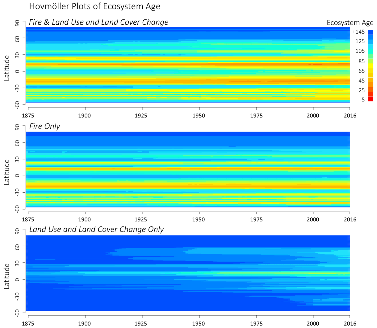
Figure 8. Zonal ecosystem age versus year based on LPJ-wsl v2.0 simulations using full forcing (top), only fire (middle), or only land use and land cover change (bottom).
