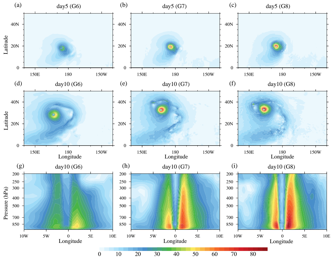
Figure S1. The same as Figure 6 but for the ptend_f1_f1 configuration in GRIST-CAM5phys.
