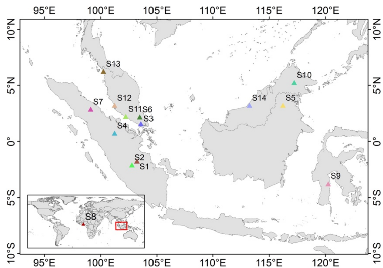
785 Figure 1. Spatial distribution of the 14 observation sites used for model calibration and evaluation. The red rectangle in the inserted map shows the location of main map (Malaysia and Indonesia).
