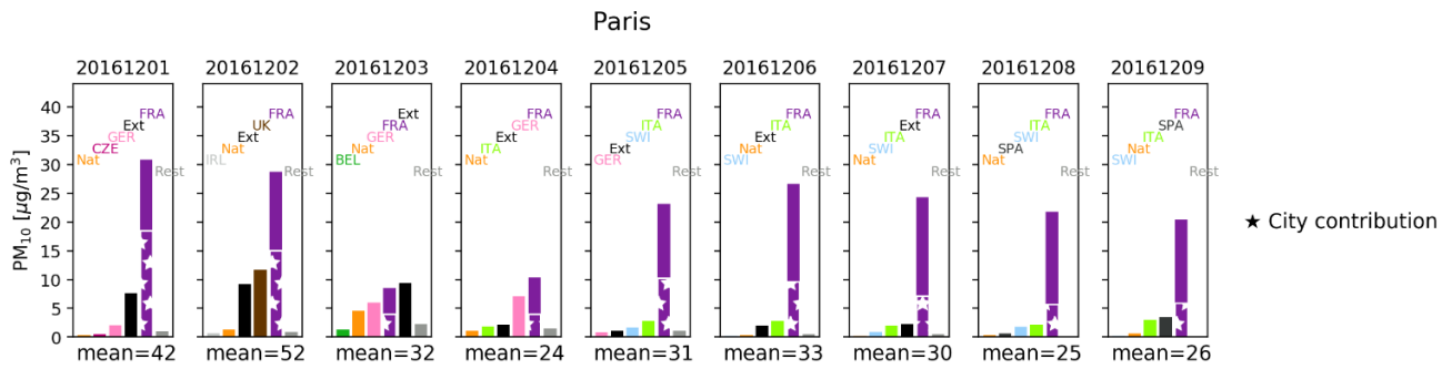
750 Figure 8: Main country contributors to surface PM 10 over Paris, defined by 9 grid cells, for each single day from 01 to 09 December 2016 predicted by the EMEP model (see Pommier et al., 2020). The five main contributors are plotted. The “Rest” is the difference between the daily mean and the sum of these five contributors. The “external” contributor (“Ext” on the figure) essentially corresponds to the countries not included in the country SC runs and the BCs. The “City” contribution is highlighted by white stars. The daily mean surface PM 10 concentration is written below each bar 755 chart. The labels BEL, CZE, FRA, GER, IRL, ITA, SPA, SWI, UK, refer to Belgium, Czechia, France, Germany, Ireland, Italy, Spain, Switzerland, and the United Kingdom, respectively.
