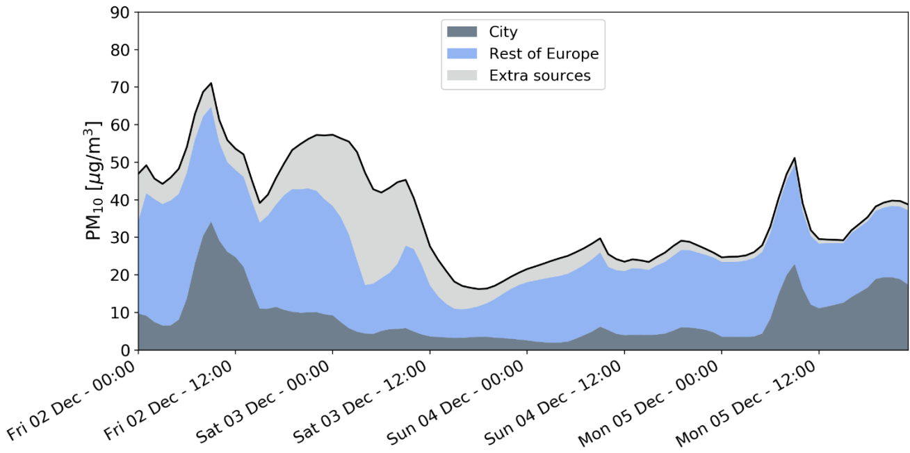
695 Figure 2: Hourly PM 10 concentrations in µg/m 3 predicted by the EMEP model over Paris (defined by 9 grid cells) from 02 December to 05 December 2016. The black curve highlights the total concentration. The “city”, “Rest of Europe” and “Extra sources” contributions are provided. “City” corresponds to the contribution from the area defined by 9 grid cells. “Rest of Europe” corresponds to all the European countries included in the regional domain and excluding the “City” contribution. “Extra sources” include the natural sources, the boundary conditions, the ship traffic, the biogenic sources, the soil NO emission, the aircraft emission and the lightning.
