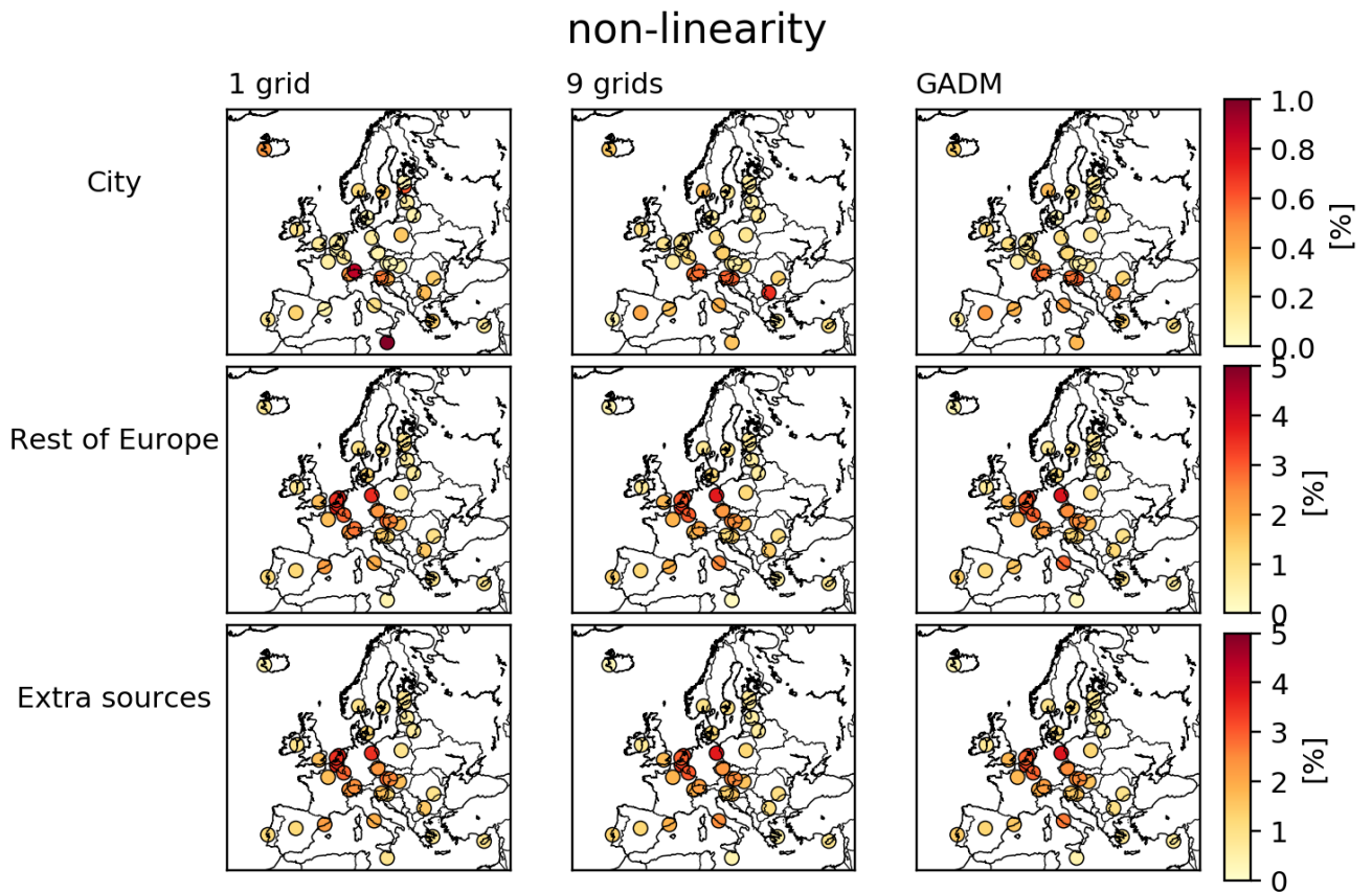
Figure 5: Mean non-linearity in percent calculated for the “City”, “Rest of Europe” and “Extra sources” contributions, over the 34 European cities and for each 4-day forecast (i.e. from 01-04 Dec to 09-12 Dec 2016). The non-linearity is presented for the cities defined by 1 grid (left row), 9 grids (middle row) and by the GADM (right row). Note the different scale to the “City” contribution compared to the two others.
