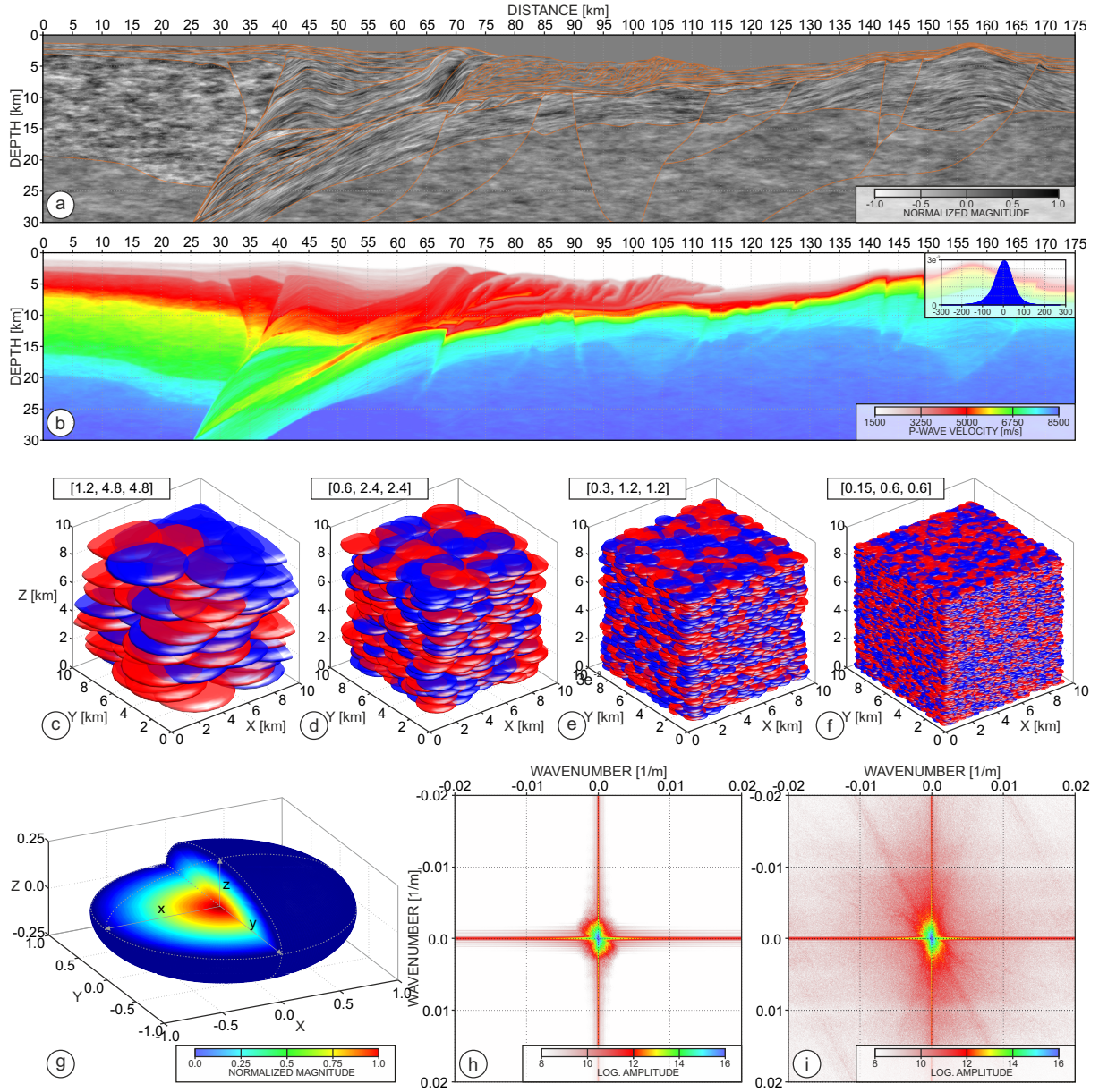
Figure 7. (a) Matrix of stochastic perturbations for a 2D inline section. (b) V_p model shown in Figure 4(c) after application of the stochastic perturbations shown in (a). (c-f) 3D stack of structural elements of different scales - see the correlation lengths in brackets. Red/blue colours indicate positive/negative magnitudes of the stacked structural elements. (g) Shape of the 3D structural element used to generate the stochastic perturbations. (h-i) Wavenumber spectrum of the 2D V_p inline section with and without stochastic perturbations.
