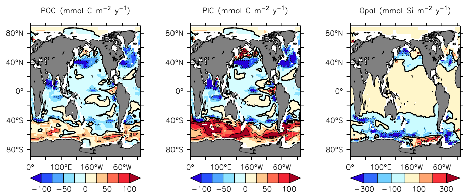
Figure 26. Modelled change in particle fluxes at 2 km depth, from 2014 to 2294.
