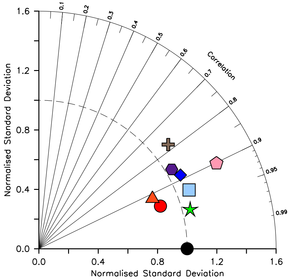
Figure 15. Taylor diagram (Taylor, 2001) of CMIP6 annual average dissolved silicon distribution (in \text{mol Si m}^{-3} ) for year 2014, normalised to the Garcia et al. (2014b) dataset. The distance to the origin represents the normalised standard deviation. Normalised correlation with observations is read from the azimuthal position. Perfect agreement with observations is a normalised standard deviation of 1 and a normalised correlation of 1. Models are KMBM3 (red circle), GFDL-ESM4 (green star; Krasting et al., 2018), CESM2 (light blue square; Danabasoglu, 2019), MPI-ESM1.2-LR (pink pentagon; Wieners et al., 2019), NorESM2-LM (brown plus; Seland et al., 2019), CMCC-ESM2 (orange triangle; Lovato et al., 2021), EC-Earth3-CC (blue diamond; EC-Earth Consortium, 2021), and IPSL-CM6A-LR (purple hexagon; Boucher et al., 2018). With the exception of KMBM3, the data for all models were obtained by mining the CMIP6 database ( https://esgf-node.llnl.gov/search/cmip6/ ) using the following search terms: CMIP/si/historical/annual output. Data were accessed between 01-05.02.2021.
