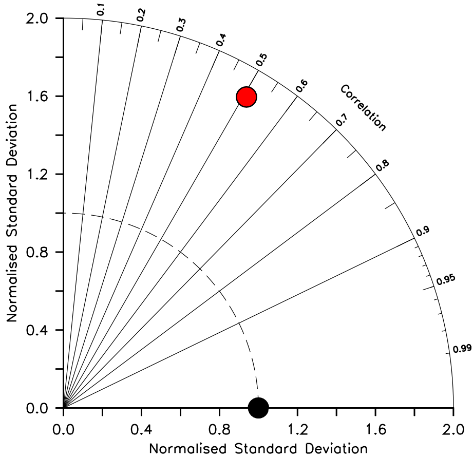
Figure 5. Taylor diagram (Taylor, 2001) of KMBM3 annual average diatom biomass concentrations (in \text{mol C m}^{-3} ) at year 2014 referenced to CMIP6 model mean diatom biomass. The distance to the origin represents the normalised standard deviation. Normalised correlation with mean CMIP6 concentrations is read from the azimuthal position. Perfect agreement with mean CMIP6 concentrations is a normalised standard deviation of 1 and a normalised correlation of 1. Normalisation against the model ensemble, rather than observations, is shown due to the models having greater similarity with each other than with the very sparse observations of diatom biomass currently available. Models are KMBM3 (red circle), and the black circle represents mean values from GFDL-ESM4 (Krasting et al., 2018), CanESM5-CanOE (Swart et al., 2019), CESM2 (Danabasoglu, 2019), CMCC-ESM2 (Lovato et al., 2021), EC-Earth3-CC (EC-Earth Consortium, 2021), and IPSL-CM6A-LR (Boucher et al., 2018). With the exception of KMBM3, the data for all models were obtained by mining the CMIP6 database ( https://esgf-node.llnl.gov/search/cmip6/ ) using the following search terms: CMIP/phydiat/historical/annual output. Data were accessed between 01-05.02.2021.
