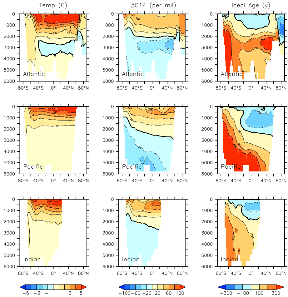
Figure 25. Modelled change in temperature, radiocarbon, and ideal age profiles by major ocean basin, from 2014 to 2296.
