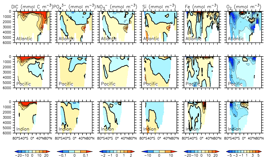
Figure 21. Modelled change in carbon and nutrient profiles by major ocean basin, from 1964 to 2014.
