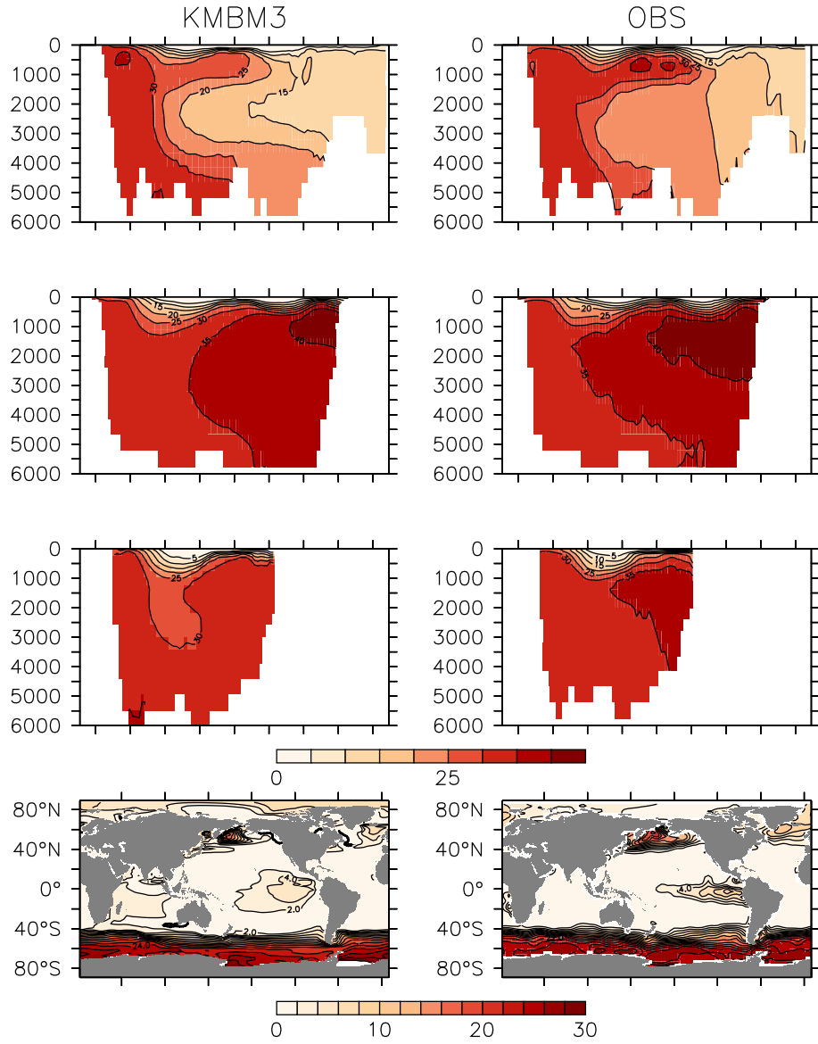
Figure 12. Model (left column) year 2014 \text{NO}_3^- ( \text{mmol m}^{-3} ) averaged by basin compared to WOA (right column; Garcia et al., 2014b). Regions are as follows: Atlantic (top row), Pacific (second row), Indian (third row) and global surface (bottom row).
