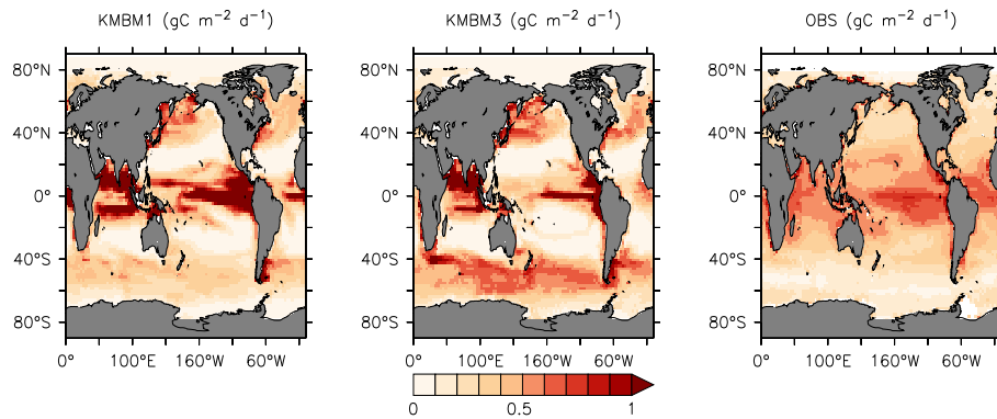
Figure 2. Comparison of model NPP output at 2014 (left panel; Keller et al. (2012), and middle panel; this model) and satellite-derived NPP climatology (NASA, 2018), 2012-2018 (right panel) in gC\ m^{-2}\ day^{-1} .
