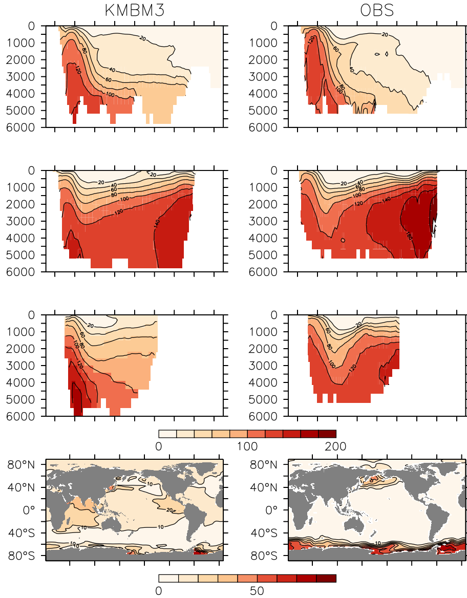
Figure 14. Model (left column) year 2014 Si ( \text{mmol m}^{-3} ) averaged by basin compared to WOA (right column; Garcia et al., 2014b). Regions are as follows: Atlantic (top row), Pacific (second row), Indian (third row) and global surface (bottom row).
