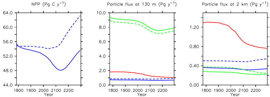
Figure 20. Major biogeochemical fluxes in the model, 1776 to 2300. Left panel is total net primary production, middle panel is total particle fluxes at 130 m depth, right panel is total particle fluxes at 2 km depth. Blue lines in the middle and right panels are PIC, green lines are POC, red lines are opal. Solid lines are from this model (KMBM3), dashed lines from the Keller et al. (2012) version (KMBM1).
