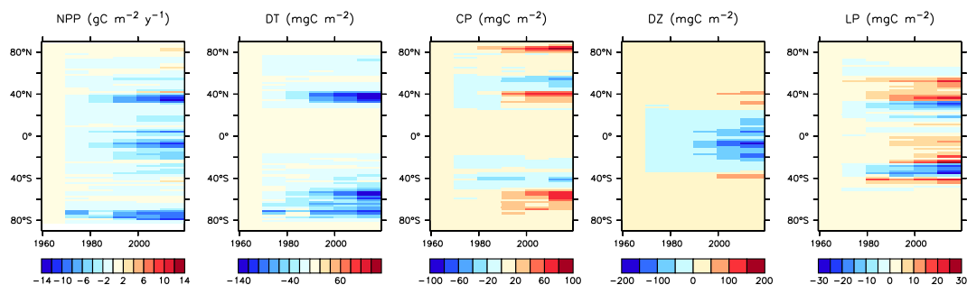
Figure 17. Modelled historical changes in zonally averaged and depth integrated NPP, and phytoplankton biomass, from 1964 to 2014.
