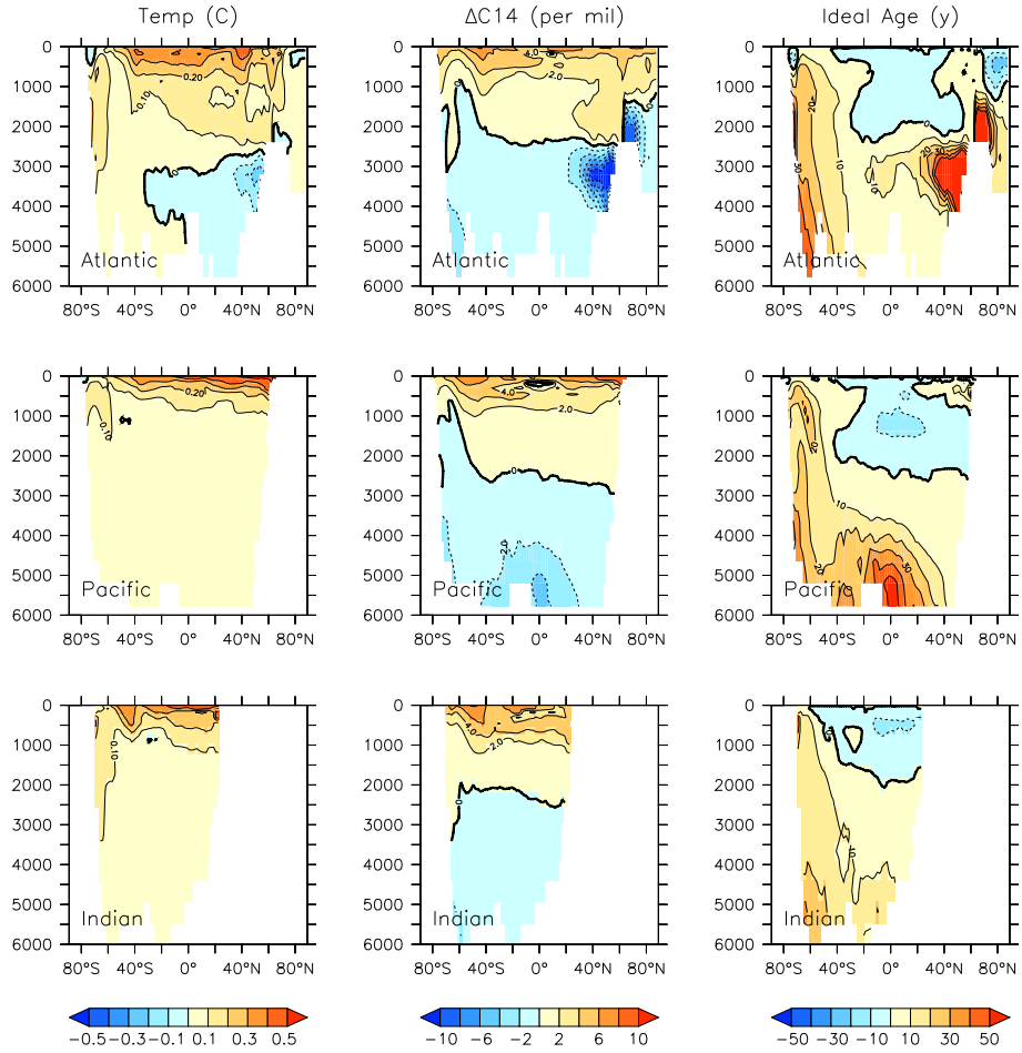
Figure 19. Modelled change in temperature, radiocarbon, and ideal age profiles by major ocean basin, from 1964 to 2144.
