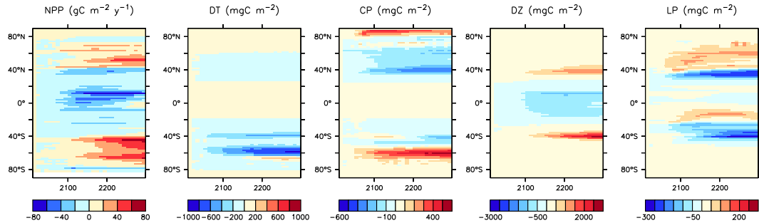
Figure 24. Modelled changes in zonally averaged and depth integrated NPP, and phytoplankton biomass, from 2014 to 2294.
