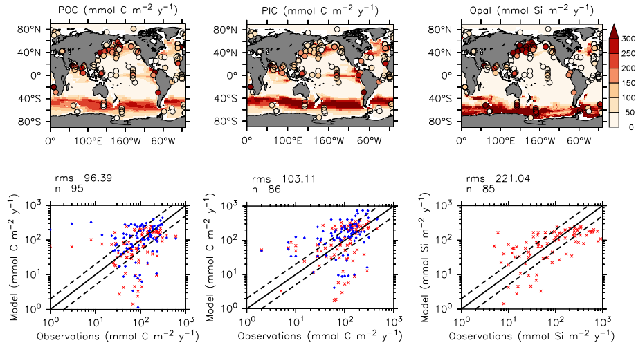
Figure 6. Comparison of model POC (left panels), \text{CaCO}_3 (middle panels), and opal (right panels) fluxes at year 2004 and 2 km depth with Honjo et al. (2008) data. Red points are this model (KMBM3), blue points are the Keller et al. (2012) model (KMBM1). Statistics are given for KMBM3 only.
