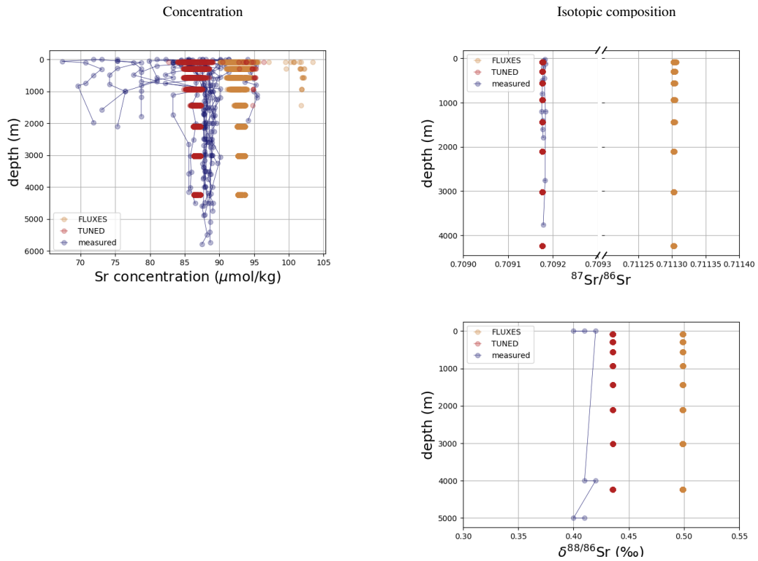
Figure B5. Comparison between measured and simulated Sr profiles in seawater. Shown are composites of all available measured Sr concentration and isotope ratio profiles and all profiles in the simulation. Data is taken from Angino et al. (1966), Fabricand et al. (1967), Bernat et al. (1972), Brass and Turekian (1974), De Villiers (1999) and Mokadem et al. (2015). Sr concentrations are normalized to a salinity of 34.903495.
