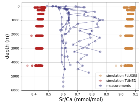
Figure B8. Comparison between measured and simulated Ca and Sr/Ca profiles in seawater. Shown are composites of all available measured concentration profiles and all profiles in the simulation. Data is taken from Fabricand et al. (1967), De Villiers (1999) and Fantle and Tipper (2014). Ca concentrations are normalized to a salinity of 34.903495.
