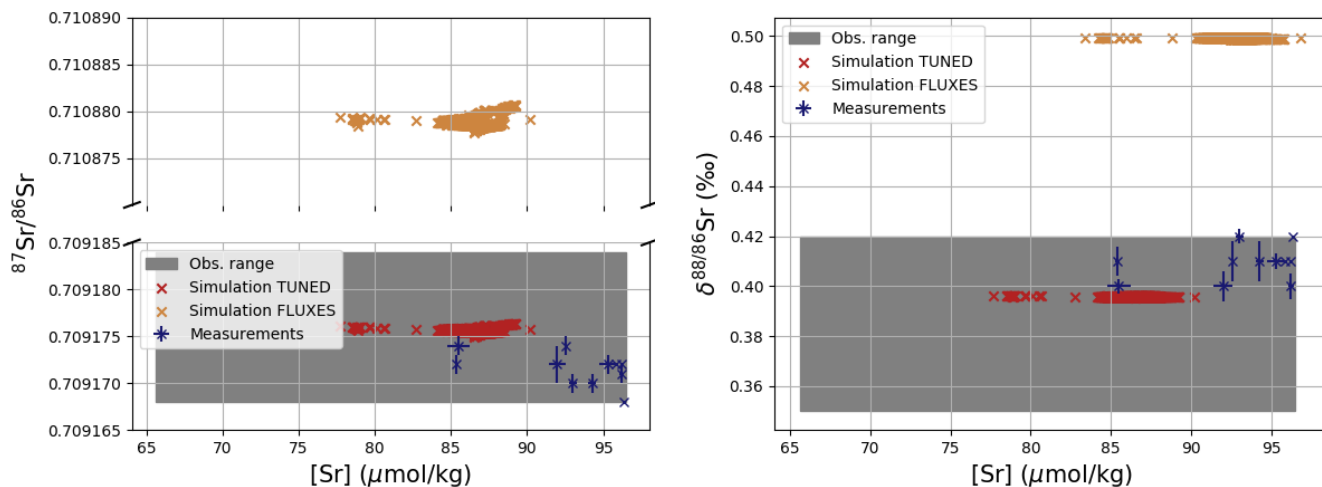
Figure 3. Comparison between measured and simulated concentrations and isotopic composition of dissolved Sr in seawater. The displayed data points are paired measurements of Sr concentrations and isotope ratios (Wakaki et al., 2017), while the gray box also indicates the full range of concentrations and isotopic compositions (separate measurements of Sr concentration or isotope ratios) (Angino et al., 1966; Fabricand et al., 1967; Bernat et al., 1972; Brass and Turekian, 1974; De Villiers, 1999; Mokadem et al., 2015). Observations and model results are salinity-normalized.
