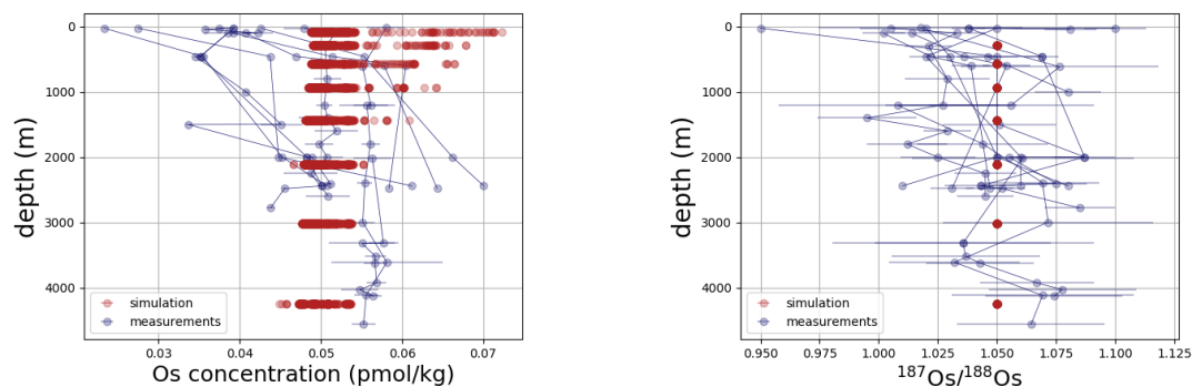
Figure B6. Comparison between measured and simulated Os vertical profiles in seawater. Shown are composites of all available measured Os concentration and isotope ratio profiles and all profiles in the simulation. Data is taken from Levasseur et al. (1998), Woodhouse et al. (1999) and Gannoun and Burton (2014).
