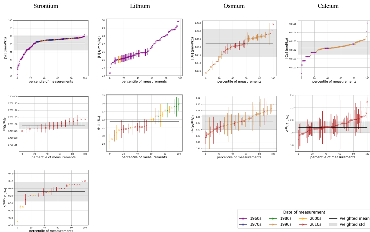
Figure 1. Sr, Li, Os and Ca composition of modern seawater. Shown are composites of all published measured concentrations and isotope ratios with reported errors. From these, we calculated mean concentrations and isotope ratios weighted by the reported error (the more uncertain a value, the less it contributes to the mean), which are indicated by horizontal lines. Shading indicates one weighted standard deviation around the means. Data are taken from Angino et al. (1966), Fabricand et al. (1967), Bernat et al. (1972), Brass and Turekian (1974), De Villiers (1999), Pearce et al. (2015), Mokadem et al. (2015) and the compilation of Wakaki et al. (2017) for Sr, Angino and Billings (1966), Fabricand et al. (1967), Chan (1987), Chan and Edmond (1988), You and Chan (1996), Moriguti and Nakamura (1998), Tomascak et al. (1999), James and Palmer (2000), Košler et al. (2001), Nishio and Nakai (2002), Hall (2002), Bryant et al. (2003), Pistiner and Henderson (2003), Millot et al. (2004), Choi et al. (2010), Pogge von Strandmann et al. (2010), Phan et al. (2016), Lin et al. (2016), HENCHIRI et al. (2016), Weynell et al. (2017), Fries et al. (2019), Gou et al. (2019), Hindshaw et al. (2019), Murphy et al. (2019) and Pogge von Strandmann et al. (2019) for Li, LévassEUR et al. (1998), Woodhouse et al. (1999) and Gannoun and Burton (2014) for Os and Fabricand et al. (1967), De Villiers (1999) and Fantle and Tipper (2014) for Ca. The decade of publication is indicated by colour as measurement techniques for some metals/isotopes have improved over time. Concentrations of Sr, Li and Ca are normalized to a salinity of 34.903495. Os concentrations could not be salinity-normalized because of missing salinity measurements at one out of three measurement sites (Woodhouse et al., 1999).
