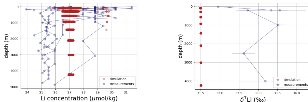
Figure B7. Comparison between measured and simulated Li profiles in seawater. Shown are composites of all available measured Li concentration and isotope ratio profiles and all profiles in the simulation. Data is taken from Angino and Billings (1966), Fabricand et al. (1967), Chan (1987), Chan and Edmond (1988), You and Chan (1996), Moriguti and Nakamura (1998), Tomascak et al. (1999), James and Palmer (2000), Košler et al. (2001), Nishio and Nakai (2002), Hall (2002), Bryant et al. (2003), Pistiner and Henderson (2003), Millot et al. (2004), Choi et al. (2010) and Lin et al. (2016). Li concentrations are normalized to a salinity of 34.903495.
