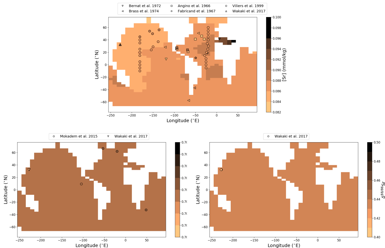
Figure C1. Comparison between measured and simulated Sr concentrations and isotopic composition in surface waters. Measurements are shown as symbols on the map, the colour indicating the respective value. Data is taken from Angino et al. (1966), Fabricand et al. (1967), Bernat et al. (1972), Brass and Turekian (1974), De Villiers (1999), Mokadem et al. (2015) and Wakaki et al. (2017).
