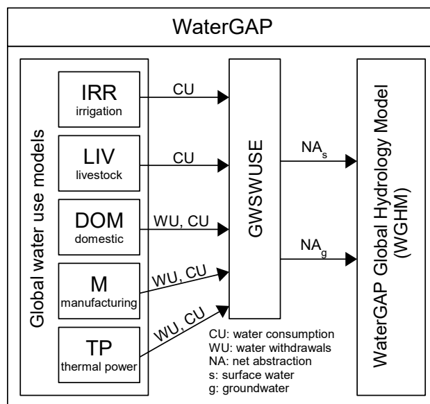
Figure 1. The WaterGAP 2.2d framework with its water use models and the linking module GWSWUSE that provides net water abstraction from groundwater and surface water as input to the WaterGAP Global Hydrology Model (WGHM). Figure adapted from Müller Schmied et al. (2014).
