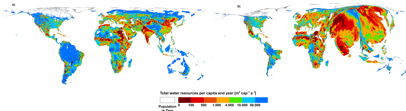
Figure 14. Water availability indicator per capita renewable water resources Q_{r,out,lt,nat} ( \text{m}^3 \text{cap}^{-1} \text{yr}^{-1} ) for 1981–2010 visualized in a) an equal area projection and b) as a cartogram with population in 2010 as distorter. In the cartogram each half degree grid cell is distorted such that its area is proportional to the population of the grid cell.
