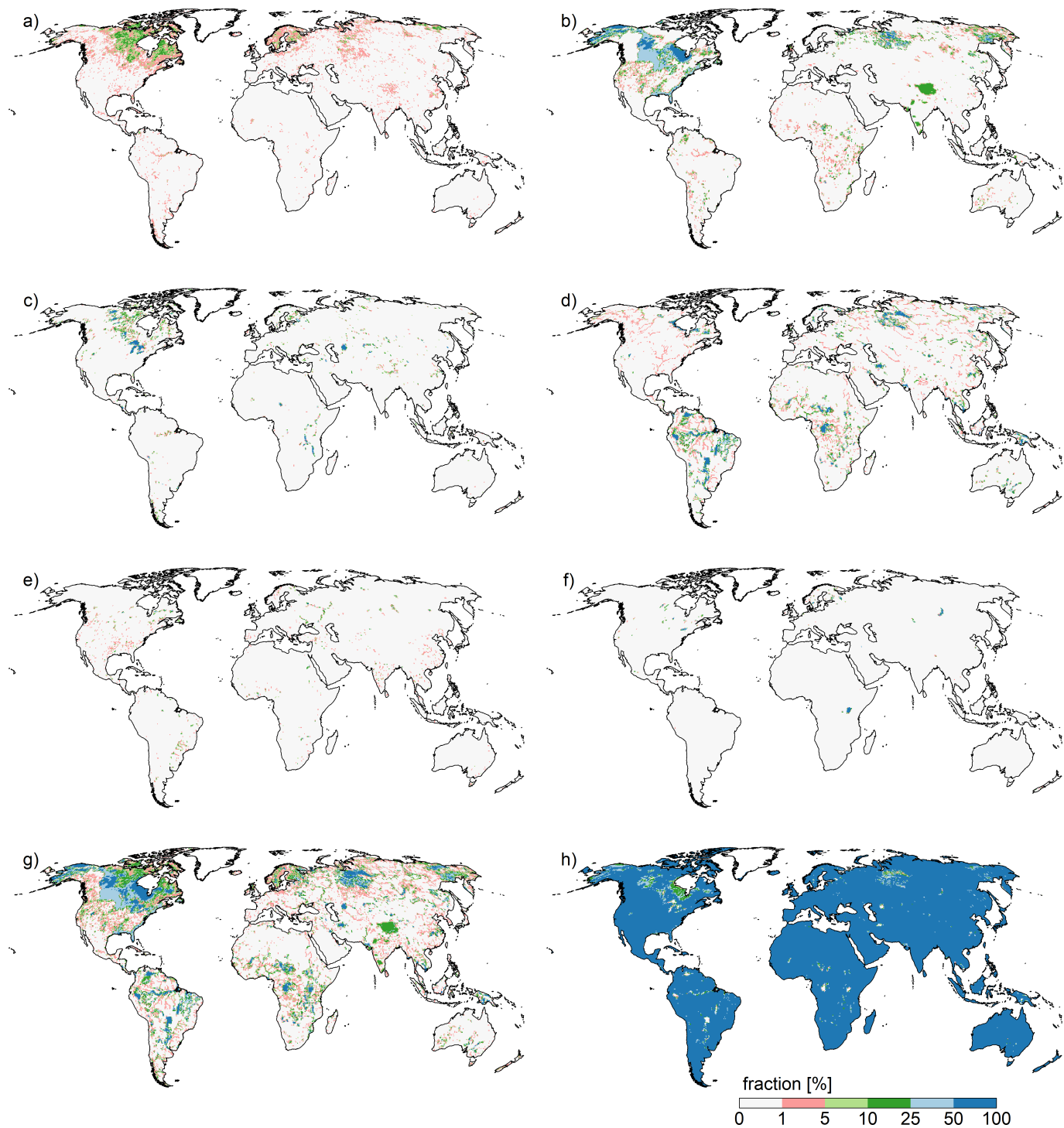
Figure E1. figure single fractions and sum grid cell area covered (maximum extent) and land fraction (minimum)
