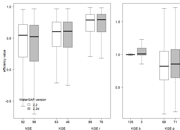
Figure D5. Efficiency of streamflow for the 1319 river basins in comparison of model versions WaterGAP 2.2d and WaterGAP 2.2 showing similar model performance. Outliers are excluded but number of outliers indicated at x axis.
