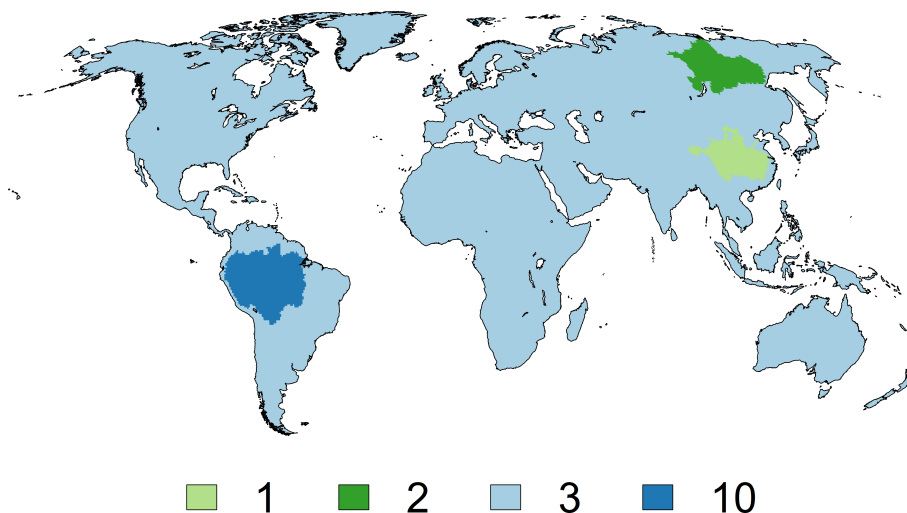
Figure D3. Region-specific multiplier for river roughness.
