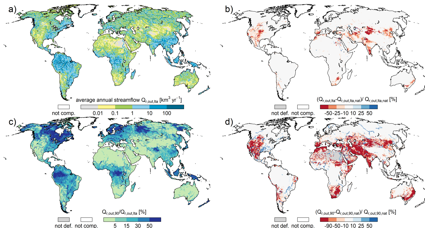
Figure 12. Streamflow indicators of WaterGAP 2.2d for 1981-2010 with a) long-term average annual streamflow Q_{r,out,lta} , ( \text{km}^3 \text{ yr}^{-1} ), b) indication of streamflow alteration due to human water use and man-made reservoirs, reddish indicates less streamflow for ant conditions, blue the opposite, c) statistical monthly low flow Q_{r,out,90} in percent of Q_{r,out,lta} , d) differences of long term average statistical monthly low flows as indication of low flow alteration due to human water use and man-made reservoirs. Not defined are areas where the denominator is smaller than 10^{-5} \text{ km}^3 \text{ yr}^{-1} .
