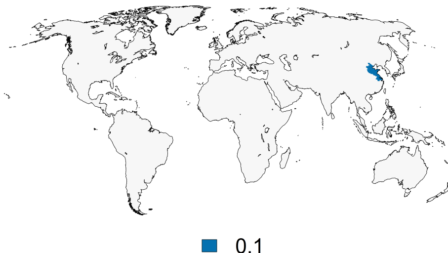
Figure D2. Regional correction of calibration parameter \gamma to allow more realistic groundwater recharge rates.
