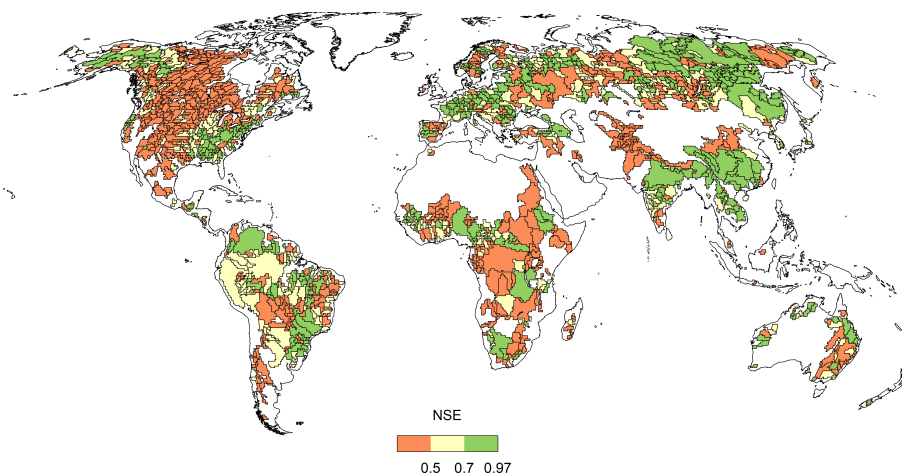
Figure D7. Classified NSE efficiency metric represented for the 1319 river basins and WaterGAP 2.2.
