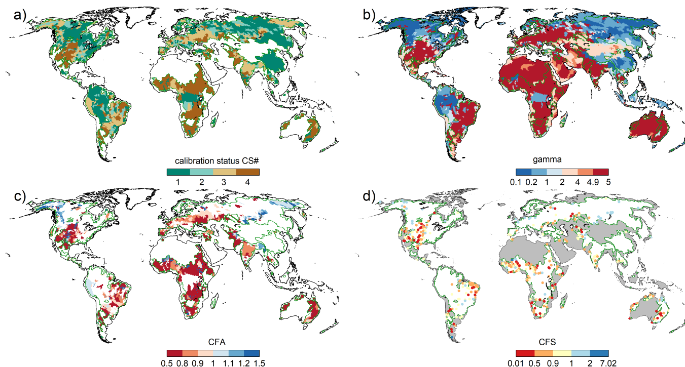
Figure 4. Results of the calibration of WaterGAP 2.2d to the standard climate forcing with a) the calibration status (see Sect. 4.9.1) of each calibration basin b) calibration parameter \gamma , c) areal correction factor CFA, and d) station correction factor CFS. Grey areas in d) indicate regions with regionalized calibration parameter \gamma and for a-d) dark green outlines indicate the boundaries of the calibration basins.
