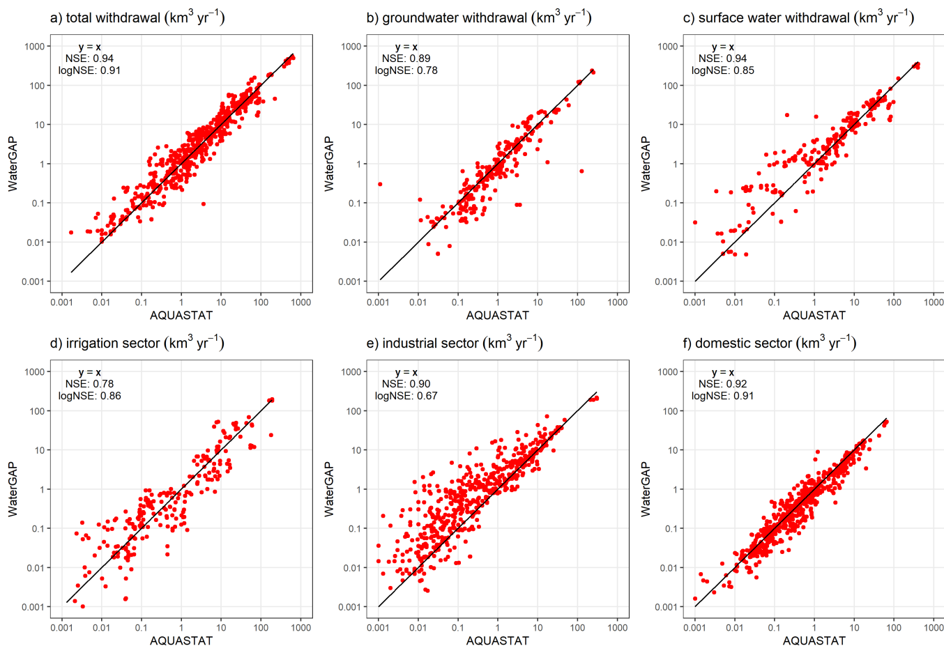
Figure 5. Comparison of potential withdrawal water uses from WaterGAP 2.2d with AQUASTAT (FAO - AQUASTAT). Each data point represents one yearly value (if present in the database) per country for the time span 1962-2016
