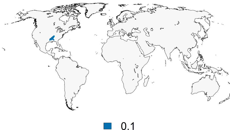
Figure D1. Regional correction of the groundwater factor f_g to allow more realistic groundwater recharge rates.
