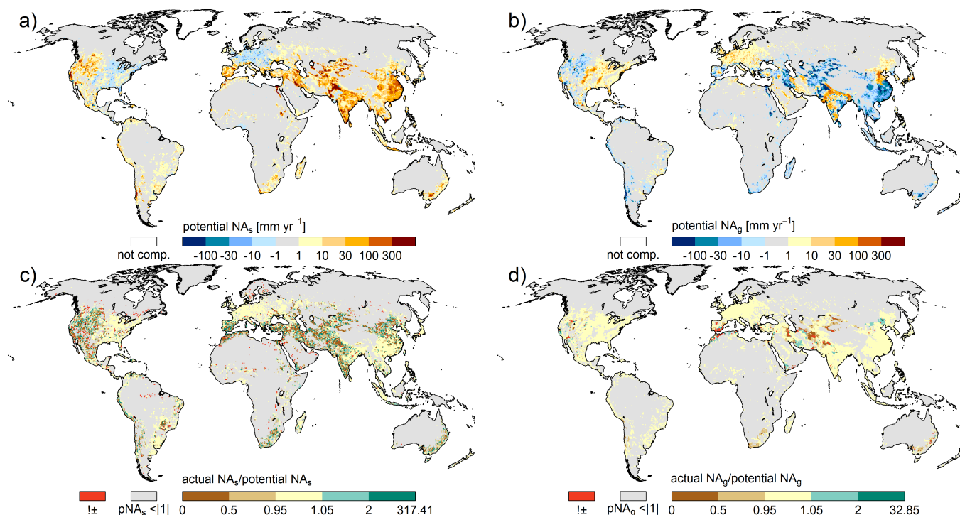
Figure 15. Long term (1981-2010) annual net abstractions: potential net water abstractions from surface water bodies a), potential net water abstractions from groundwater b), ratio of actual net water abstractions from surface water bodies to its potential value c) and ratio of actual net water abstractions from ground water to its potential value. In a) and b) negative values indicate a net recharge of surface water and groundwater, respectively, due to return flows caused by human water use, while positive values indicate a net removal of water from the sources. In c) and d), cells with potential net water abstractions smaller than 1 \text{ mm yr}^{-1} are greyed out. Furthermore, grid cells where the sign of water abstractions changes between potential and actual net abstractions are displayed in red.
