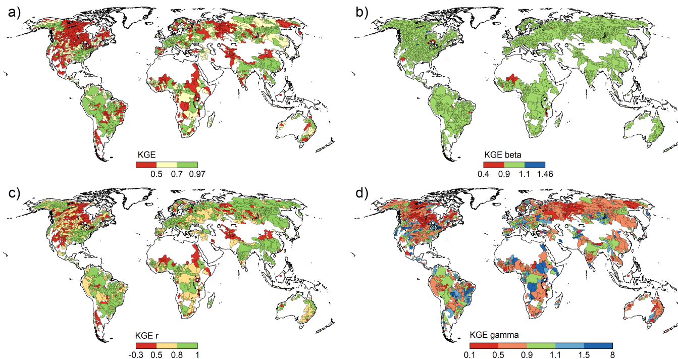
Figure D4. KGE and its components range at 1319 river basins for WaterGAP 2.2
