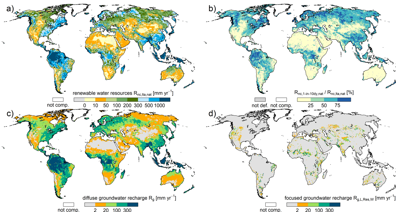
Figure 11. Water resources assessment 1981-2010 using WaterGAP 2.2d, with a) total renewable water resources defined as long-term annual net cell runoff R_{nc,lt,a,nat} [ \text{mm yr}^{-1} ], b) 1-in-10 dry year runoff generation in percent of total renewable water resources [%], c) long-term annual diffuse groundwater recharge R_g [ \text{mm yr}^{-1} ], d) long-term annual focused groundwater recharge R_{g,L,Res,W} [ \text{mm yr}^{-1} ]. Results are based on naturalized model runs. In a) note that negative values for total water resources are possible (Sect. 4.7.3). In b) areas where the denominator is < 10^{-5} are labelled as not defined.
