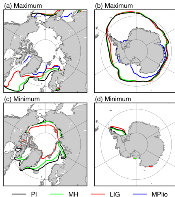
485 Figure 11. Sea ice edge in the Arctic (a, c) and Antarctic (b, d) in the maximum (a, b) and minimum (c, d) SIE month in each simulation. Maximum sea ice extents occur in March in the Arctic, and in September in the Antarctic, while minimum sea ice extents are seen in August in the Arctic, and in February in the Antarctic.
