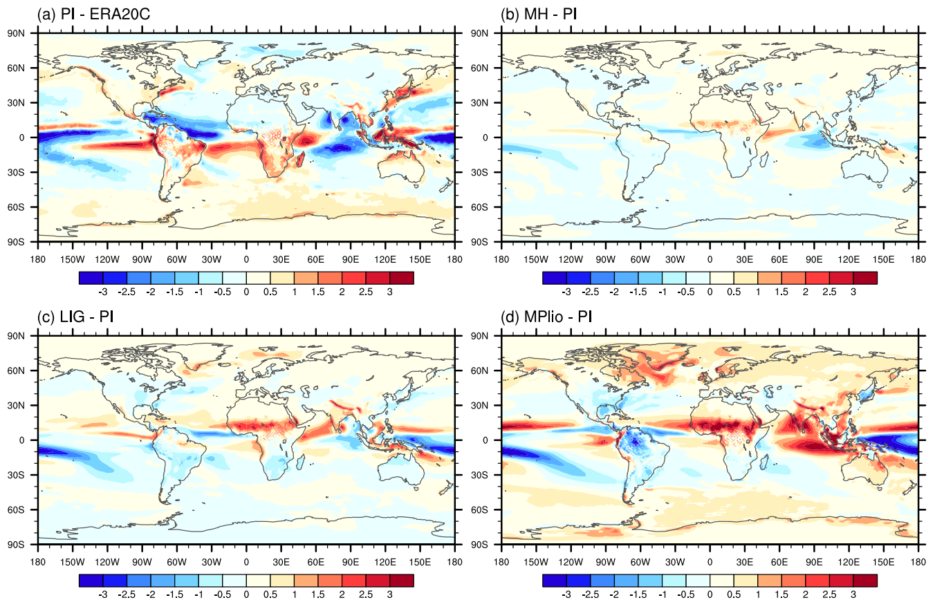
Figure 6. Mean annual precipitation ( \text{mm d}^{-1} ) in (a) difference between the piControl and ERA20C (1901-1930 mean), and 310 the anomaly in the (b) the midHolocene , (c) the lig127k and (d) the midPliocene from the piControl .
