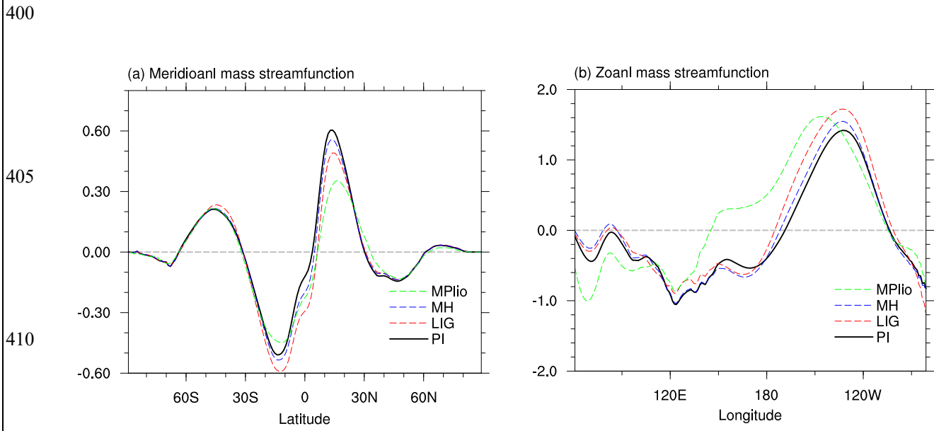
415 Figure 9. The zonal (a) and meridional (b) mean of vertical integrated meridional and zonal mass stream function in Figure 5. Unit: 10^{10} \text{ kg s}^{-1} .
