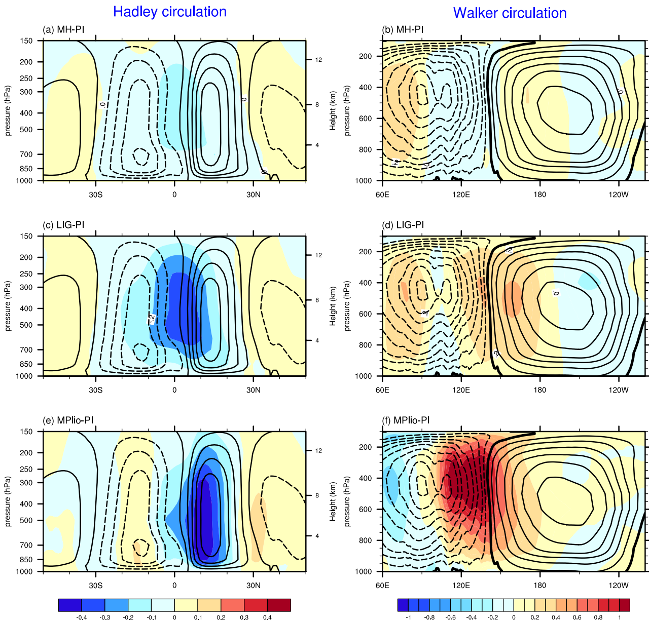
Figure 8. The changes in annual mean Hadley circulation (represented by zonal-mean meridional mass stream function in the left panel) and Walker circulation (represented by zonal mass stream function averaged between 10° S~10° N over Indo-Pacific region 60° E-150° W in the right panel). The shadings indicate the changes in (a, b) the midHolocene , (c, d) the lig127k and (e, f) the midPliocene respect to piControl . The contours represent the climatology from the piControl simulation (solid contours indicate positive value and dashed contours indicate negative value). Units: 10^{10} \text{ kg s}^{-1} .
