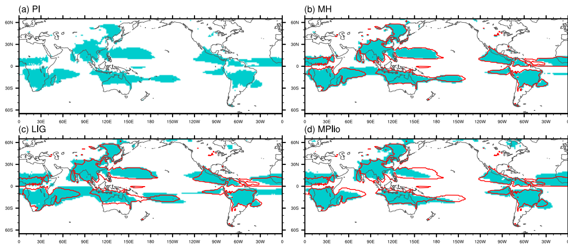
505 Figure 12. Global monsoon area in (a) the piControl , (b) the midHolocene , (c) the lig127k , (d) the midPliocene simulation, with piControl global monsoon boundary as a red line in b-d.
