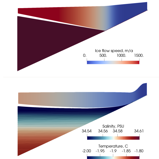
Figure 6. Profiles through the center line for experiment VE2 after the first ice component time step (top) and after 25 years (bottom). Ice flow speed is shown (flow direction is right to left). Ocean temperature (solid colour) and salinity (contours) are shown after 25 years (these are uniform at the start of the run, hence the solid colour for the ocean in the upper plot). Vertical exaggeration is 50 times. The gap between ocean and ice shelf is half an ocean grid cell and is a plotting artefact (The upper extent of the plotted region for the ocean is the uppermost rho point, which is half an ocean grid cell below the top of the ocean domain).
