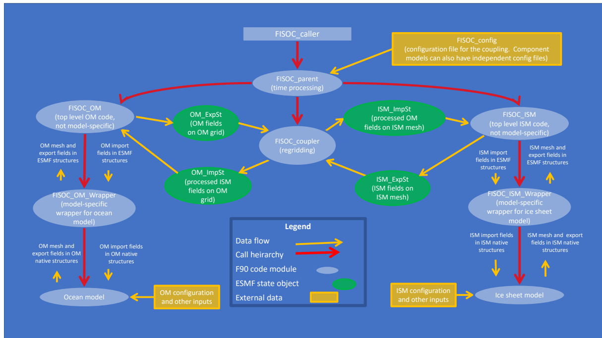
Figure 1. Overview of FISOC code structures. “OM” and “ISM” are short for Ocean and Ice Sheet Model (or component) respectively. “ImpSt” and “ExpSt” are short for Import and Export State respectively.
