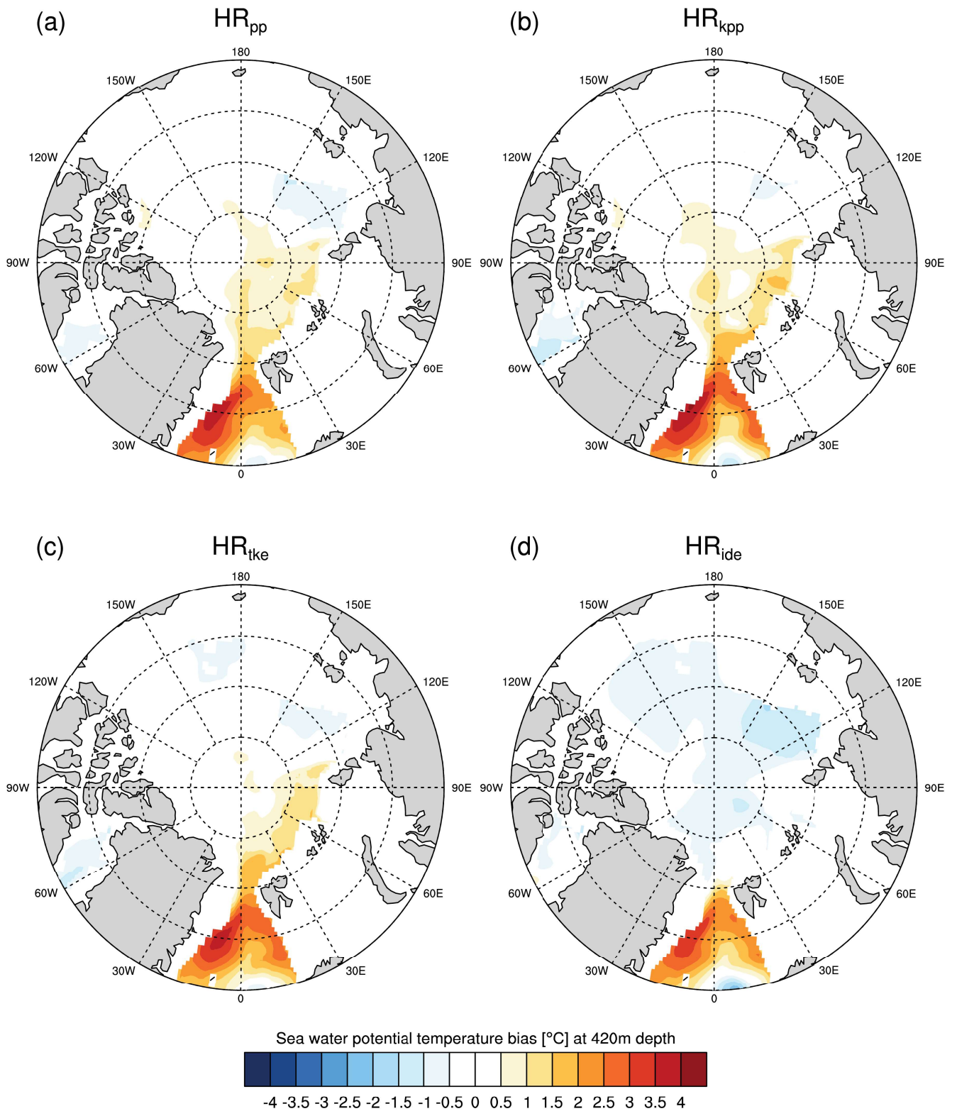
Figure 14. Time-averaged potential temperature bias of MPI-ESM1.47HR minus EN4 (1945-1955) at a depth of 420 m in the Arctic Ocean and at Fram Strait for (a) HR_{pp} , (b) HR_{kpp} , (c) HR_{tke} , and (d) HR_{ide} .
