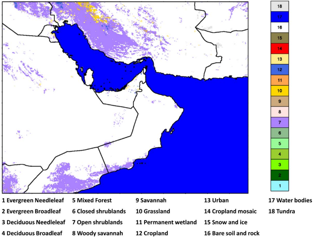
Figure 4: Map of whole model domain with the land cover data set used in the simulation. It is a composite of the standard 30 arc second (~1-km) IGBP 21-class MODIS dataset included as standard with WRF, with two local datasets superimposed: Abu Dhabi and Dubai Emirates, obtained respectively from the Environment Agency of Abu Dhabi (EAD) and the International Center for Biosaline Agriculture (ICBA) in Dubai. The local datasets were first reclassified in a logical manner into MODIS categories. 18 classes are shown here. There is a reduction in resolution due to the grid increment of 2.7 km.
