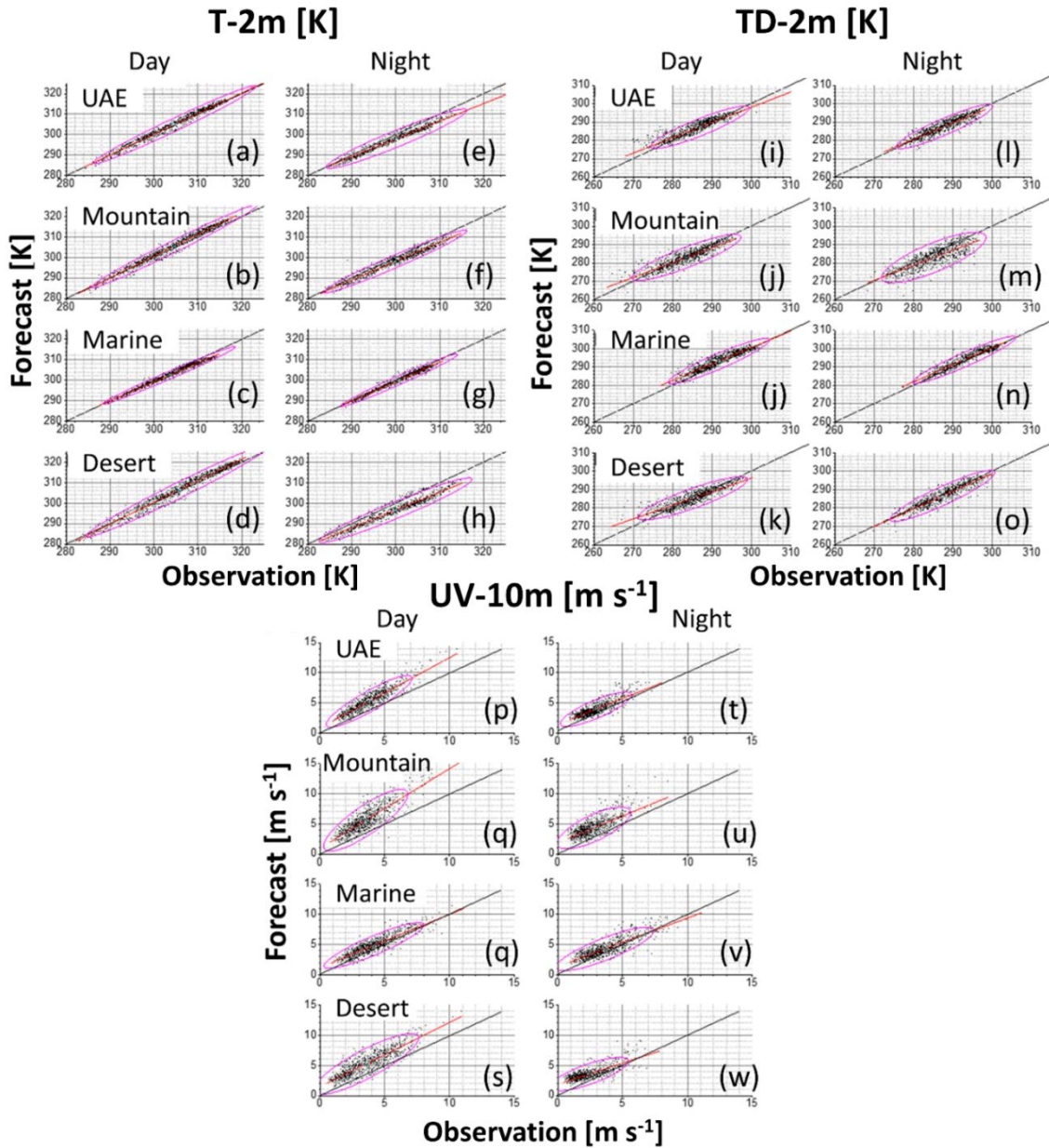
20 Figure 5: Scatter plots of forecast vs observation for all time steps over the period of January-November 2015, comparing each weather station at the corresponding WRF grid point. The plots are split by day-time (left panels) and night-time periods (right) (respectively, day 06:00-17:00 (left panels) and night 18:00-05:00 (right) in local time), and by region (UAE, Mountain, Marine, Desert). The variables compared are 2-m air temperature (T-2m, K) in panels (a – h), 2-m dew point (T D -2m, K) in panels (i – o), and 10-m wind speed (UV-10m, m s -1 ) in panels (p – w). Also shown is a line of best fit (red) and a line of perfect fit (black), and 95% confidence ellipse (magenta).
