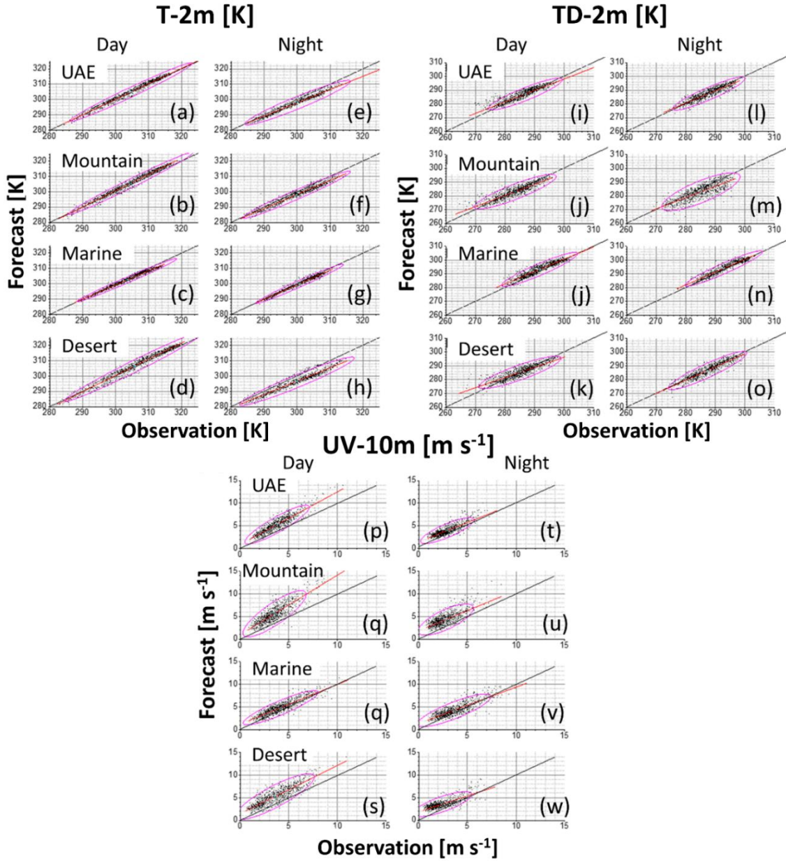
Figure 5: Scatter plots of forecast vs observation vs forecast for all time steps over the period of January–November 2015, comparing each weather station at the corresponding WRF grid point. The plots are split by day-time (left panels) and night-time periods (right) (respectively, day 06:00–17:00 (left panels) and night 18:00–05:00 (right) in local time), and by region (UAE, Mountain, Marine, Desert). The variables compared are 2-m air temperature (T-2m, K) in panels (a – h), 2-m dew point (T D -2m, K) in panels (i – o), and 10-m wind speed (UV-10m, m s -1 ) in panels (p – w). Also shown is a line of best fit (red) and a line of perfect fit (black), and 95% confidence ellipse (magenta).
