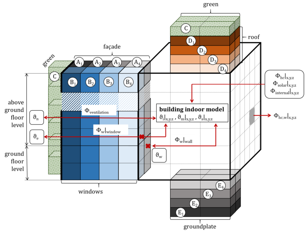
Figure 2: Integration of the building indoor model (red darts) with the independent driving forces \Phi_{solar} , \Phi_{internal} , and \Phi_{hc} into the building surface model ( \vartheta_w ) and the PALM model ( \vartheta_n and \vartheta_e ) considering the coupled driving forces \Phi_{ventilation} , \Phi_{w|window} , and \Phi_{w|wall} . A- E are five façade types (consisting of different materials) and 1-4 are the four layers for each façade. Additionally, the
