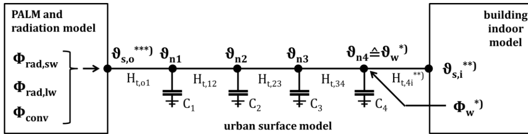
360 Figure 3: Building surface model. Heat flows \Phi and temperatures \vartheta in the R4C4 network. *) The wall temperature \vartheta_{n4} is the model output to the building indoor model \vartheta_w , and the heat flow into the wall \Phi_w is the input from the building indoor model. **) The heat flow at the inside surface is calculated by the building indoor model. Hence, H_{t,4i} is equal to H_{t,ws} in the building indoor model. ***) The temperature at the outside surface \vartheta_{s,o} is calculated with input variables from the PALM model and the radiation model.
