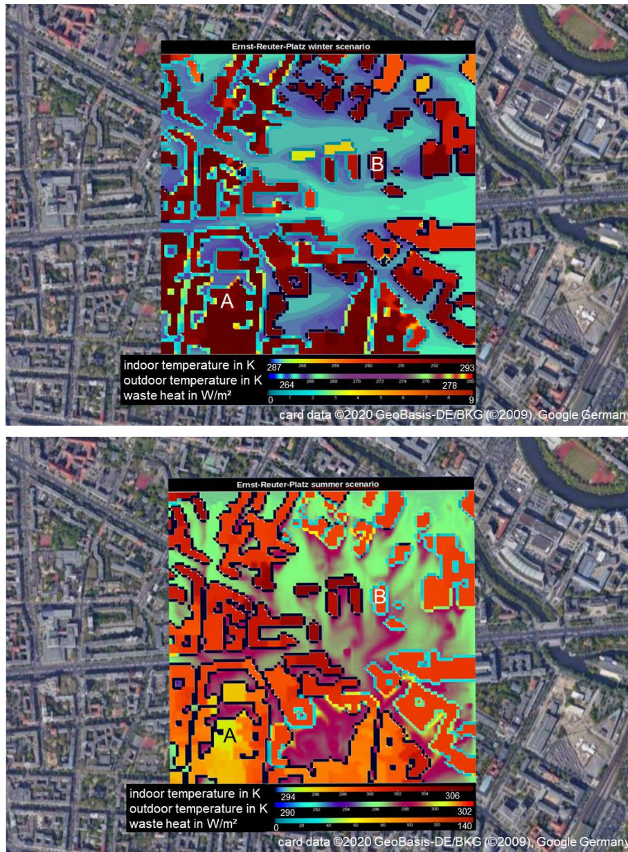
365 Figure 4: Building surface and building indoor model in a test setup. The Ernst-Reuter-Platz connects five urban street canyons and is surrounded by high-rise buildings. The simulation runs with a resolution of 1 m x 1 m x 1m. The graphs show the operative room temperature \vartheta_i , the ambient air temperature \vartheta_e and the anthropogenic waste heat \Phi_{hc,w} at the outside surface. The outdoor temperature is around +24 °C in the summer scenario (above) and -10 °C in the winter scenario (below). Façade elements with no anthropogenic waste heat (i.e. buildings with district heating in winter or passive cooling in summer, respectively) are shown in 370 black.
