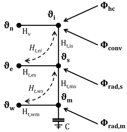
Figure 1: Building indoor model. Heat flows \Phi and temperatures \vartheta in the R5C1 network. The dashed lines show the energy flow \Phi_w between the building indoor model and the building surface model.
