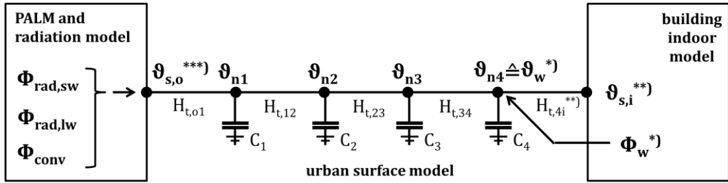
Figure 3: Building surface model. Heat flows \Phi and temperatures \vartheta in the R4C4 network. *) The wall temperature \vartheta_{n4} is the model output to the building indoor model \vartheta_w , and the heat flow into the wall \Phi_w is the input from the building indoor model. **) The heat flow at the inside surface is calculated by the building indoor model. Hence, H_{t,4i} is equal to H_{t,ws} in the building indoor model. ***) The temperature at the outside surface \vartheta_{s,o} is calculated with input variables from the PALM model and the radiation model.
