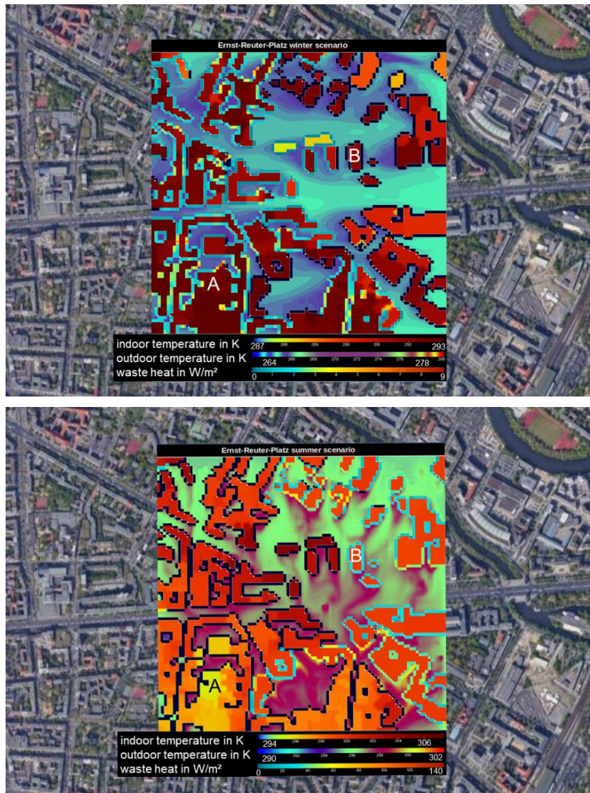
Figure 4: Building surface and building indoor model in a test setup. The Ernst-Reuter-Platz connects five urban street canyons and is surrounded by high-rise buildings. The simulation runs with a resolution of 1 m x 1 m x 1m. The graphs show the operative room temperature \vartheta_i , the ambient air temperature \vartheta_e and the anthropogenic waste heat \Phi_{hc,w} at the outside surface. The outdoor temperature is around +24 °C in the summer scenario (above) and -10 °C in the winter scenario (below). Façade elements with no anthropogenic waste heat (i.e. buildings with district heating in winter or passive cooling in summer, respectively) are shown in black.
