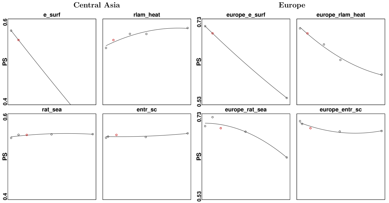
Figure 11. PS values calculated for Central Asia ( left ) and Europe ( right ), for different values of the parameters e\_surf , rlam\_heat , rat\_sea and entr\_sc . The values of the parameters are the same in the two cases. Red dots represent correspond to the considered parameter PS values obtained for the default simulation.
