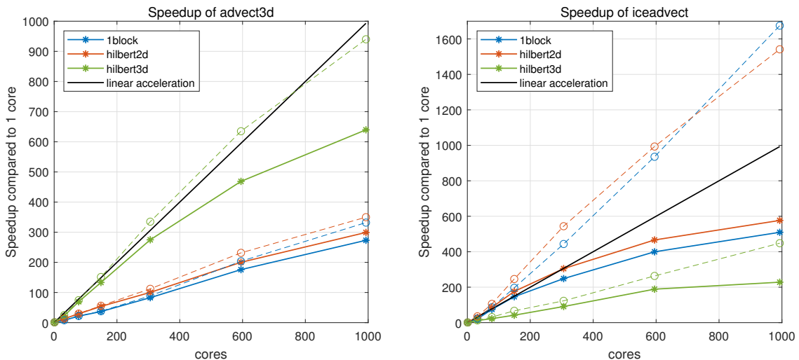
Figure 4. Speedup compared to one core for two functions: advect3d and iceadvect . Solid/dashed lines correspond to measurements with/without MPI-exchanges / MPI exchanges , respectively. Different partitions are shown in colour (1block, hilbert2d, and hilbert3d).
