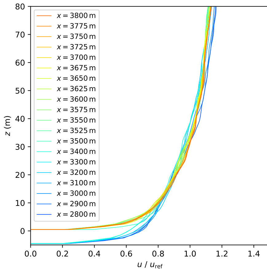
Fig. 1. Time averaged vertical profiles of the normalized u component from the PALM simulation at several x coordinates at y=1400\text{m} .
