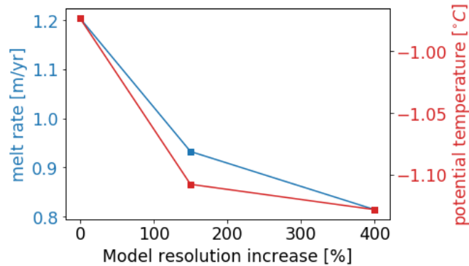
Figure 4. Grid convergence. Annual means of average melt rate and continental shelf potential temperature resolved at the different horizontal resolutions: 10 km (0 % increase), 4 km (150 % increase) and 2 km (400 % increase). Continental shelf temperatures have been calculated for depths shallower than 1500 m and including the ice shelf cavities (see Fig. 1). Continental shelf processes converge when grid spacing is refined.
