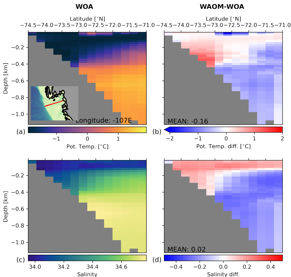
Figure 12. As Fig. 11, but for a transect across the Amundsen Seas along 107^{\circ}\text{W} .
