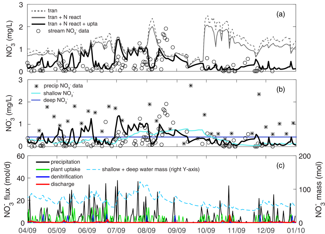
Figure 8. Stream nitrate dynamics and fluxes at Shale Hills in Example 2. (a) Three simulation scenarios with different processes are demonstrated here: transport only (dashed line, tran ), transport + N reaction (gray line, tran + N react ), transport + N reaction + plant uptake (thick black line, tran + N react + upta ), where N reactions include both nitrate leaching and denitrification (see Fig. 7); (b) nitrate concentration in precipitation and shallow and deep water; (c) nitrate fluxes and budget. Note that nitrate leaching was ignored in (b) due to its minimal flux as N deposition from rainfall was the dominant input (Weitzman and Kaye, 2018).
