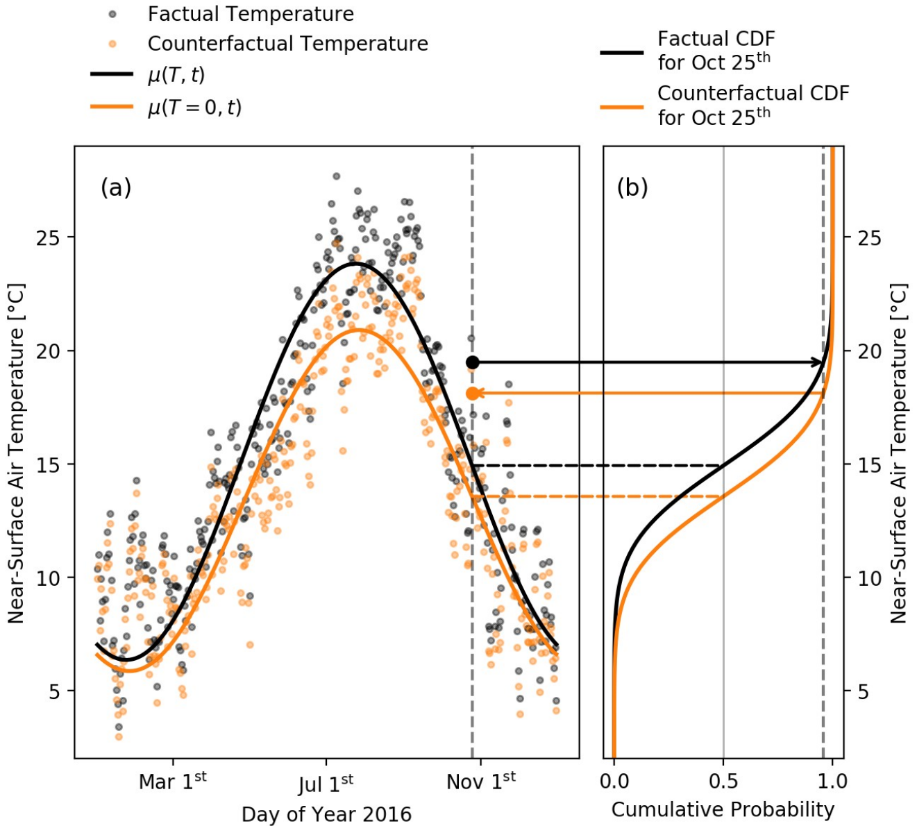
Figure 4. Illustration of detrending with quantile mapping sensitive to the annual cycle. Panel (a) shows factual (black points) and counterfactual (orange points) daily mean near-surface air temperature for the year 2016 of GSWP3-W5E5 for a single grid cell in the Mediterranean region at 43.25°N, 5.25°E. In panel (a), the black and orange lines show the temporal evolution of the expected value \mu of the factual and the counterfactual distribution. In panel (b), the black and orange lines show the factual and counterfactual cumulative distribution function (CDF) for a single day (October 25 th , 2016). The large black and orange points in panel (a) show the factual and counterfactual daily mean near-surface temperature on October 25 th . They correspond to the 95 th percentile in their respective distributions.
