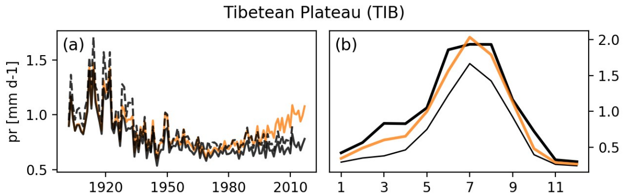
455 Figure 10. Same as Fig. 7 but for precipitation over the Tibetan Plateau (TIB).
