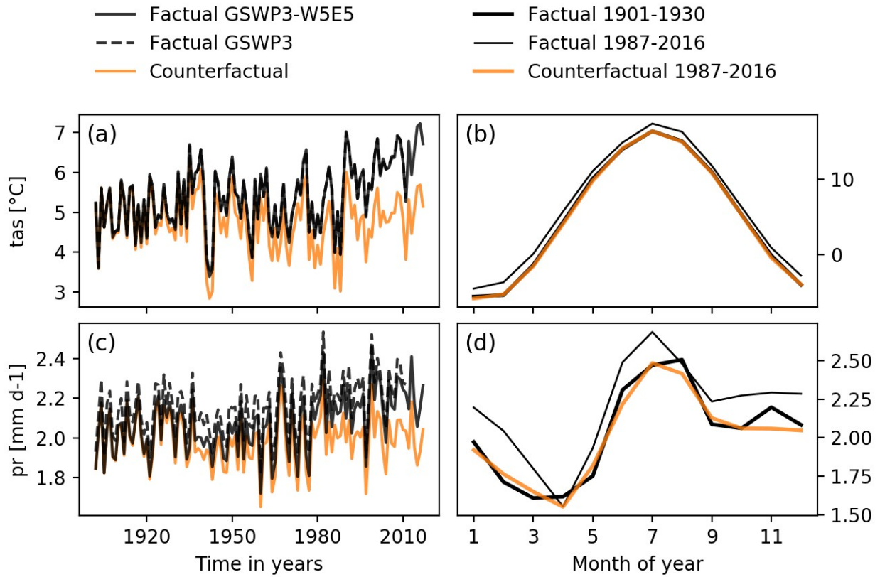
Figure 7. Panels (a) and (c) show annual regional mean time series of factual GSWP3-W5E5 data (solid black line), factual GSWP3 data (dashed black line) and counterfactual GSWP3-W5E5 data (orange line) for near-surface air temperature (a) and precipitation (c) over Northern Europe (NEU). Panels (b) and (d) show multi-year regional mean climatologies for near-surface air temperature (b) and precipitation (d) of factual and counterfactual GSWP3-W5E5 data for NEU. To obtain the counterfactual annual cycle (orange line), our method aims to map the late factual (thin black line) to the early factual (thick black line) annual cycle.
