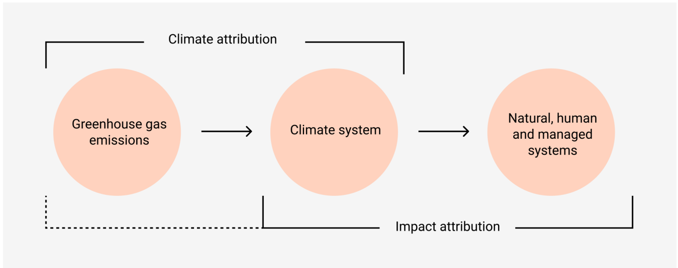
55 Figure 1. Differences between drivers and affected systems in attribution research. Climate attribution is a focus of IPCC WGI (IPCC 2013) and (climate) impact attribution is a focus of IPCC WGII (IPCC 2014, chap. 18). The methodology and data presented here facilitates the use of (process-based) impact models to attribute observed changes in human, managed and natural systems to climate change (lower thick line). The additional step of attribution to emissions (hatched line) is not addressed here.
