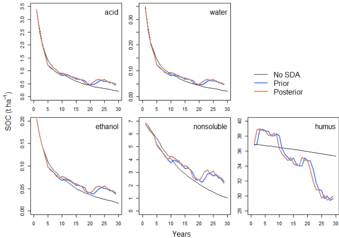
595 Figure 4: The mean of prior and posterior distribution SOC pools at Askov B4 before and after each assimilated observation. Different SOC pools showed different responses to SDA where humus pool was adjusted the most in response to the observations and always to their direction. AWEN pool dynamics responded SDA later over the course of assimilation.
