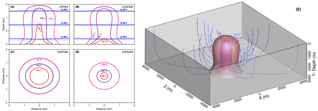
Figure 8. Snapshots of three-dimensional model results. Contour lines for fluid pressure (blue) and temperature calculated from Hydrothermal-Foam are plotted as solid lines, and that from HYDROTHERM are plotted as black dotted lines. (A) and (B) show pressure and temperature contours on vertical slices, (C) and (D) show temperature contours on horizontal slices. (E) show three-dimensional isothermal surfaces and stream lines.
