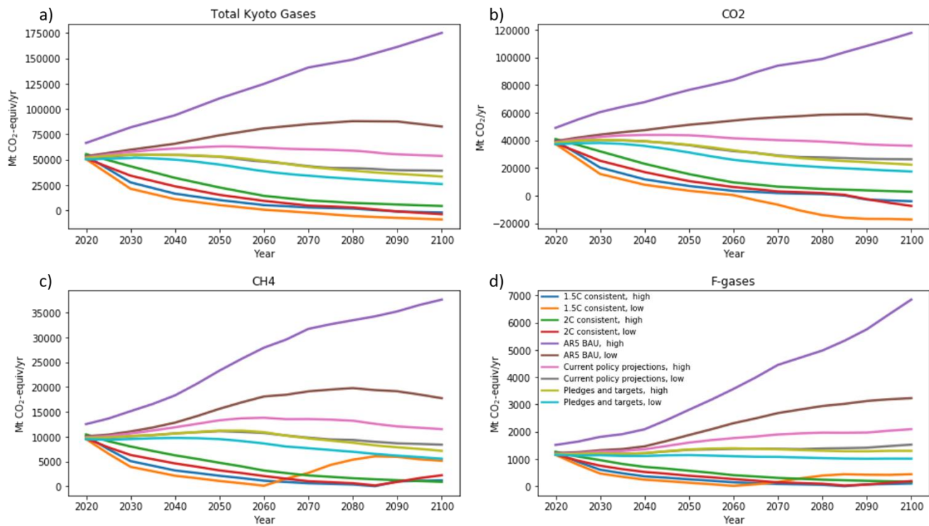
560 Figure 6: Kyoto gases, decomposed by first infilling the non-negative emissions using the (non-ratio) quantile rolling windows, then infilling the CO 2 using infill composite values.
