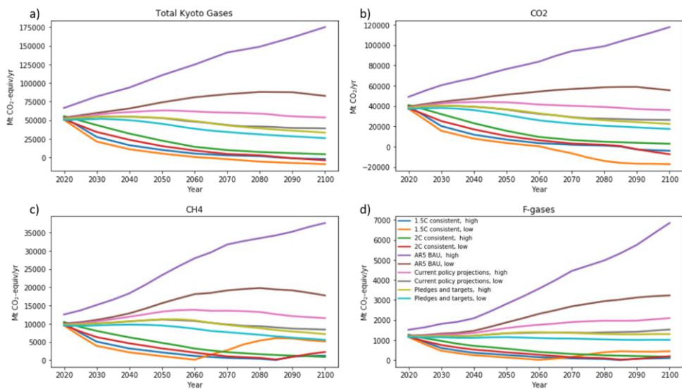
565 Figure 6: Kyoto gases, decomposed by first infilling the non-negative emissions using the (non-ratio) quantile rolling windows, then infilling the CO 2 using infill composite values.
