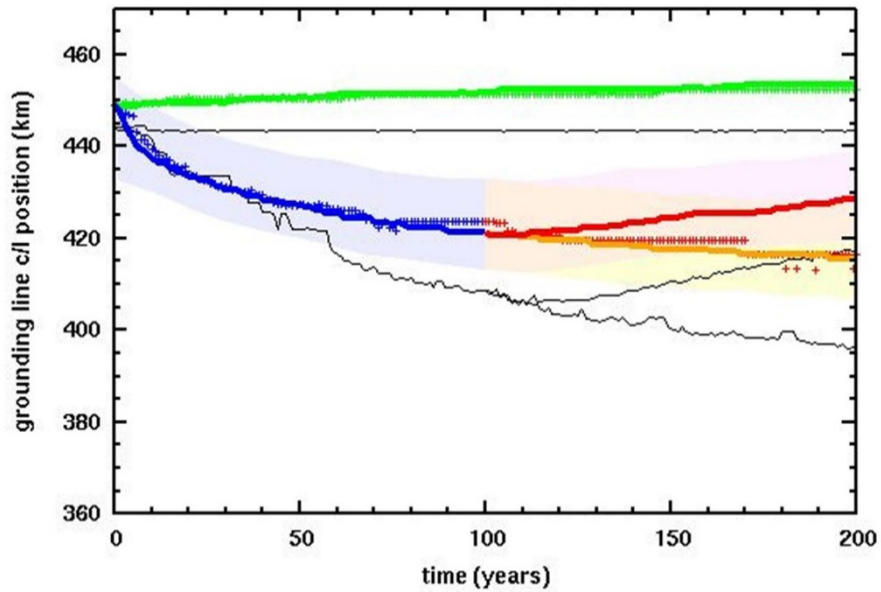
245 Figure 6. As Fig. 3 except for the MISIMIP+ Ice2 experiments. Shading for the "main subset" of MISIMIP+ models is copied from Cornford et al. (2020, their Fig. 13b).
