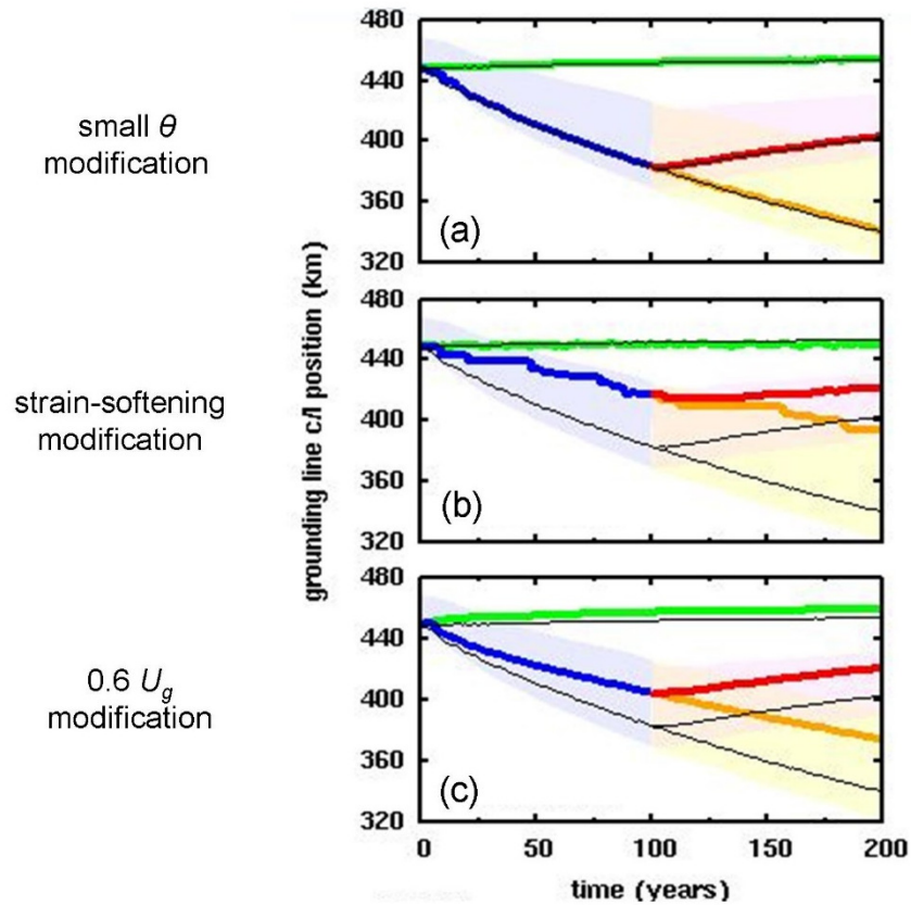
Figure B1. Along-fjord centerline position (km) of grounding lines in the MISIMIP+ Ice1 experiment (Cornford et al., 2020). (a) with small- \theta modification described in section B1. (b) with strain-softening modification described in section B2. (c) with 0.6 U_g modification described in section B3. Thick colored lines: as in main paper except with one of the above modifications. Thin black lines: as in main paper with no further modification. Green: control (continuation of spin-up with zero oceanic melt). Blue and yellow: with oceanic melt perturbation. Red: with oceanic melt reset zero after year 100. Shaded regions show the envelopes for the "main subset" of MISIMIP+ models, copied from Cornford et al. (2020, their Fig. 7a).
