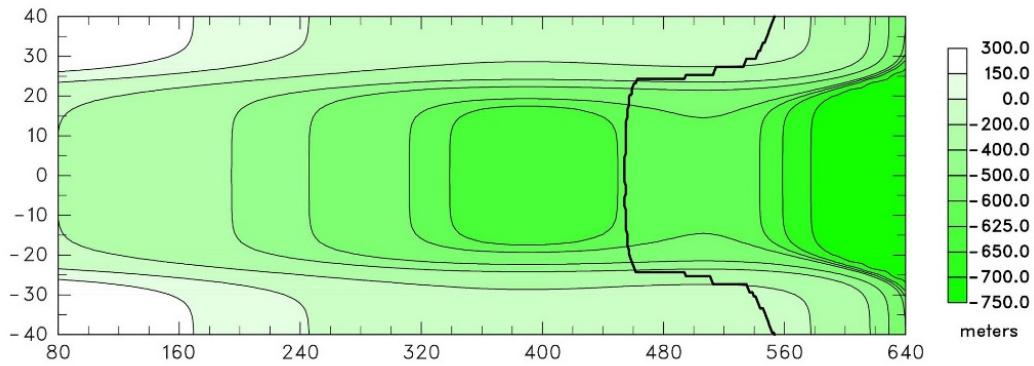
200 Figure 2. Bedrock topography used in the MISMIP+ experiments (Cornford et al, 2020). Also shown is the "control" grounding line after spin-up at year 0 (thick black line). Axes scales are in km. The first 80 km of the channel is not shown. Note the nearly 3x stretching of the channel width relative to the length.
