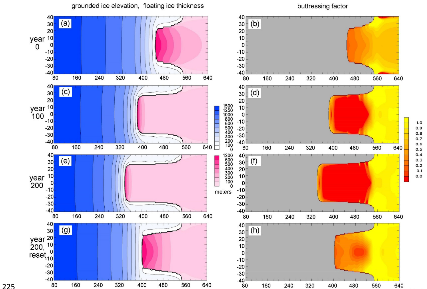
225 Figure 4. Spatial maps in the MISMIP+ Ice1 experiments, for the new model version (as in Fig. 3 with A = 3 \times 10^{-17} \text{ Pa}^{-3} \text{ a}^{-1} ). Flow is left to right. The grounding line is shown by a thick black line. The axes scales (km), truncation of first 80 km, and stretched width are as in Fig. 2. 1st row (a-b): at year 0 (control). 2nd row (c-d): at year 100 with oceanic melt perturbation. 3rd row (e-f): at year 200 with oceanic melt perturbation. 4th row (g-h): at year 200 with oceanic melt reset to zero after year 100. 1st column (a,c,e,g): Grounded ice surface elevations (m, blue scale), and floating ice thicknesses (m, pink scale). 2nd column (b,d,f,h): Buttressing factor \theta (diagnostic except at grounding line).
