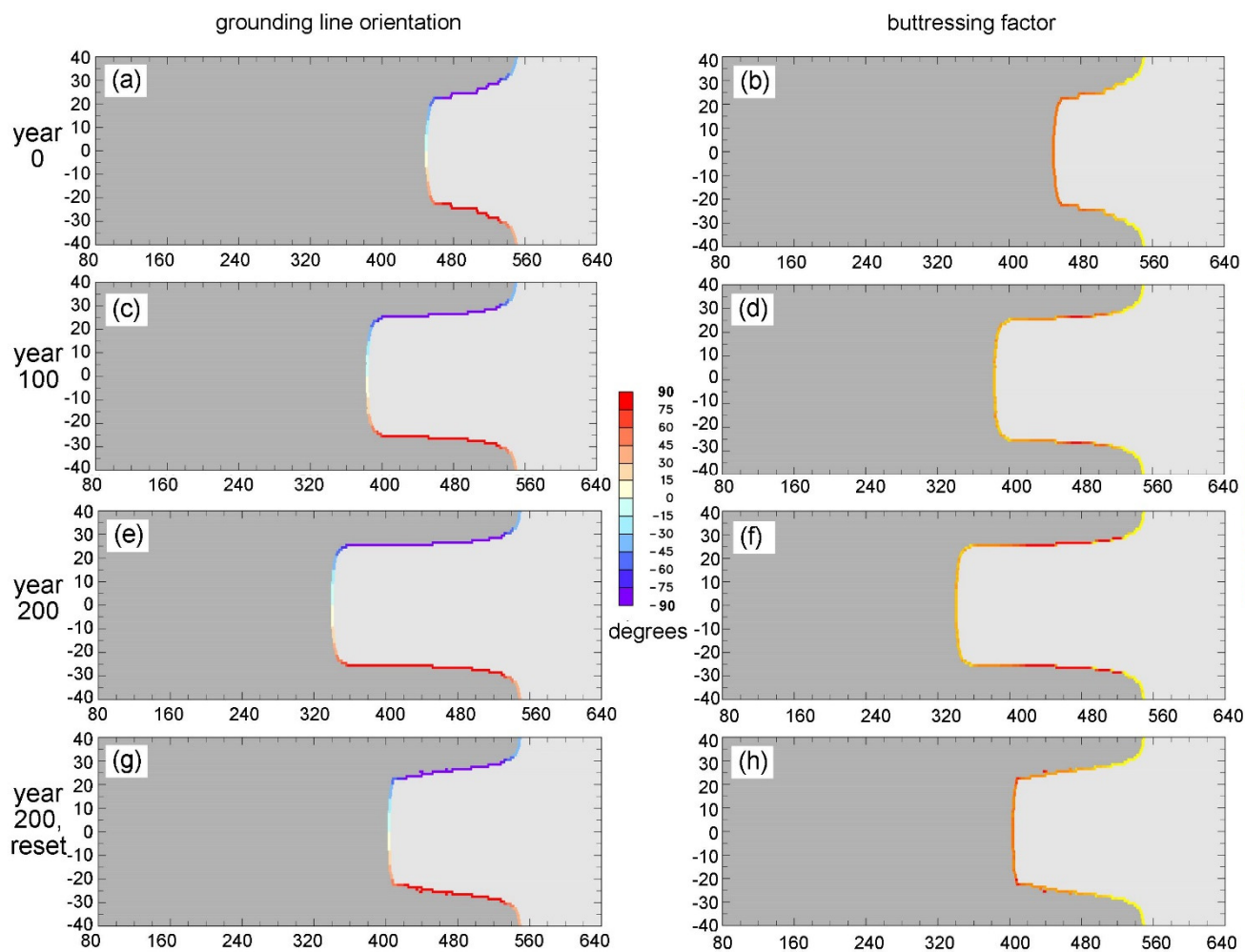
Figure 5. As Fig. 4 for quantities at grounding lines. 1st column (a,c,e,g): Orientation of grounding line (degrees counterclockwise of normal vector (n_x, n_y) from the along-fjord x axis, given by algorithm in section 2). 2nd column (b,d,f,h): Buttressing factor \theta .
