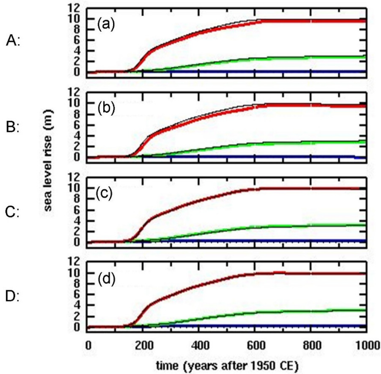
465 Figure A2. Equivalent global sea level rise in simulations of future West Antarctic ice retreat with climate forcing based on RCP8.5 greenhouse-gas scenario. (a) to (d): with the four alternate \theta methods A to D described in the text. Thick colored lines: as in the main paper except with one of the alternate \theta methods. Thin black lines: as in the main paper with the new \theta method described in section 2. Blue: control (perpetual modern climate). Green: with RCP8.5 forcing, without hydrofracturing or cliff failure. Red: with RCP8.5 forcing, with hydrofracturing and cliff failure.
