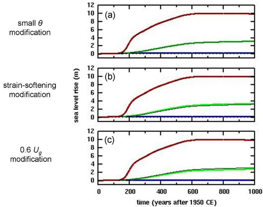
Figure B2. Equivalent global sea level rise in simulations of future West Antarctic ice retreat with climate forcing based on RCP8.5 greenhouse-gas scenario. (a) with small- \theta modification described in section B1. (b) with strain-softening modification described in section B2. (c) with 0.6 U_g modification described in section B3. Thick colored lines: as in main paper except with one of the above modifications. Thin black lines: as in main paper with no further modification. Blue: control (perpetual modern climate). Green: with RCP8.5 forcing, without hydrofracturing or cliff failure. Red: with RCP8.5 forcing, with hydrofracturing and cliff failure.
