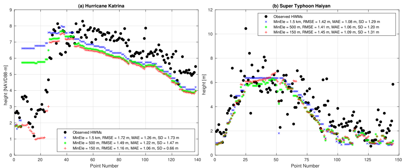
Figure 10. Comparisons of the observed HWMs to the simulated maximum storm tide height at the nearest vertex on meshes with different local MinEle (1.5 km, 500 m, 150 m). (a) Hurricane Katrina (0.23 m has been added to simulated results) and (b) Super Typhoon Haiyan. Points are numbered by starting from the most southwest point and following the shoreline clockwise around.
