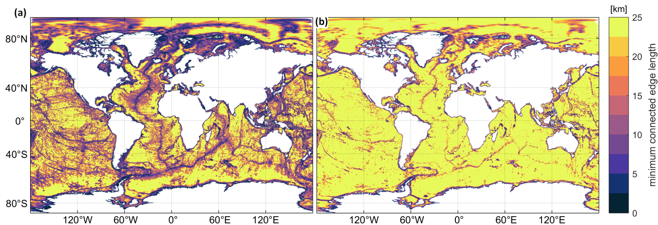
Figure 1. Mesh resolution distribution (defined as the minimum connected element edge length for a mesh vertex) for two global mesh designs. (a) Ref, (b) TLS-B (c.f., Table 2).
