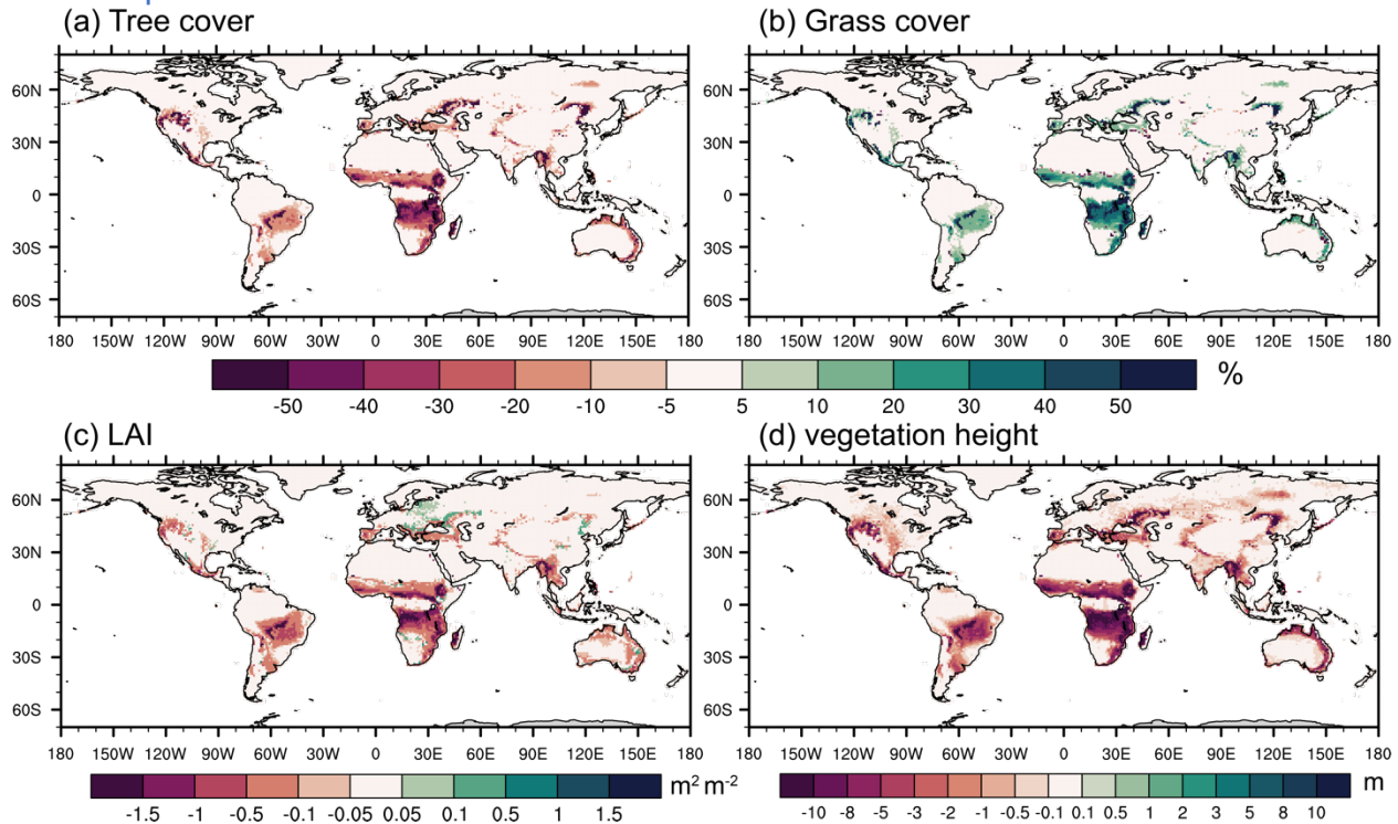
Difference in (a) tree cover (BET, NET, and BDT; %) (b) grass cover (C3 and C4; %), (c) LAI (m 2 m -2 ), and (d) Vegetation height (m) in SSiB4/TRIFFID-Fire averaged over 2000–2014 between FIRE-ON and FIRE-OFF
