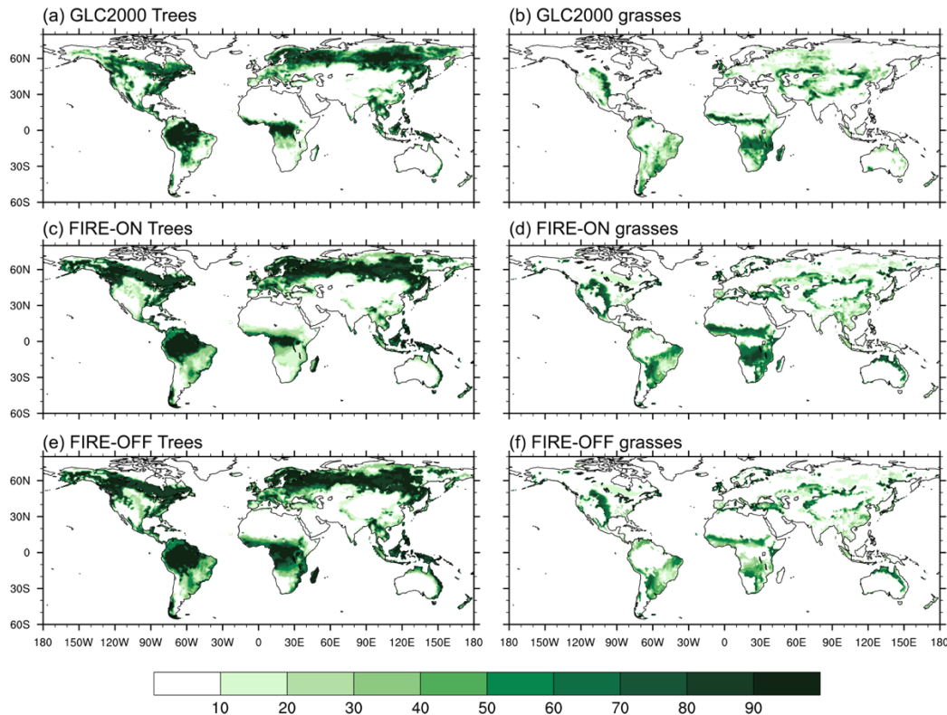
Figure. 10 The spatial distribution of trees in (a) GLC2000 (c) FIRE-ON, and (e) FIRE-OFF and the spatial distribution of grasses in (b) GLC2000 (d) FIRE-ON, and (f) FIRE-OFF in 2000
