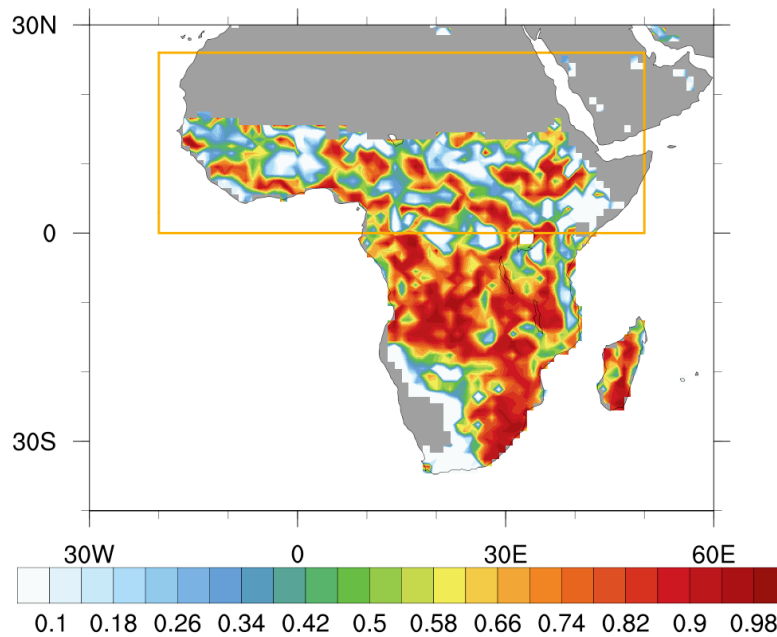
Temporal correlation of monthly burned area in West Africa
