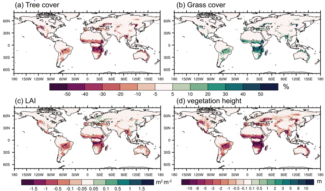
Difference in (a) tree cover (BET, NET, and BDT; %) (b) grass cover (C3 and C4; %), (c) LAI ( \text{m}^2 \text{m}^{-2} ), and (d) Vegetation height (m) in SSiB4/TRIFFID-Fire averaged over 2000–2014 between FIRE-ON and FIRE-OFF
