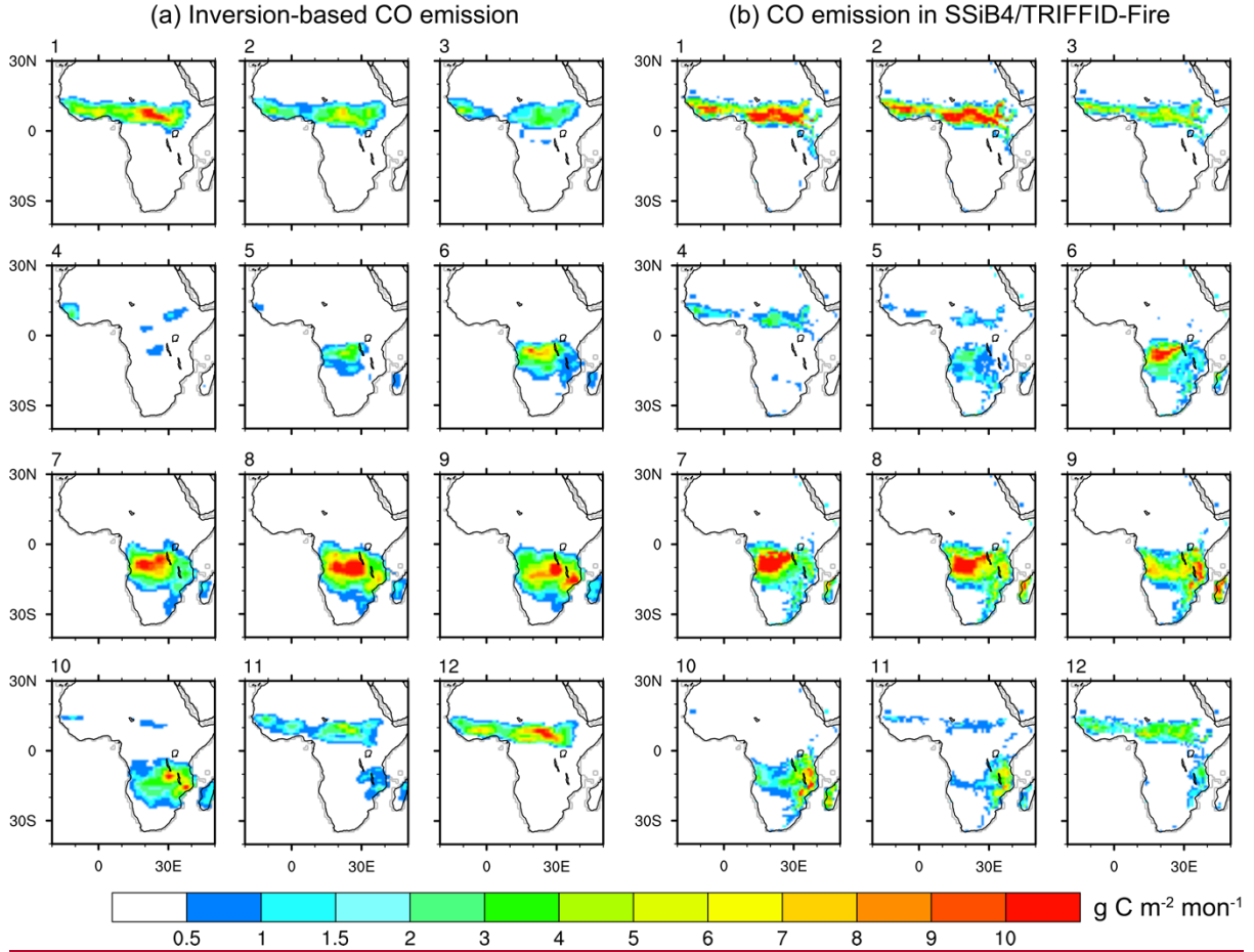
Figure 9. Monthly CO emission in Africa averaged in 2000-2014 from (a) Zheng et al. (2019) and (b) SSiB4/TRIFFID-Fire
