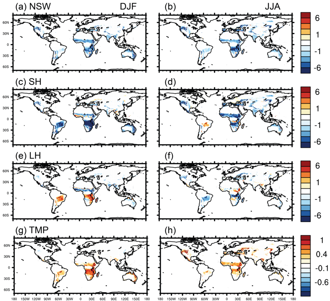
Figure 12. Differences in net shortwave (a, b; W m^{-2} ), sensible heat (c, d; W m^{-2} ), latent heat (e, f; W m^{-2} ), and surface temperature (g, h; K) in DJF (a, c, e, and g), and JJA (b, d, f, and h) averaged over 2000 -2014 between FIRE-ON and FIRE-OFF.
