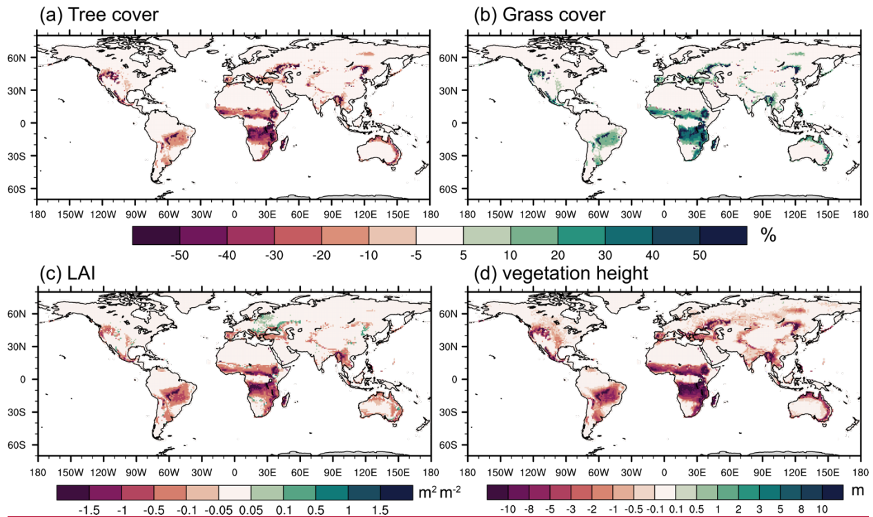
Figure 11. Differences in (a) tree cover (BET, NET, and BDT; %), (b) grass cover (C3 and C4; %), (c) LAI ( \text{m}^2 \text{m}^{-2} ), and (d) Vegetation height (m) in SSiB4/TRIFFID-Fire averaged over 2000 -2014 between FIRE-ON and FIRE-OFF
