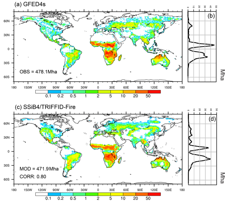
360 Figure 3. Spatial distribution of annual burned fraction (%) averaged over 2000–2014 for (a) GFED4s and (c) SSiB4/TRIFFID-Fire. The right panel shows the zonal mean burned area (Mha) for (b) GFED4s and (d) SSiB4/TRIFFID-Fire
