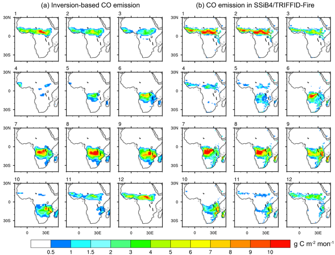
Monthly CO emission in 2000-2014 in Africa from (a) Zheng et al. (2019) and (b) SSiB4/TRIFFID-Fire
