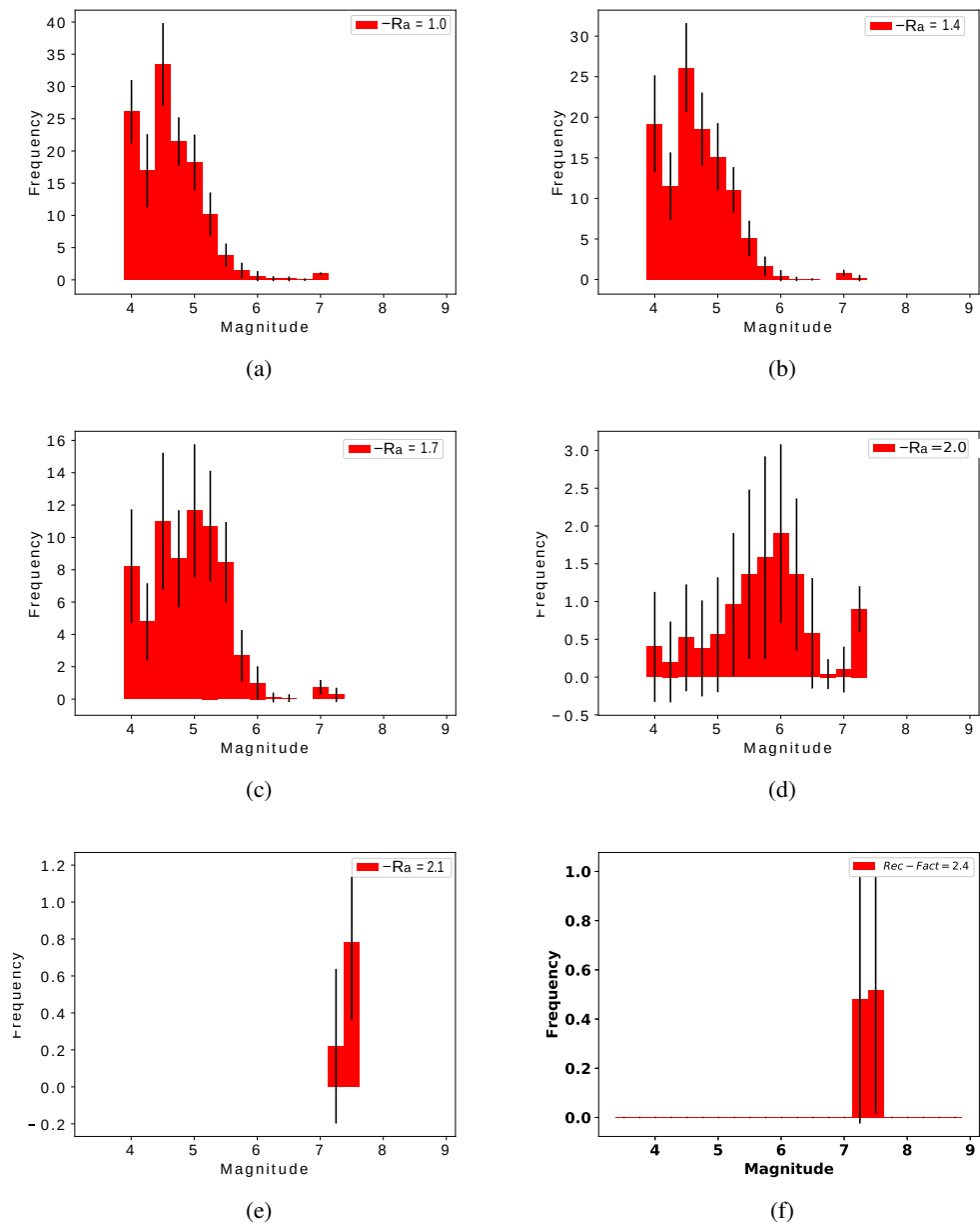
Figure 11. Frequency-magnitude histograms as function of the ratio size R_a and the area domain of 100000 cells. The bars shows the mean histogram, and the error bars depicts the standard deviation of the twenty realizations.
