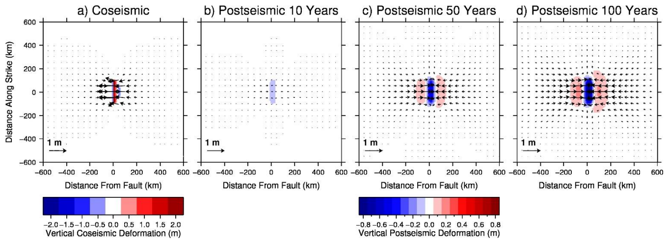
Figure B2: As for Figure B1 but for a 30° dipping reverse fault. Note the different colour scales for coseismic and postseismic displacement.
