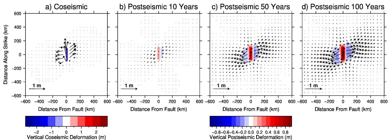
Figure B4: As for Figure B3, a 45° dipping fault, but using the PREM Earth model. Note the different colour scales for coseismic and postseismic displacement.
