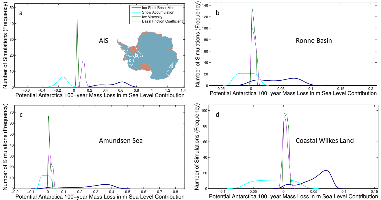
Figure 1. Contribution to uncertainty in 100-year extreme warming simulations of AIS and three subregions of the AIS, tested for four different model variables independently. Each probability distribution function represents an ensemble of 800 Ice-sheet and Sea-level System Model ice dynamics (ISSM-ICE) runs, sampled using the ISSM-DAKOTA uncertainty quantification framework. (Schlegel et al., 2018)
