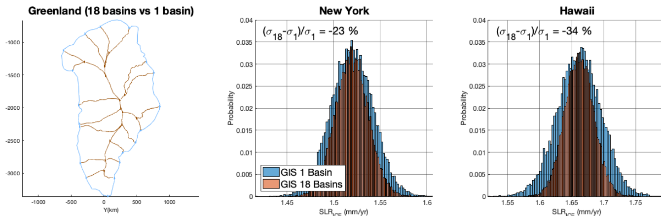
Figure 11. Impact of sub-sampling the GIS mass (from 1 basin for the whole ice sheet to 18 basins) on barystatic sea-level rise in New York and Hawaii. The distributions are a result of SLPS, where H_{GIS} , H_{AIS} and H_{GLA} were sampled 10,000 times using an LHS algorithm. The mean in PDF distributions for both scenarios are identical, however the tails are much larger for the 1 basin scenario. The relative difference in standard deviations between 1 and 18 basins ranges from -23% for New York to -34% for Hawaii. This implies that current probabilistic RSL projections could significantly overestimate (20-30%) the "likely" (5-95%) range in ice-melt contribution from glaciers and ice sheets.
