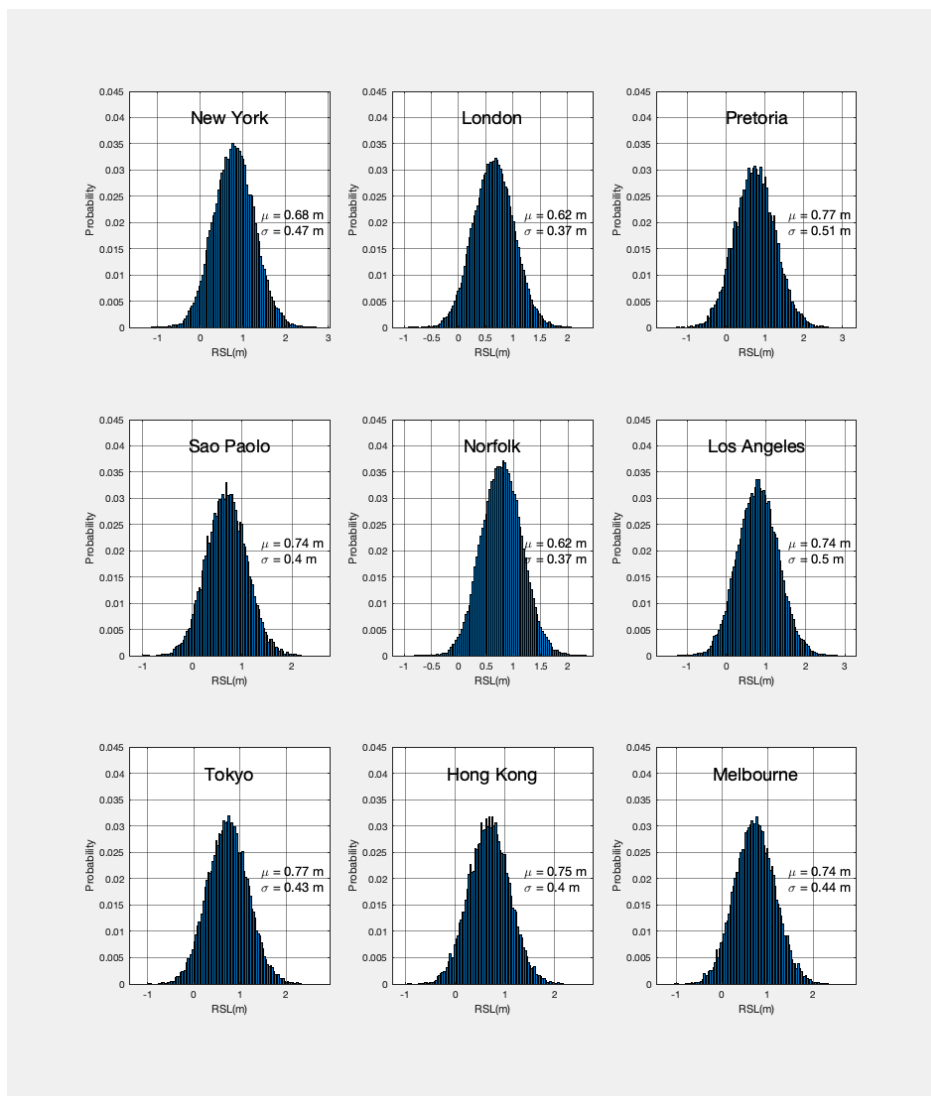
Figure 9. AR5 calibrated projection of RSL for nine cities around the world. Sampling was carried out for H_{AIS} , H_{GIS} , H_{GLA} , STR and H_{TWS} using mean and standard deviations from AR5 (Church et al., 2013a). The patterns for ice thickness are from GRACE 2003-2016 trends (Adhikari and Ivins, 2016). DSL is fully deterministic, from the CMIP5 NorESM runs (Bentsen et al., 2013). RSL_{GIA} was deterministically set to 0. Each time step was sampled for using 10,000 LHS samples.
