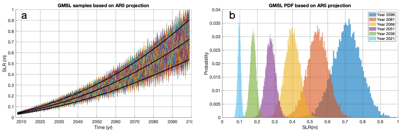
Figure 8. ISSM-SLPS projections based on AR5 RCP8.5. For each time step, we sample (10,000 times with Latin Hypercube Sampling, or LHS) the following inputs: H_{GIS} , H_{AIS} , thermal expansion of the ocean ( STR ), H_{TWS} , and glacier contributions H_{GLA} (see AR5 WG1 Chapter 13, Church et al. (2013b)). Each input's PDF is calibrated using the AR5 5-95% projection confidence interval, similar to Kopp et al. (2014). The resulting GMSL PDF distribution is shown in a) (in time) and b) (at a sub-set of time steps). The 5-95% confidence interval (likely range, following AR5 definition) is plotted in black in a), along with the temporal mean. Each time step is fully decorrelated from the previous time steps, this test being used to validate against existing an existing AR5 projection
