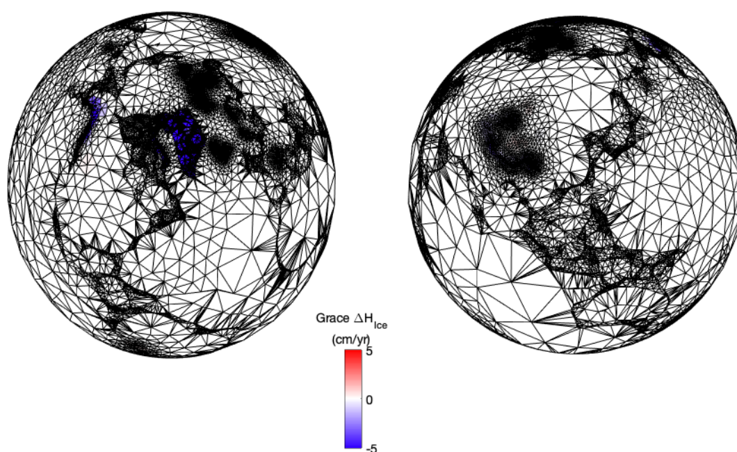
Figure 5. 3D Earth mesh stitched from 3D projections of 2D regional meshes of the following regions: South and North America, Australia, Eurasia, the Pacific regions as well as Antarctica and Greenland. GRACE observations of ice mass change (in cm/yr) from 2003 to 2016 (Adhikari and Ivins, 2016) are overlaid over the mesh. Left frame azimuth is 30° with elevation of 64°. Right frame azimuth is 205° with elevation of 23°.
