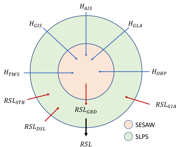
Figure 2. Diagram ISSM’s Sea-Level Projection System (ISSM-SLPS) model. The system is driven by requirements from Eq. 2. ISSM-SESAW is the GRD core of the system ( in pink). ISSM-SLPS is a combination of ISSM-SESAW and a layer (in green) that handles STR, DSL and GIA inputs, as well as all uncertainty quantification aspects.
