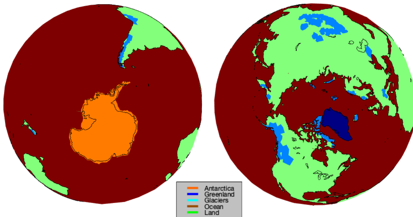
Figure 6. Partition vector (values from 1 to 5, 1 for Antarctica, 2 for Greenland, 3 for Glaciers around the world, 4 for the ocean and 5 for land excepted glaciers). The partition vector is used to sample probabilistic variables in a geographically consistent way, with PDF distributions moments (mean and standard deviation) defined for each partition area.
