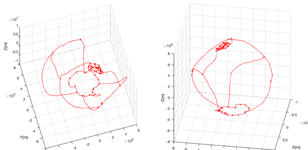
Figure 3. 3D plot of the boundaries used to mesh each continental area of the Earth surface. Regions include South and North America, Australia, Eurasia and the Pacific regions, as well as Greenland and Antarctica. In this particular scenario, Greenland has been sub-divided into 18 regions along the boundaries defined in Zwally et al. (2012).
