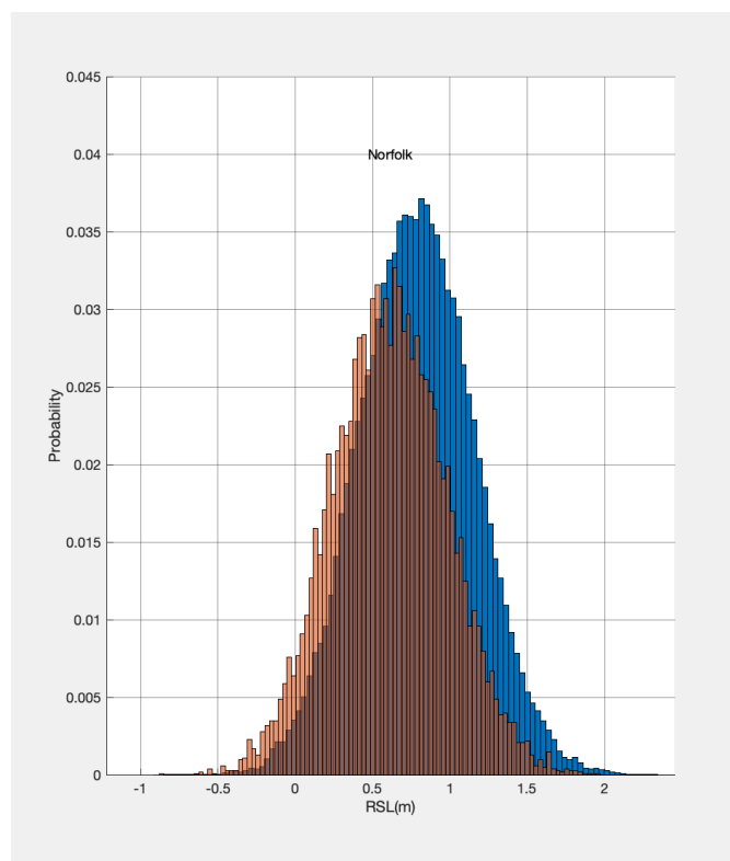
Figure 10. AR5 calibrated projection of RSL for Norfolk (in brown) vs same projection in which GIA statistics from Caron et al. (2018) are used to account for GIA induced RSL (in blue)
