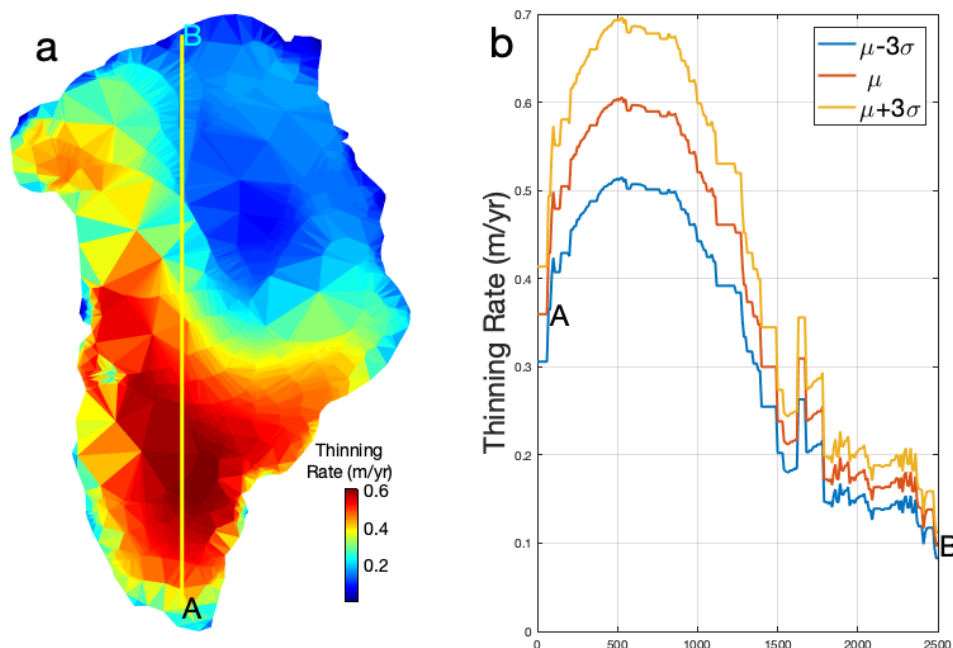
Figure 7. Random sampling of thinning rates across Greenland. a) GRACE generated thinning rate pattern at 2005 (in m/yr). b) Thinning rate along the AB profile (from a) (in red, representing the average of the PDF), and samples generated at -3\sigma (blue) and +3\sigma (yellow) from the average.
