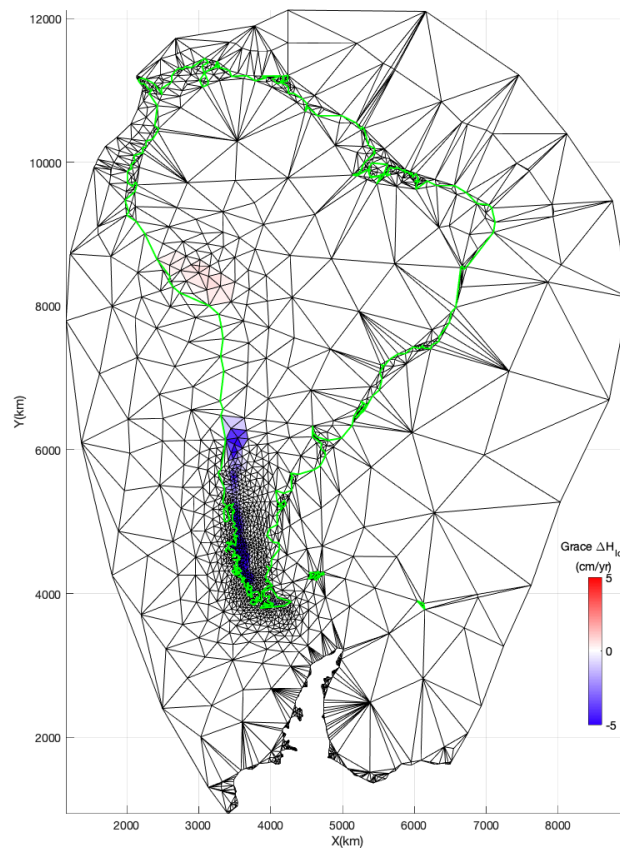
Figure 4. 2D Adaptive mesh of South-America using GRACE observations of ice mass change (in cm/yr) from 2003 to 2016. Seismic effects (Richter et al., 2019) are not removed in this rendering of Patagonian ice mass loss that was directly taken from Adhikari and Ivins (2016). The Global Self-consistent, Hierarchical, High-resolution Geography Database (GSHHG) coarse L1 coastline is shown in green. Segments of the triangular mesh are plotted in black.
