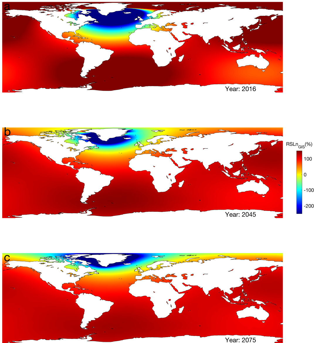
Figure 1. Normalized fingerprints for Greenland at 2016, 2045 and 2075, based on the JPL ISSM experiment 5 simulation contributed to ISMIP6 (Goelzer et al., 2020). [.1] The relative sea level change patterns [.2] in [.3] the [.4] North Atlantic and [.5] Arctic Oceans vary significantly in both space and [.6] time, resulting in [.7] very different contributions to local RSL [.8] in the years 2016, 2045 and 2075.
